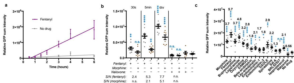
Figure 5. Characterization of M-SPOTIT1.1. (a) Characterization of the maturation time dependence of M-SPOTIT1.1. Similar to Figure 1C, 10 \mu M of fentanyl was used. n=9-10 for each time point. Error bars, standard error of the mean. The mean is represented by each point in the plot. (b) Characterization of M-SPOTIT1.1 agonist exposure time dependence. Similar to Figure 2c, M-SPOTIT1.1 was exposed to fentanyl and morphine for different time periods to characterize the sensitivity of the sensor. The MOR antagonist, naloxone, was added after 30 s stimulation to test its inhibition of sensor maturation. 10 \mu M drug concentration was used for all. Cells were imaged fixed at pH 9 24-hours post-stimulation. S/N was calculated by dividing the sum GFP intensity of the agonist condition and no agonist condition for 30s, 5min, and 6hr + agonist time points. An unpaired Student's t-test was used to determine the significance between the agonist and no agonist conditions and the agonist + naloxone and only naloxone conditions. Stars indicate significance. Four stars is a p -value of 0.0034 and 0.0036 for 30s + Fentanyl and 5min + morphine, respectively. "n.s." indicates no significant difference between compared conditions with p -values of 0.263, 0.1692, and 0.0722 for 30s + morphine and antagonist conditions, respectively. Error bars, standard error of the mean. The mean is represented by the thicker horizontal bar. n=7-10 for each condition. (c) Characterization of M-SPOTIT1.1 drug selectivity. Two days after infection with lentiviruses expressing M-SPOTIT1.1, cells were stimulated with 10 \mu M of each drug for 24-hours, and then fixed and imaged at pH 9. Error bars, standard error of the mean. The mean is represented by the thicker horizontal bar. Values above the dots represent the fold-change of GFP signal compared to no drug condition. Stars indicate significance after performing an unpaired Student's t-test. Four stars indicate a p -value <0.0001 . Two stars indicate a p -value of 0.0065, 0.0047, and 0.0018 for Leu-enkephalin, DADLE, and naloxone, respectively. One star indicates a p -value of 0.0270, 0.0350, and 0.0132 for endomorphin-1, endomorphin2, and sal A, respectively. "n.s." indicates no significant difference with a p -value of 0.0853. n=8-10 for each condition.
