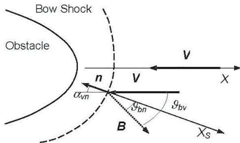
Figure 2. Definitions of the additional bow shock parameters for arbitrary direction of the interplanetary magnetic field.
