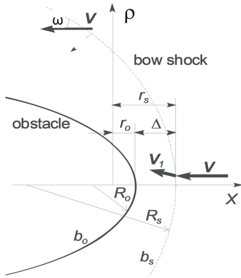
Figure 1. Bow shock parameters used in our model: r_o , r_s are positions of the obstacle boundary and bow shock nose, respectively; R_o , R_s are nose curvature radii; respectively; and \Delta is the bow shock standoff distance; \omega is the slope of the bow shock.
