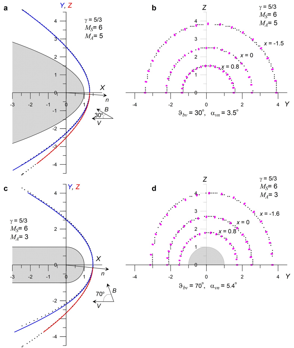
Figure 7. Two examples of fitting the magneto-hydrodynamics bow shock calculations (black points) with relation (1): (a and c) Blue line shows fitting in the (X, Y) plane of the Geocentric InterPlanetary Medium system, red line shows fitting in the (X, Z) plane; (b and d) cross-sections of the bow shock by planes X = \text{const} , hot pink points.
