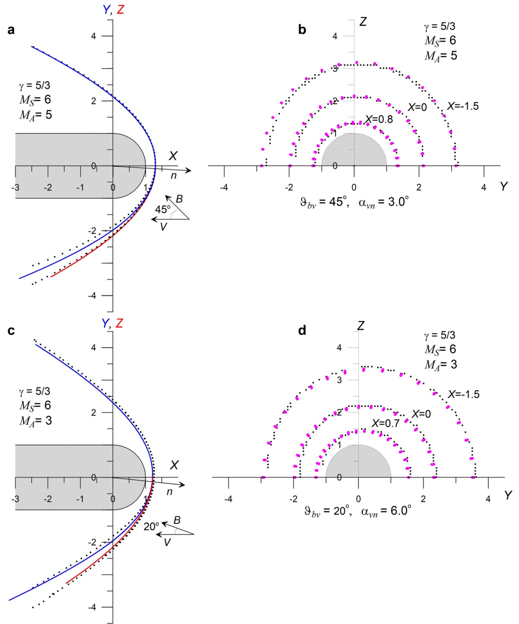
Figure 10. Two examples comparing the magneto-hydrodynamics bow shock calculations (black points) with its location determined by relations (1, 6, 27–30): (a and c) blue line shows expression (1) in the (X, Y) plane of Geocentric InterPlanetary Medium system, red line shows expression (1) in the (X, Z) plane; (b and d) cross-sections of the bow shock by planes X = \text{const} , hot pink points - expression (1).
