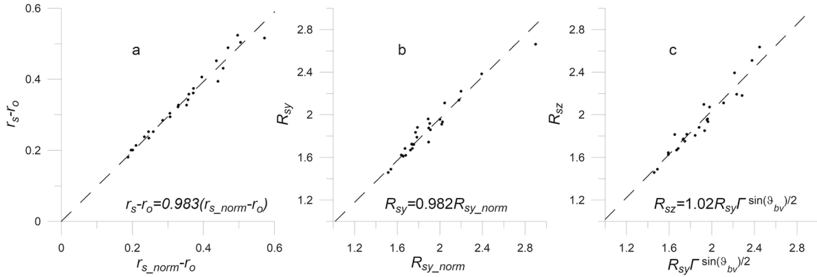
Figure 8. Comparison of the parameters r_s , R_{sy} , and R_{sz} of the bow shock model (1) fitting the magneto-hydrodynamics calculations (Table 1), with the parameters calculated using the gas dynamics model. Dashed lines represent fitting dependencies, printed at the bottom of each panel.
