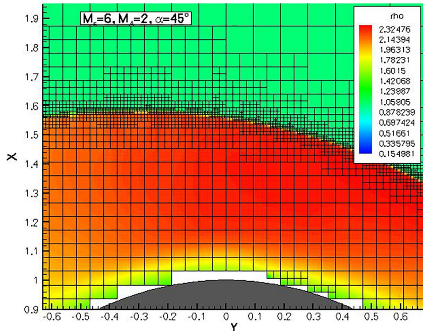
Figure 5. Example of the grid. Cut cells used to fit the central body are not shown.
