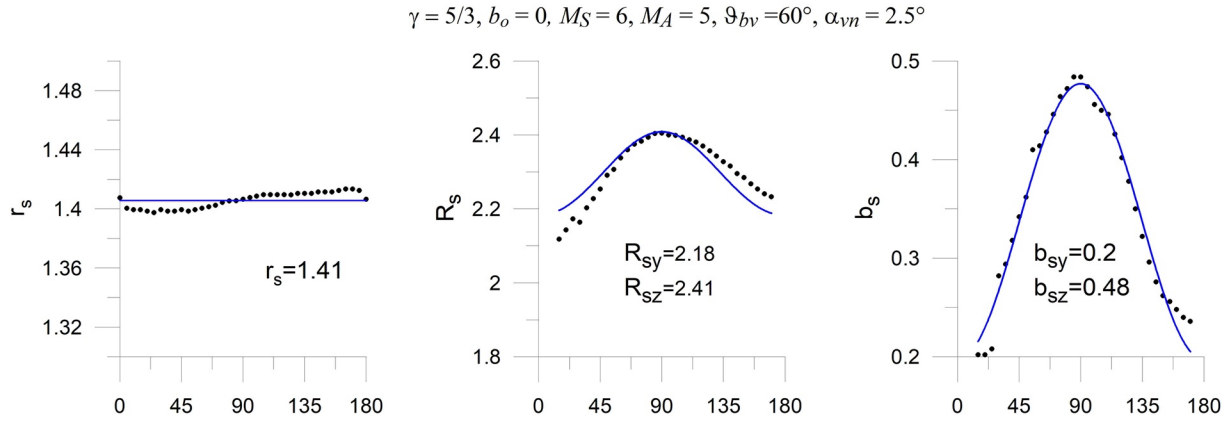
Figure 6. Parameters r_s(\varphi_s) , R_s(\varphi_s) , and b_s(\varphi_s) as functions of the angle \varphi_s . Points are the parameters of approximation of magneto-hydrodynamics simulations in planes \varphi_s = \text{const} with a step along \varphi_s equal to 5^\circ , solid lines—approximation using expressions (21).
