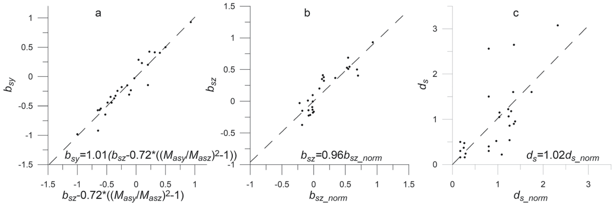
Figure 9. (a) Interrelationship between the parameters b_{sy} and b_{sz} , (b) comparison for the parameter b_{sz} fitting the magneto-hydrodynamics calculations, with the parameter b_{sz\_norm} , calculated using the gas dynamics model, (c) comparison of the fitting parameter d_s with calculated parameter d_{s\_norm} . Dashed black lines show fitting dependencies printed at the bottom of the panels.
