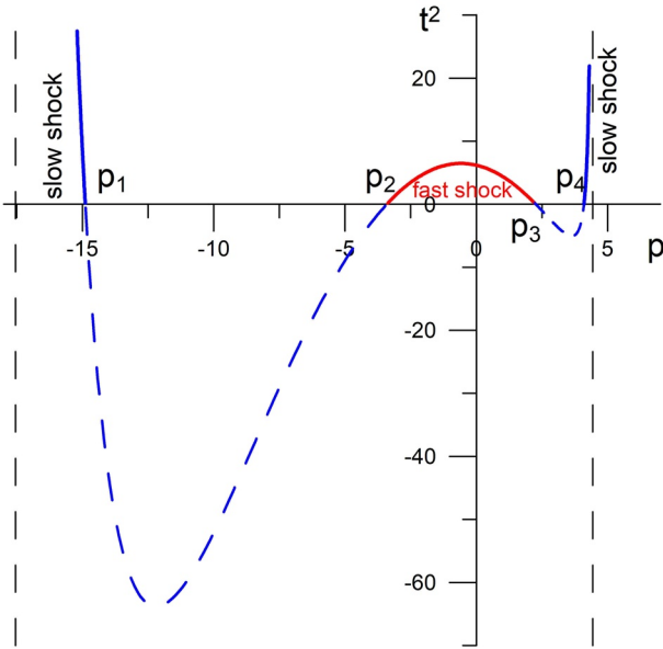
Figure 4. t^2(p) function for M_S = 6 , M_A = 3 , \vartheta_{bv} = 70^\circ , \alpha_{vn} = 4.3^\circ . Sections of t^2(p) shown with solid blue lines are physically meaningful; those shown with blue dashed lines do not correspond to real shocks. The vertical dashed lines represent the asymptotes of this function.
