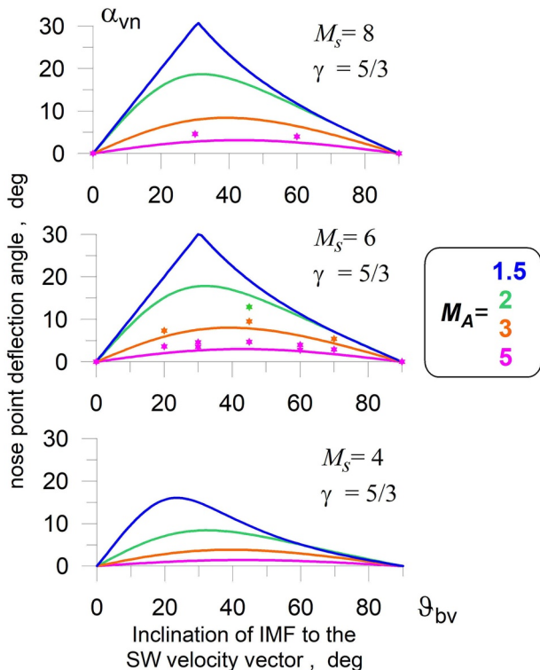
Figure 3. Calculations of \alpha_{vn} for different Mach numbers and angles \vartheta_{bv} . Asterisks mark fitting of skewing angles (see Section 6).
