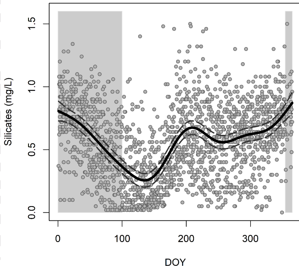
Figure 4: Seasonality of dissolved silicates in samples collected from the Union Water Treatment Plant on Lake Erie vs. day of year (DOY) for the period 1976–2013. The typical ice cover period is shown as a light grey polygon. The solid black line shows a generalized additive mixed effects model fit, with DOY as fixed factor and year as random factor; dashed lines represent the 95% CI ( F_{8,45} = 83.2 , R^2_{adj} = 0.24 , p < 0.0001 ). These data are part of the Ontario Lake Water Quality at Drinking Water Intakes program, which reports biweekly water quality data from 18 drinking water intake treatment plants along the Ontario shore of lakes Superior, Huron, Erie, and Ontario (Ontario Open Data Team, 2020). These data are the most comprehensive record of winter-period water quality in the Great Lakes, but are representative only of nearshore conditions.
