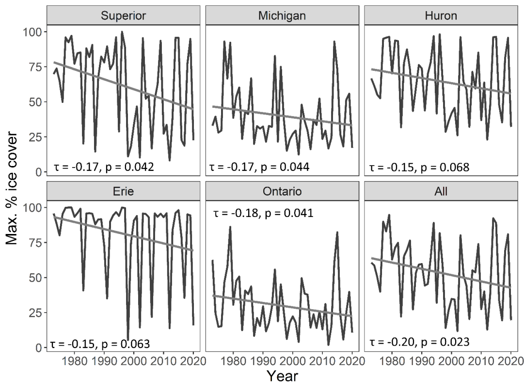
Figure 2: Annual maximum ice cover (AMIC) extent for individual Great Lakes and across all five lakes ('All') for the period between 1973 and 2020, with simple linear regression lines and tau and p-values for one-tailed Mann-Kendall trend tests. AMIC is defined as the maximum value of the daily ice extent over the entire ice season.
