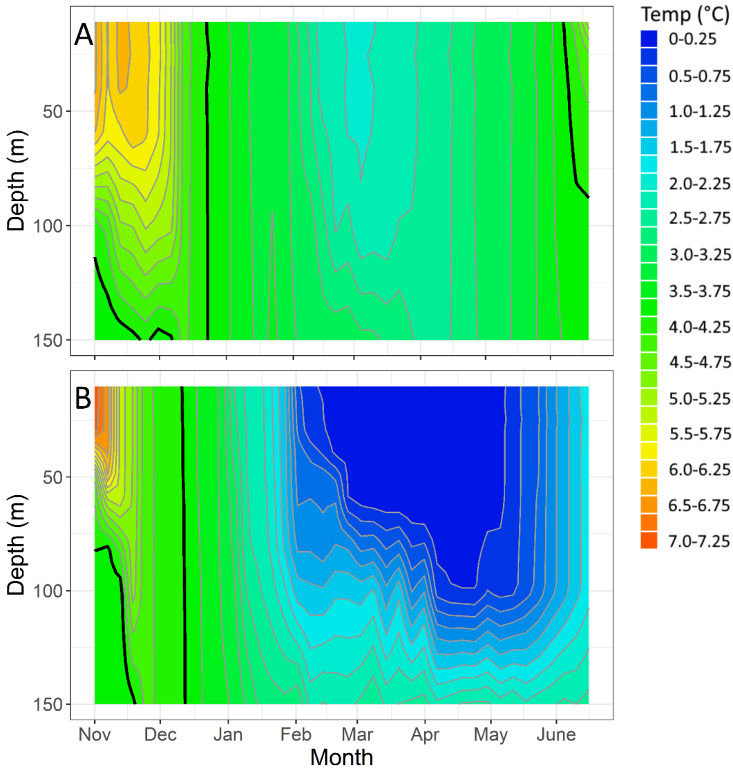
Figure 3: Winter thermal structure in eastern Lake Superior in a warm winter (2009–2010, 27.3% maximum areal ice cover; A) and a cold winter (2013–2014, 95.8% maximum areal ice cover ice cover; B) Black contour represents 4°C (temperature of maximum density).
