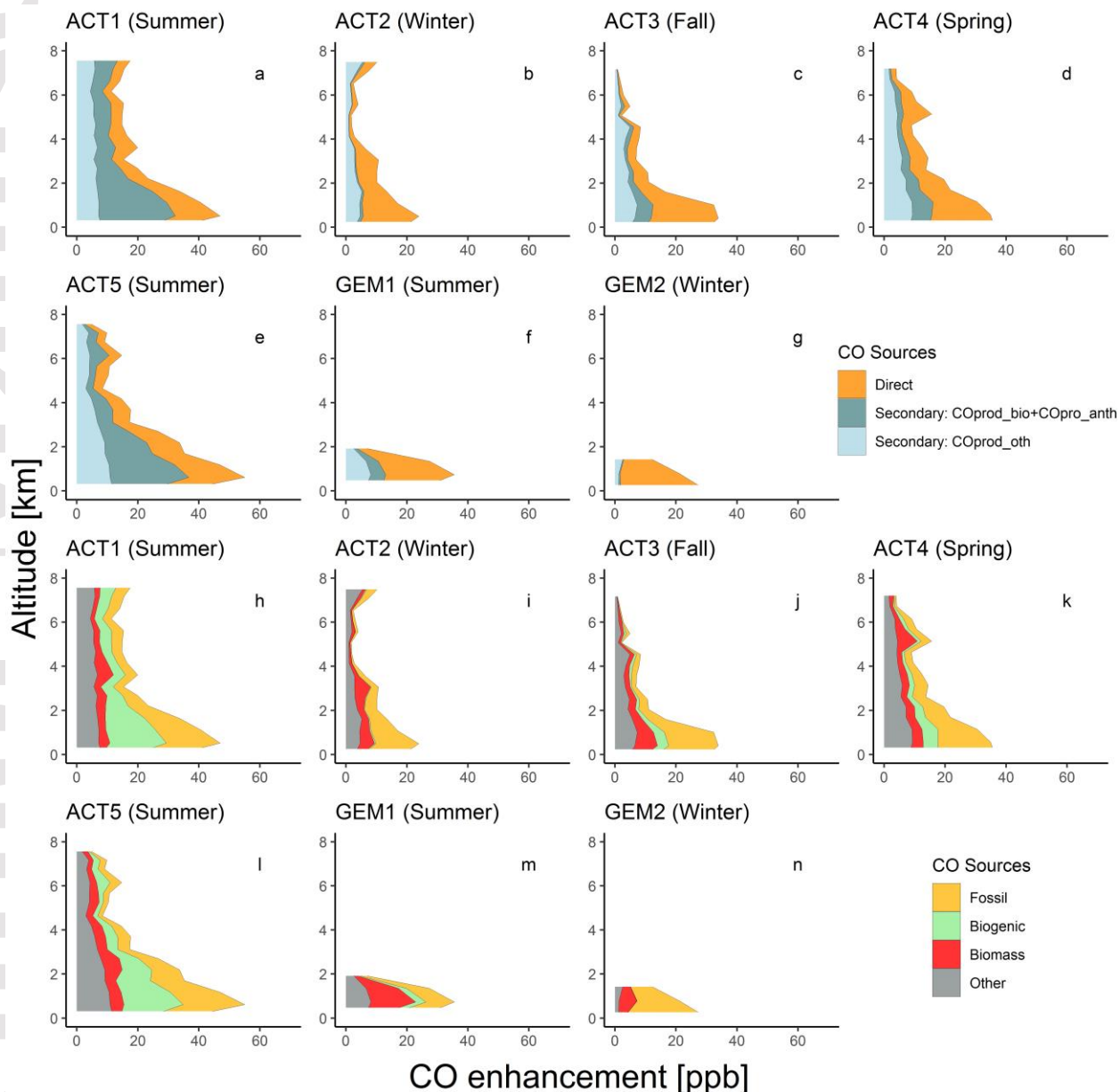
Figure 3: Observationally-constrained CO source attribution over the eastern US. Plotted are the mean above-background CO profiles from the optimized GEOS-Chem simulation along the
