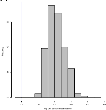
Simulation Results – Log Chi-squared distribution
