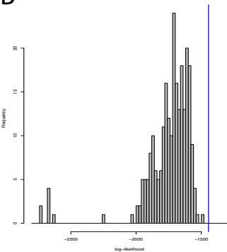
Simulation Results – Log-likelihood distribution
