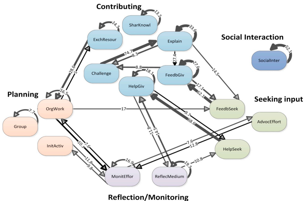
Fig. 4. Behavioral transition diagram for the IECS condition.
