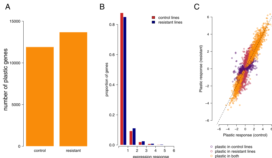
Figure 3. (A) The number of genes showing plastic expression differences in response to herbicide at FDR <0.1 in control and selected lines (B) A histogram of gene expression responses to herbicide, measured as the absolute value of the \log_2 -fold change of expression measured with and without herbicide. C) Plastic expression in control lines and lines selected for resistance. Response is shown on a \log_2 scale and the x = y line is plotted with a dashed black line. Points are colored by whether they show a significant plastic response to spray in resistant and control lines. Genes without a significant response in either set of lines are not shown.
