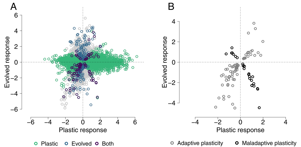
Figure 2. Plastic and evolved changes in expression: (A) The x-axis shows plastic responses to glyphosate, specifically the log fold change in expression between sprayed and nonsprayed conditions where positive values indicate increased expression in herbicide spray. The y-axis shows the log fold difference in expression between lines selected for increased resistance to herbicide and lines that were not selected (“original lines”), where positive values indicate increased expression in the resistance selection lines. Each point represents one gene, colored by whether they have significant (FDR < 0.1) plastic expression responses, evolved expression responses or both. (B) The same as (A), but only genes with significant responses to selection and treatment are shown.
