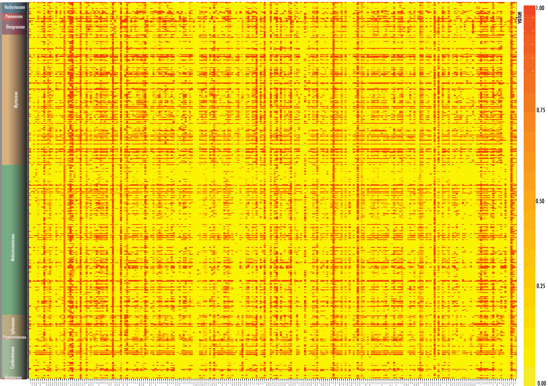
Heatmap for the Recovery of the Plastome. Cell shadings correspond to the length of the gene recovered for each sample relative to the length of the reference.
