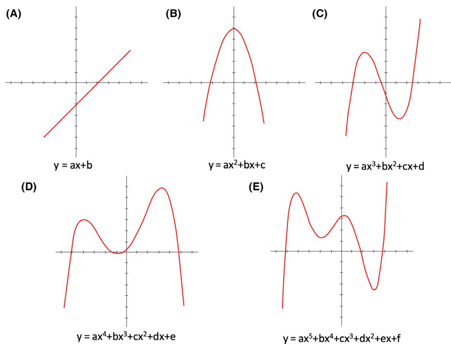
FIGURE 1 In the prediction model, chronologic age was considered as a polynomial up to the fifth order or fifth degree. Graphical representations of polynomials. A, First order or first degree polynomial (linear polynomial or linear function). B, Second order or quadratic term or second degree polynomial is represented graphically by a parabolic curve. C, Third order or cubic term or third-degree polynomial has a single inflection point, (a point where the function changes from being concave to convex or vice versa) and 2 extrema (maximum or minimum). D, Fourth order or quartic term or fourth degree polynomial has 2 inflection points and 3 extrema. E, Fifth order or quintic term or fifth degree polynomial has 3 inflection points and 4 extrema [Colour figure can be viewed at wileyonlinelibrary.com ]
