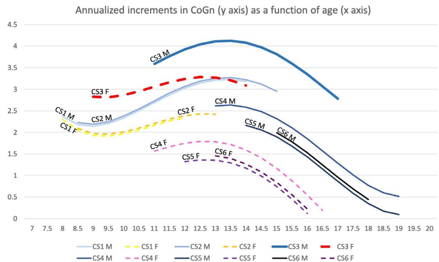
FIGURE 2 Annualized increments of Co-Gn (y axis) as of function of age (x axis), gender and cervical stage [Colour figure can be viewed at wileyonlinelibrary.com ]
