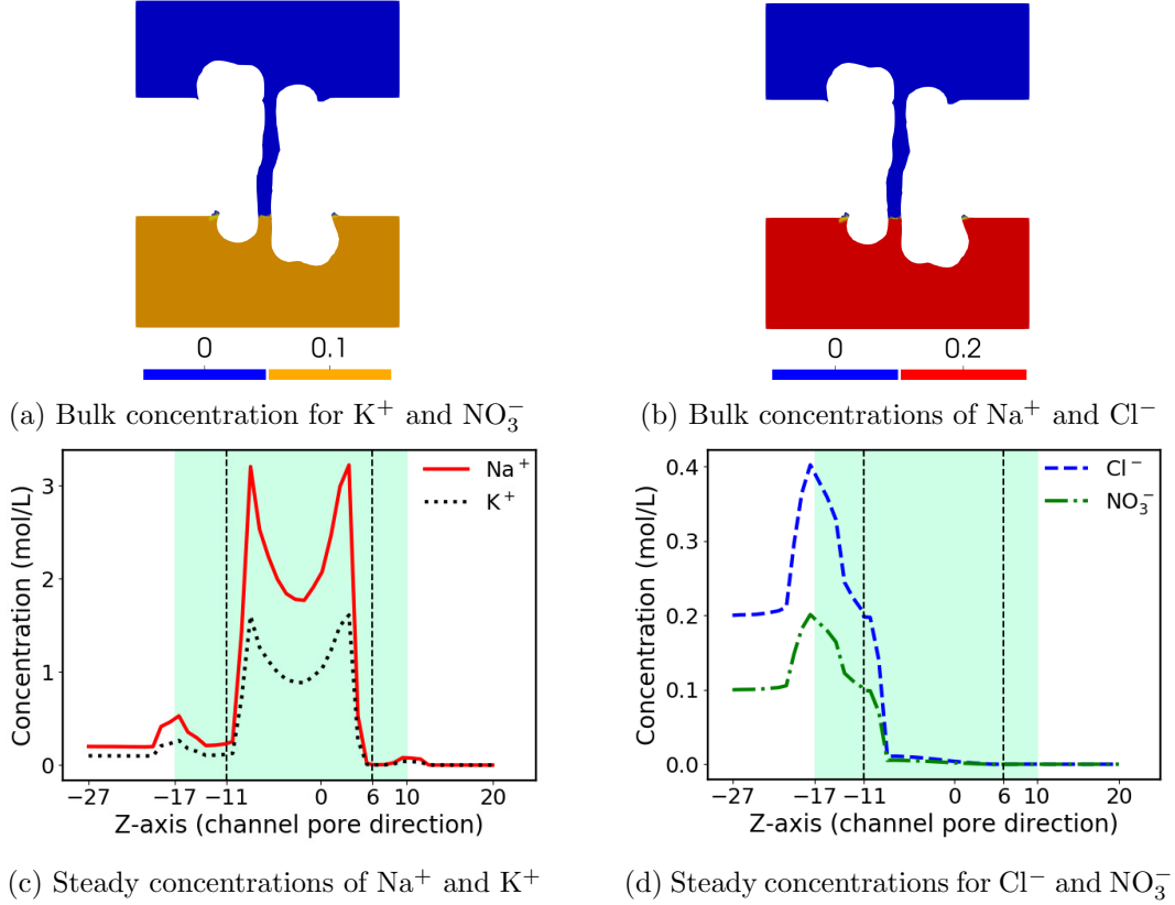
Figure 7: A comparison of the bulk concentrations with the steady concentrations of cations Na^+ and K^+ and anions Cl^- and NO_3^- — the concentrations generated by the PNPic finite element package for gA in Solvent 3. Here g_b = g_t = 0 and \sigma_b = \sigma_t = 0 .
