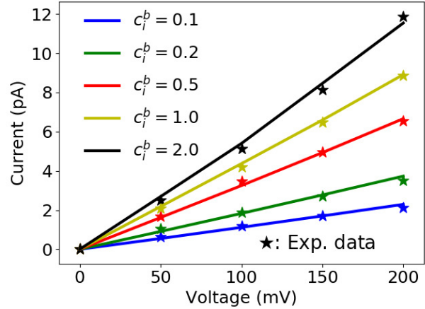
Figure 14: Five I-V curves produced by the current data of Table 4. Here the solid lines stand for our predicted curves and the star markers represent the experimental values from 23 .
