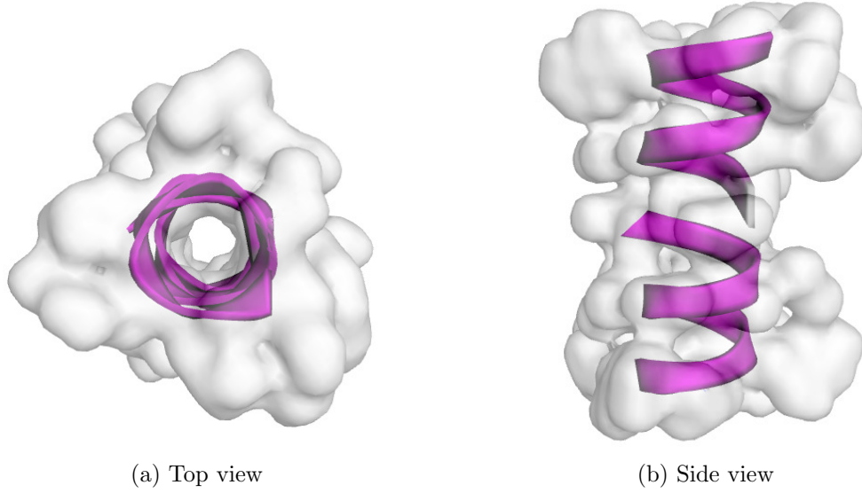
Figure 4: Two views of a gA ion channel molecular structure (in cartoon) and its Van der Waals volume (in grey) occupied by the atomic balls of gA.
