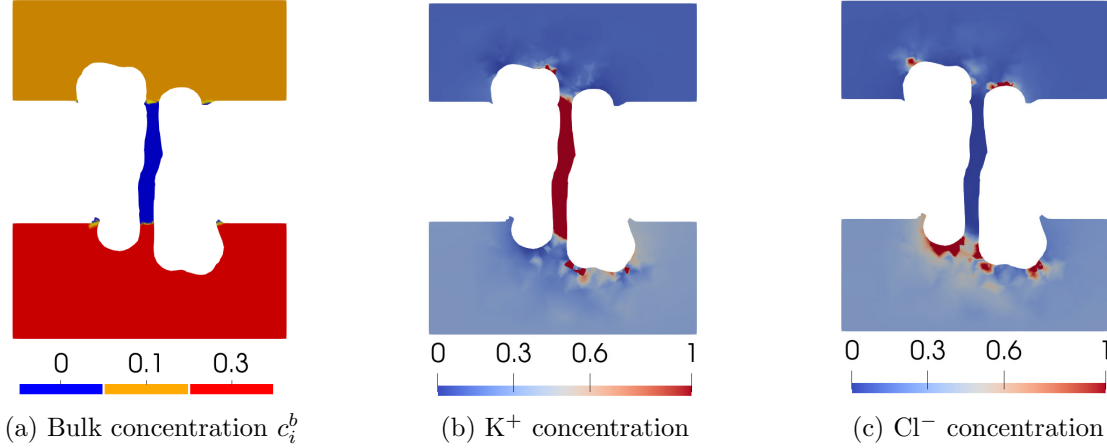
Figure 6: A comparison of the bulk concentrations c_i^b for i = 1, 2 with the concentrations of K^+ and Cl^- generated by the PNPic finite element package for gA in Solvent 2. Here c_i^b is a piecewise constant functions defined in (9), c_{i,b}^b = 0.3 , c_{i,t}^b = 0.1 , c_{i,p}^b = 0 , g_b = 2 , g_t = -2 , and \sigma_b = \sigma_t = 0 .
