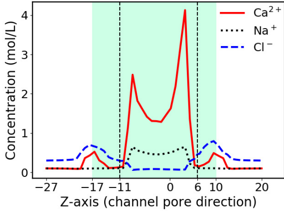
Figure 11: Concentrations for gA in Solvent 4. Figure 12: Concentrations for gA in Solvent 5.
