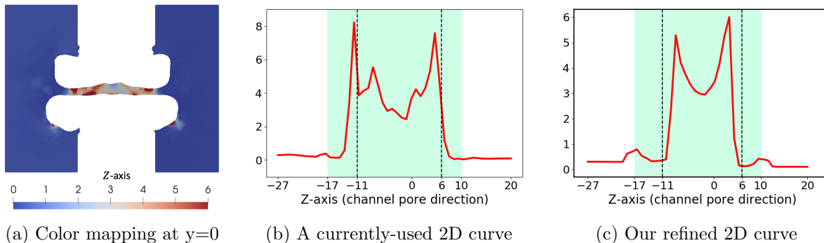
Figure 8: A comparison of our 2D curve with a color mapping and a currently-used 2D curve for a concentration of K^+ reported in Figure 9a. Here the color mapping visualizes the concentration values on a cross section ( y = 0 ) and the currently-used 2D curve is produced by the concentration values on a segment ( -27 \leq z \leq 20 ) of the z -axis.
