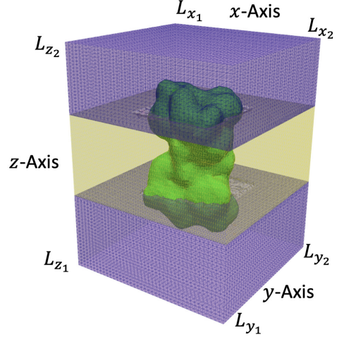
Figure 2: An interface fitted tetrahedral mesh of box domain \Omega . Here D_p , D_m , and D_s are highlighted in green, yellow, and blue-violet.
