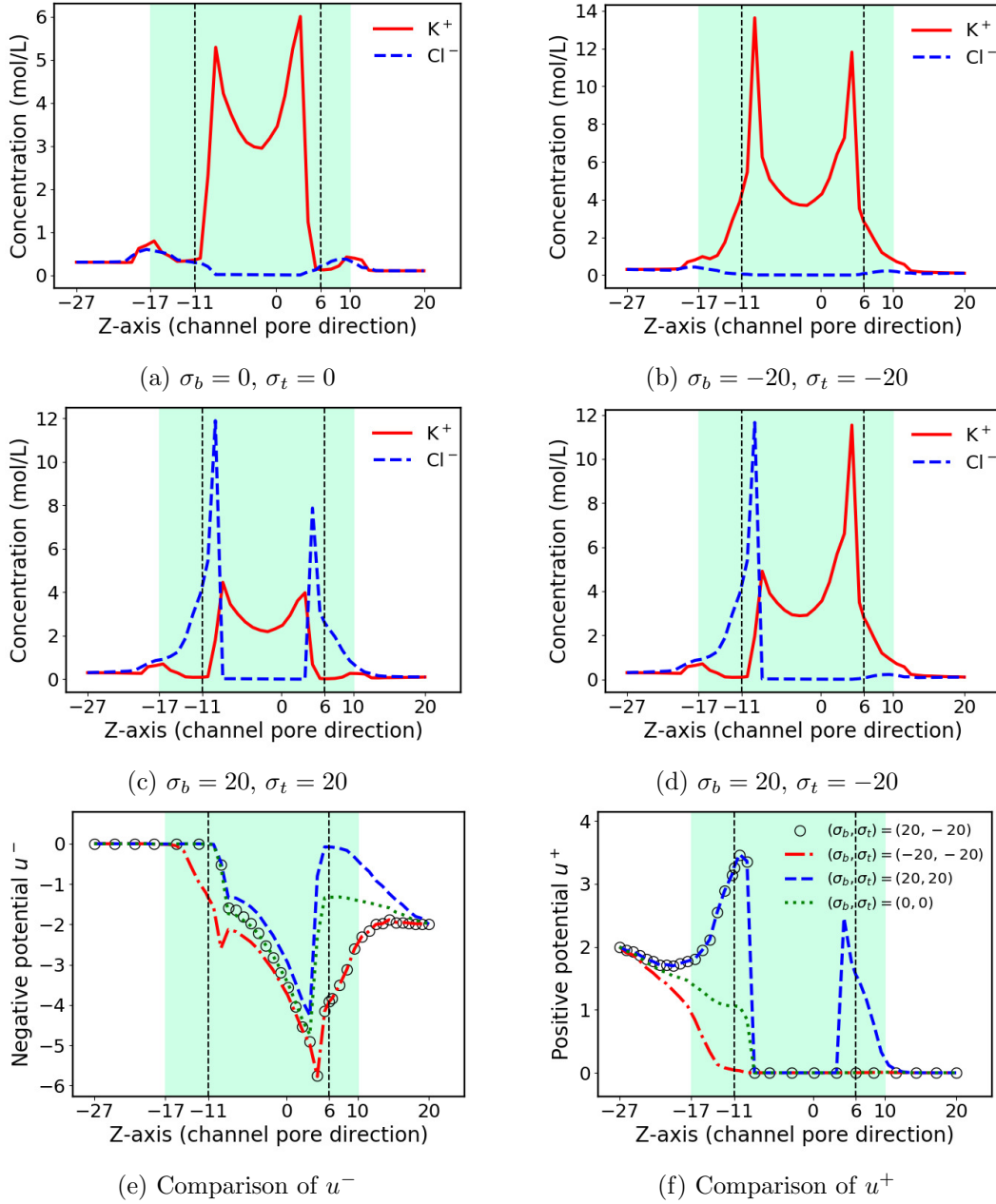
Figure 9: Effects of membrane charges on ionic concentrations (a to d) and electrostatic potentials (e, f) for gA in Solvent 2. Here \sigma_b and \sigma_t are the surface charge densities on the bottom and top surfaces of membrane, respectively; and u^+ and u^- are defined in (22). Here g_b = 2 and g_t = -2 .
