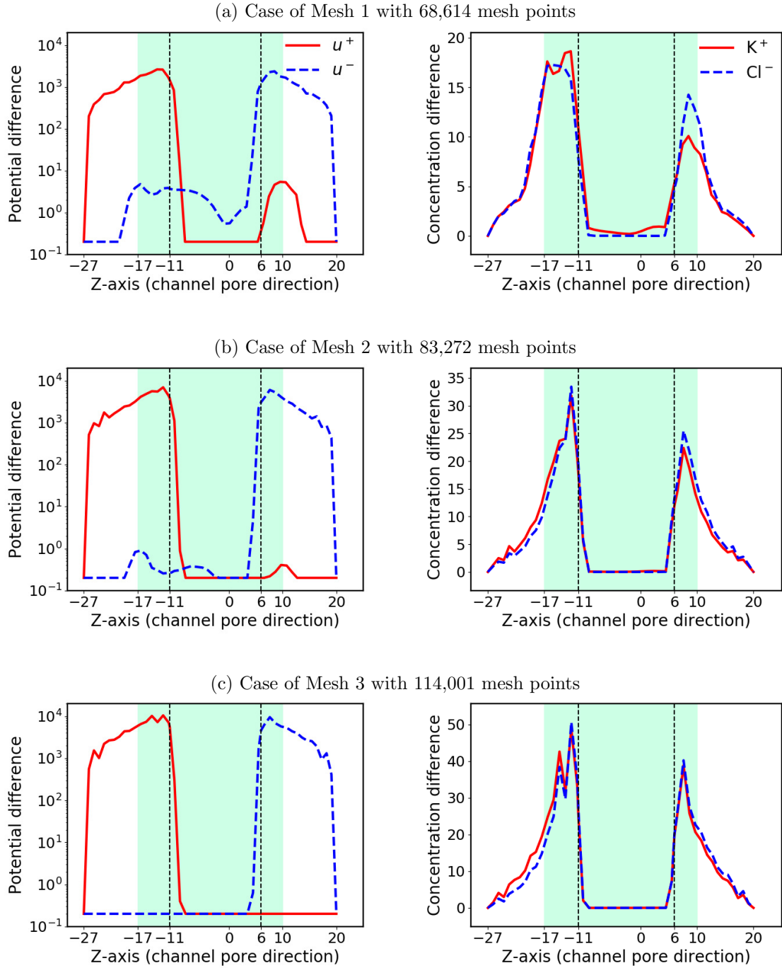
Figure 10: Differences between the potentials u^\pm and ionic concentrations generated by the Dirichlet boundary conditions and those by the Neumann boundary conditions based on Meshes 1, 2, and 3 given in Table 1 for gA in Solvent 2. Here g_b = 2 and g_t = -2 .
