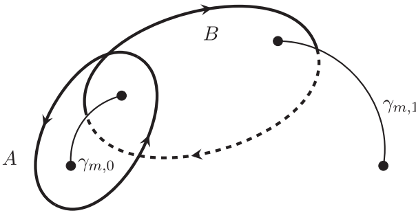
FIGURE 8 The homology basis on \mathfrak{R} . The bold contours are on the top sheet of \mathfrak{R} , and the dashed contours are on the second sheet of \mathfrak{R}
