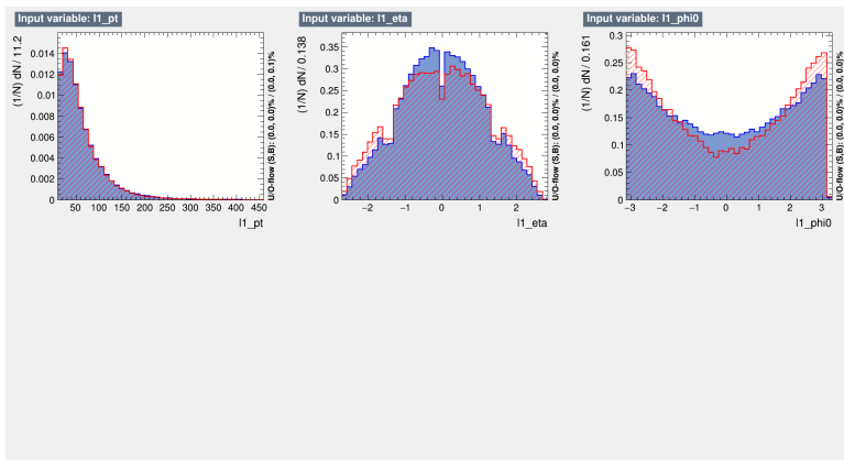
Figure B.27: Normalized training variables for the 4-vector BDT, output by TMVA. CP-odd ttH is denoted as "signal" (blue); CP-even ttH is denoted as "background" (red). Variables shown are, from left to right, top row to bottom row: p_T of leading lepton, \eta of leading lepton, \phi of leading lepton (measured with respect to the Higgs candidate)
