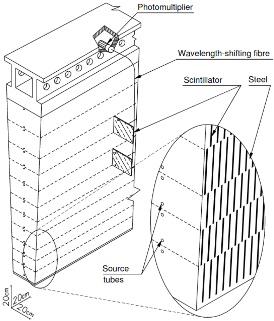
Figure 3.8: A diagram of the TileCal geometry [43]
