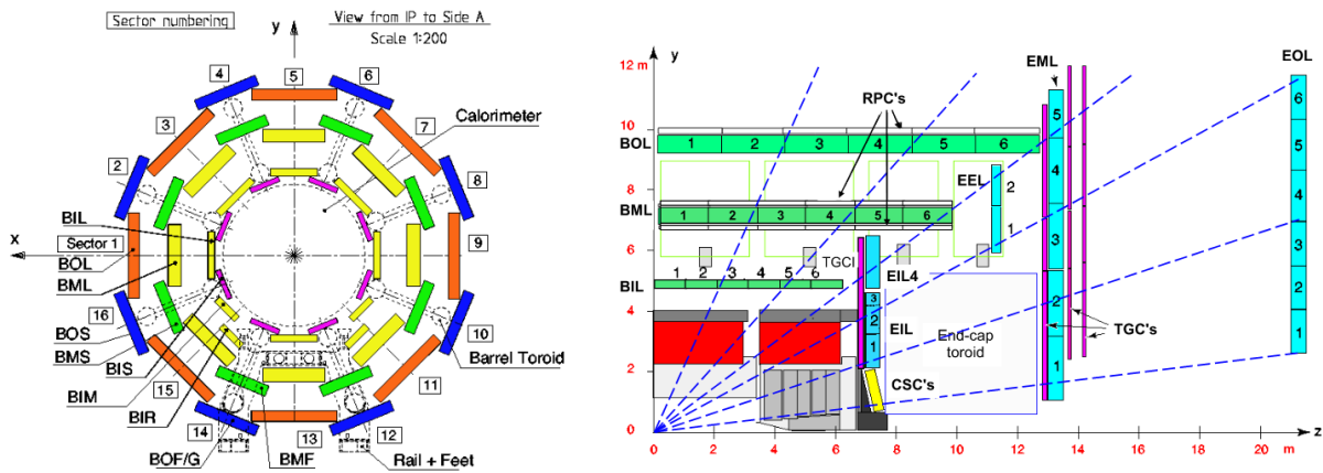
Figure 3.12: A diagram of the MDT chamber geometry from two positions, one looking down the beam pipe and one alongside the detector. [43]
