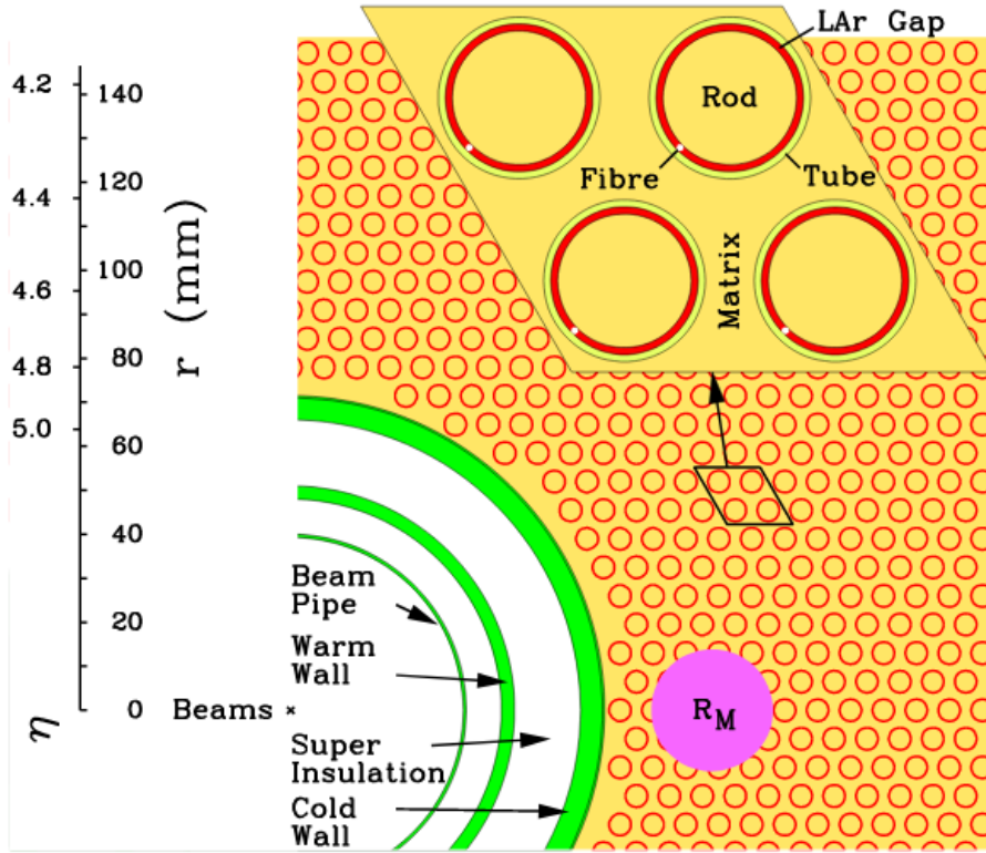
Figure 3.9: A diagram of the FCAL geometry [43]
