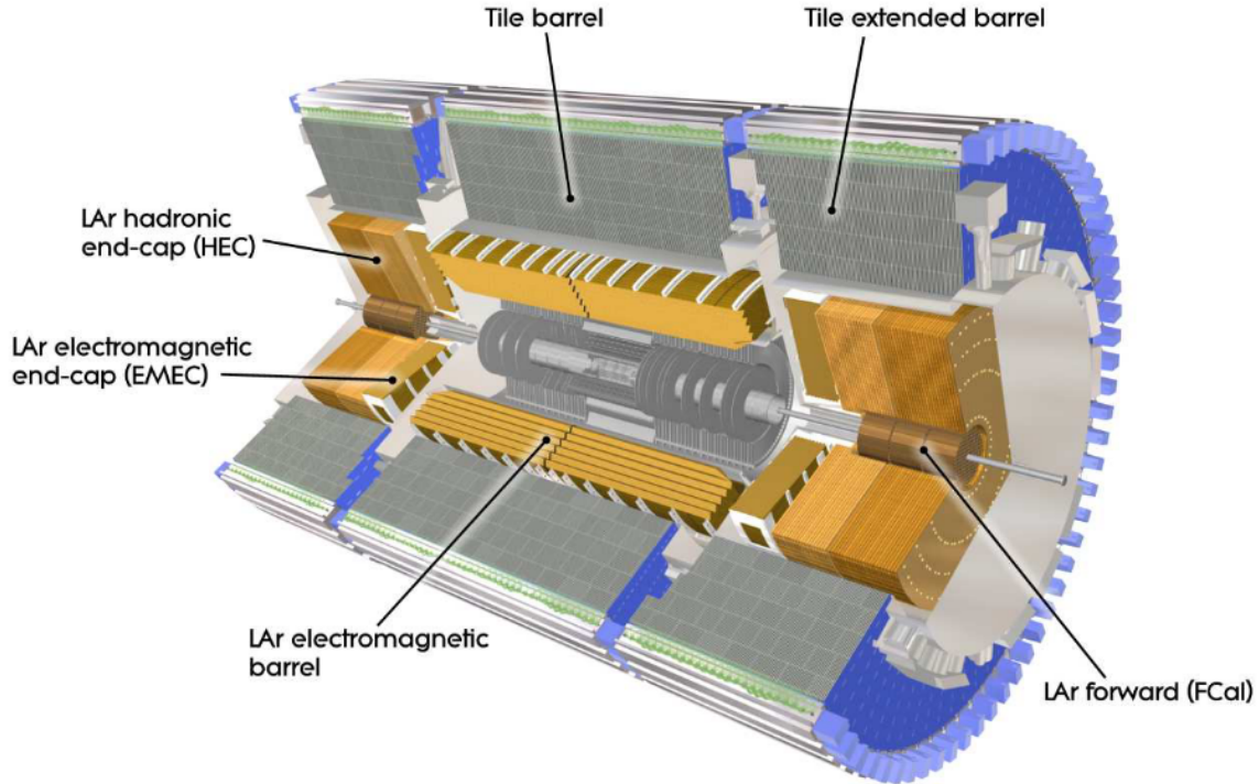
Figure 3.5: An illustration of the ATLAS calorimeter systems. [43]
