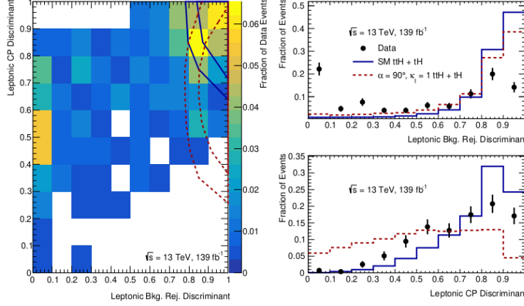
Figure 7.16: Distribution of events from TI sidebands, CP even signal, and CP odd signal in the 2D background rejection BDT vs. CP BDT plane in the leptonic category are shown in full color, black, and red contours, respectively, along with 1D projections onto each BDT score. Inner (outer) contours contain 25% (50%) of signal events.
