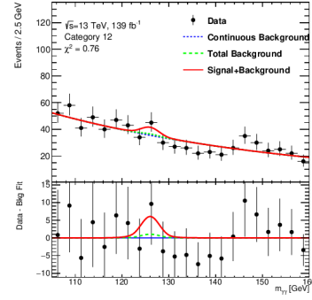
(f) Category 12: m_{\gamma\gamma} (GeV)
