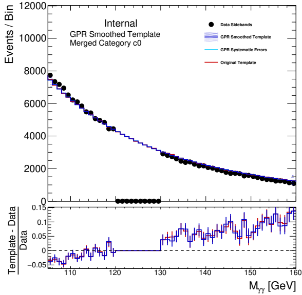
(a) GG2H_0J_PTH_0_10_0
