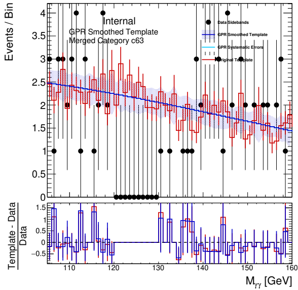
(a) QQ2HQQ_GE2J_MJJ_GT700_PTH_GT200_1
