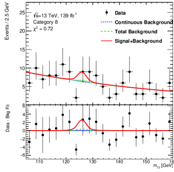
(b) Category 8: m_{\gamma\gamma} (GeV)
