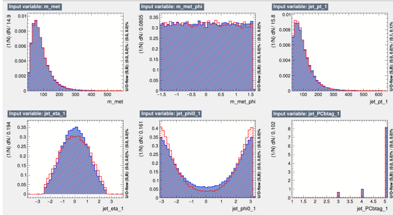
Figure B.24: Normalized training variables for the 4-vector BDT, output by TMVA. CP-odd ttH is denoted as "signal" (blue); CP-even ttH is denoted as "background" (red). Variables shown are, from left to right, top row to bottom row: Magnitude of the event E_T^{miss} , E_T^{miss} \phi (branch cut chosen to range from -\pi/2 to \pi/2 ), p_T of highest b-tag scoring jet, \eta of highest b-tag scoring jet, \phi of highest btag-scoring jet (measured with respect to the Higgs candidate), pseudo-continuous b-tag score of highest btag-scoring jet
