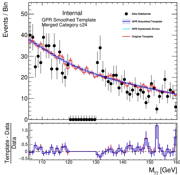
(c) GG2H_GE2J_MJJ_GT700_PTH_0_200_PTHJJ_0_25_2
