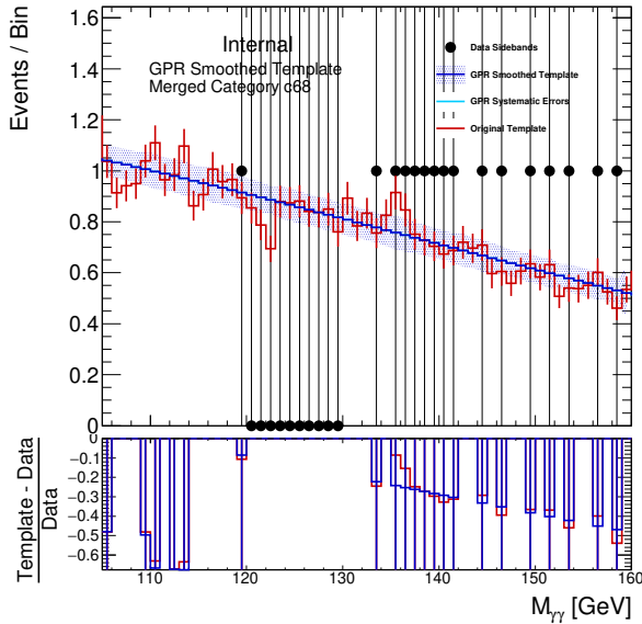
(c) QQ2HLNU_PTV_75_150_1
