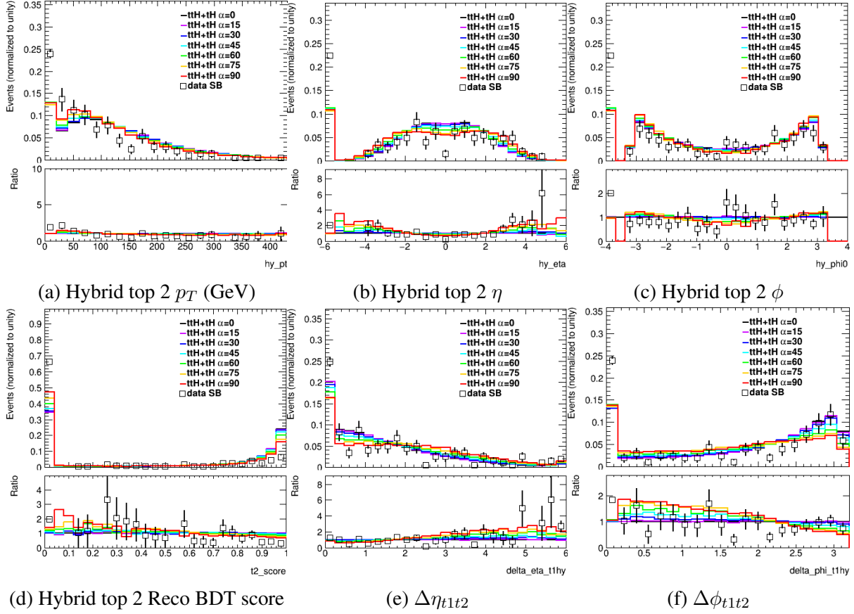
Figure 7.9: Leptonic BDT training variables. The top \phi is calculated with respect to the Higgs candidate. The underflow bins in hybrid top p_T/\eta/\phi and \Delta\eta_{t1t2}/\Delta\phi_{t1t2} contain events where no second (‘hybrid’) top is reconstructed, while the underflow bin in the BDT score contains events with fewer than six jets (i.e., events with either no hybrid top or a hybrid top that is reconstructed using the remaining-jets method). The open squares indicate data in the NTI sideband region, which approximates the shape of the continuum background.
