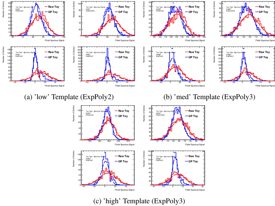
Figure E.38: The distribution of spurious signal for various functions for both the GPR and raw template, using (a) the expPoly2-derived 'low' template, (b) the expPoly3-derived 'med' template, (c) the expPoly3-derived 'high' template, extended by 5 GeV on either side and with a 3 GeV wide feature that is 0.1% of the template integral injected, and fit using a linear error kernel. Each toy in this test has one million events.
