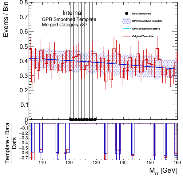
(b) TTH_PTH_GT300_0
