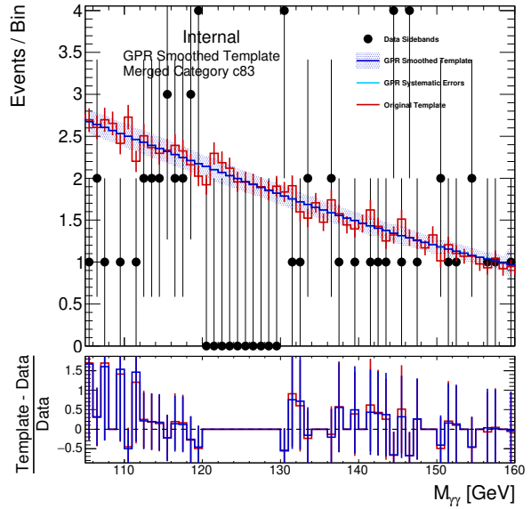
(b) TTH_PTH_60_120_1
