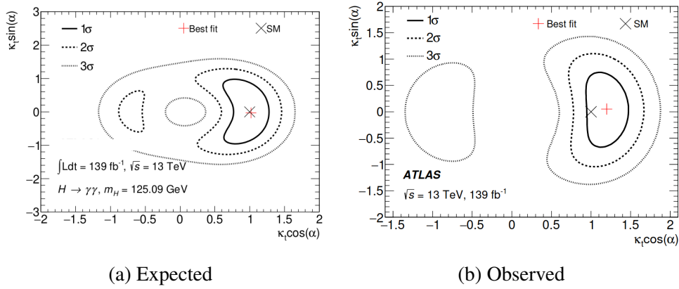
Figure 8.8: Two-dimensional likelihood contour of \kappa_t \cos \alpha and \kappa_t \sin \alpha , with ggF and H \rightarrow \gamma\gamma constrained by the existing Higgs coupling combination result, on (a) post-fit Asimov data and (b) observed data.
