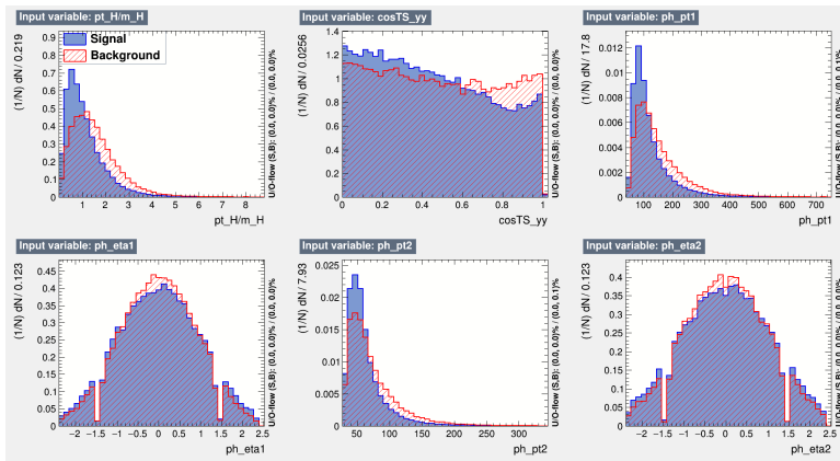
Figure B.23: Normalized training variables for the 4-vector BDT, output by TMVA. CP-odd ttH is denoted as "signal" (blue); CP-even ttH is denoted as "background" (red). Variables shown are, from left to right, top row to bottom row: Higgs candidate p_T (scaled by mass), \cos(\theta^*) , leading photon p_T , leading photon \eta , subleading photon p_T , subleading photon \eta .
