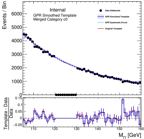
(c) GG2H_1J_PTH_0_60
