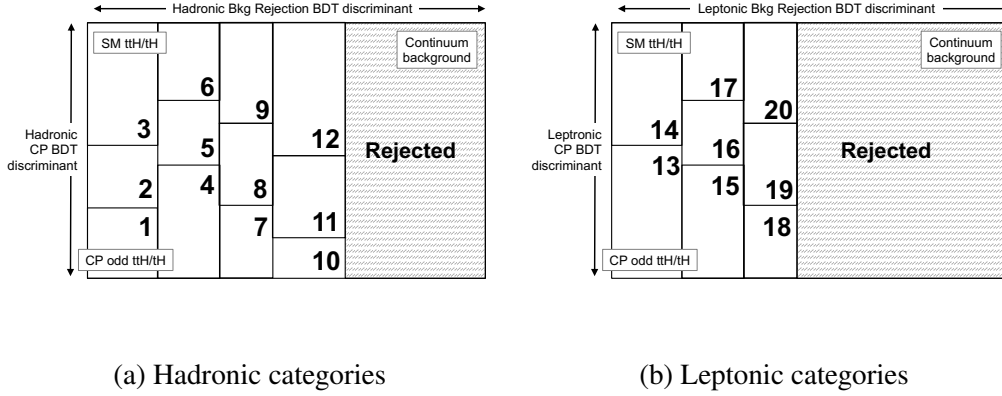
Figure 7.1: Diagram of the 2-dimensional categorization scheme in the hadronic (a) and leptonic (b) channels. The x -axis indicates the background-rejection BDT (SBBDT) score distribution, and the y -axis represents the CP-BDT score distribution. The shaded region indicates rejected events.
