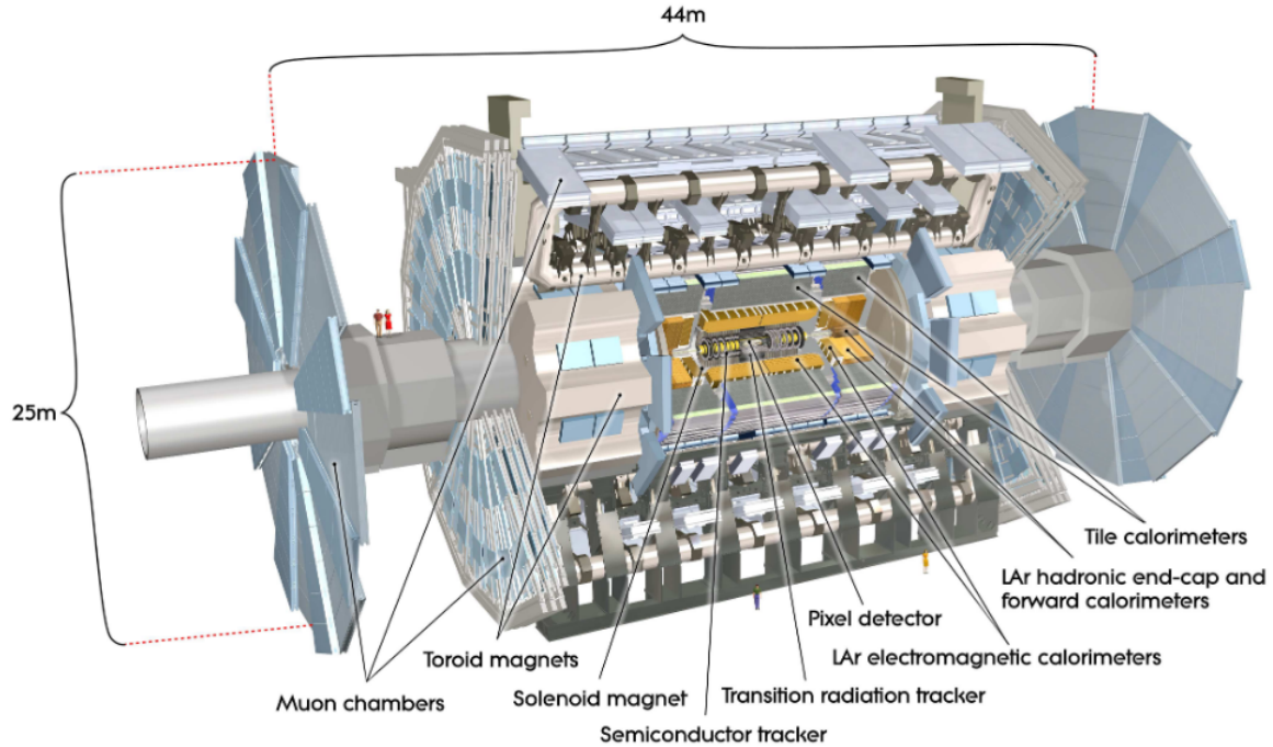
Figure 3.2: A diagram of the various subsystems of the ATLAS detector. [43]
