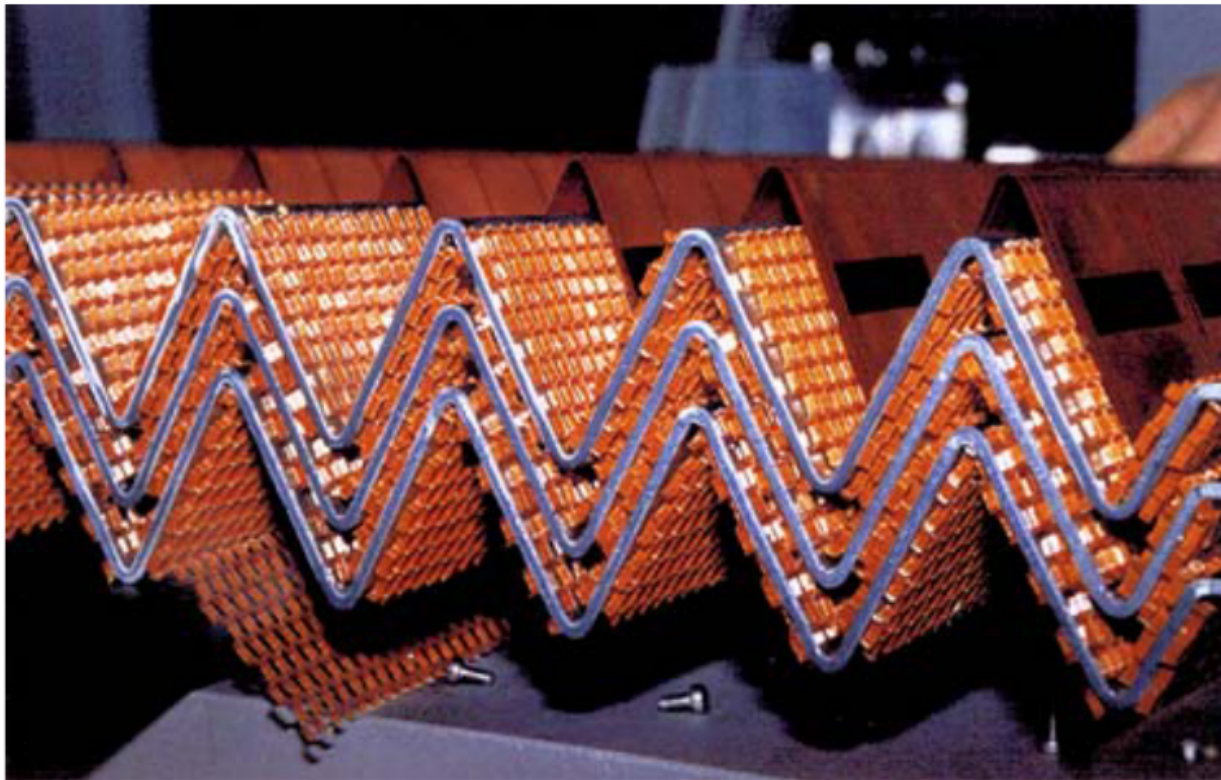
Figure 3.7: A photograph of an ECAL absorber. [52]
