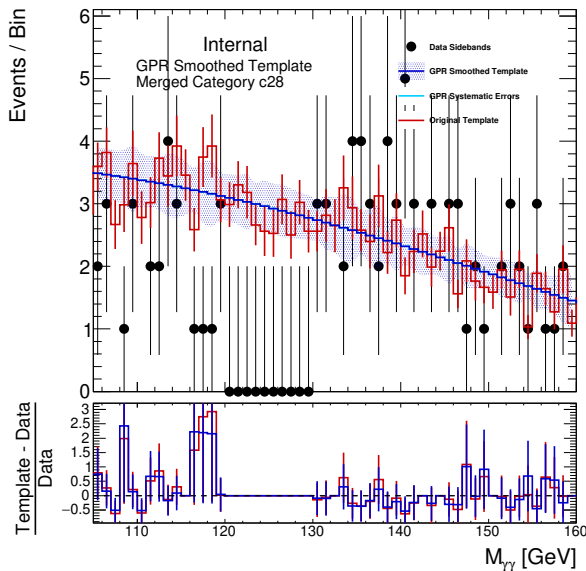
(c) GG2H_PTH_200_300_0
