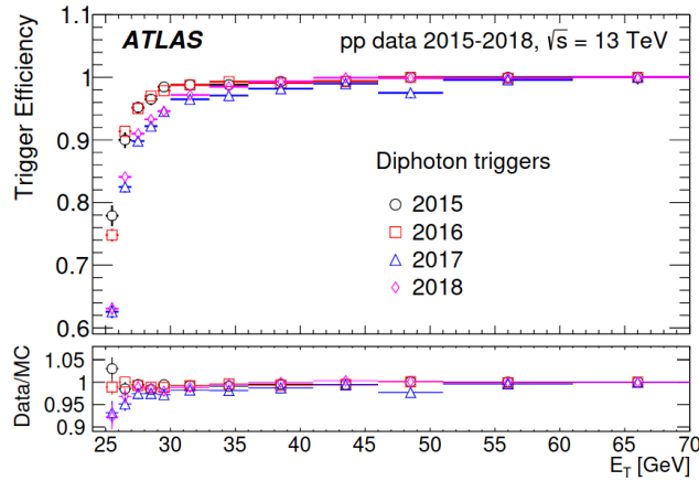
Figure 5.3: Efficiency of the trigger for the different years of the run-2 data taking period as a function of subleading photon E_T .
