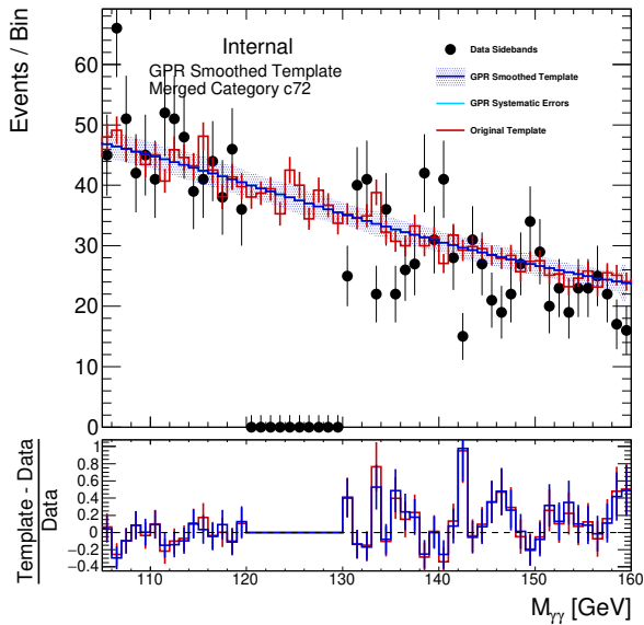
(c) UNSELECTED_ZH
