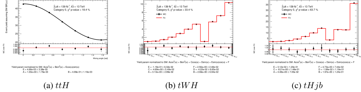
Figure 8.1: Inclusive yield parametrizations as a function of \kappa_t and \alpha , normalized to 139 fb^{-1} .
