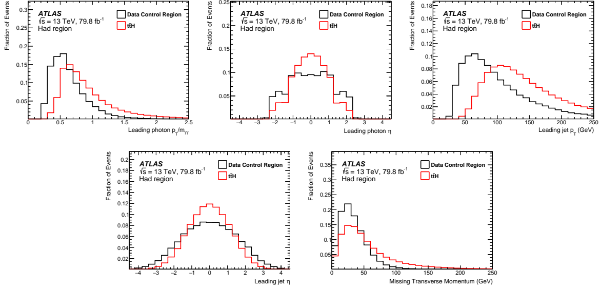
Figure 7.2: Distributions of training variables for the hadronic background-rejection BDT, trained at 79.8 fb^{-1} . Taken from [5].
