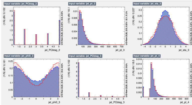
Figure B.5: Normalized training variables for the 4-vector BDT, output by TMVA. CP-odd ttH is denoted as "signal" (blue); CP-even ttH is denoted as "background" (red). Variables shown are, from left to right, top row to bottom row: pseudo-continuous b-tag score of second-highest btag-scoring jet, p_T of third-highest b-tag scoring jet, \eta of third-highest b-tag scoring jet, \phi of third-highest btag-scoring jet (measured with respect to the Higgs candidate), pseudo-continuous b-tag score of third-highest btag-scoring jet, p_T of fourth-highest b-tag scoring jet.
