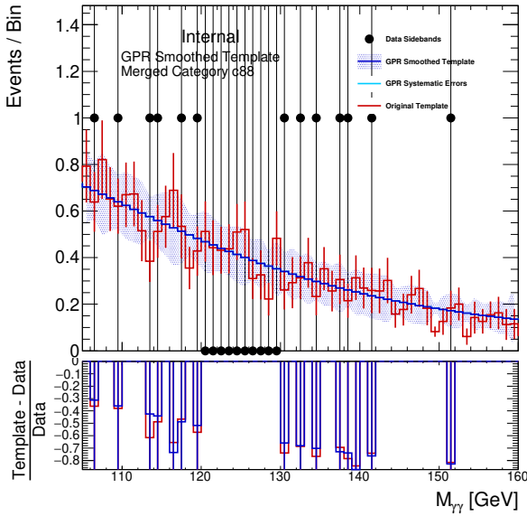
(c) THJB_0
