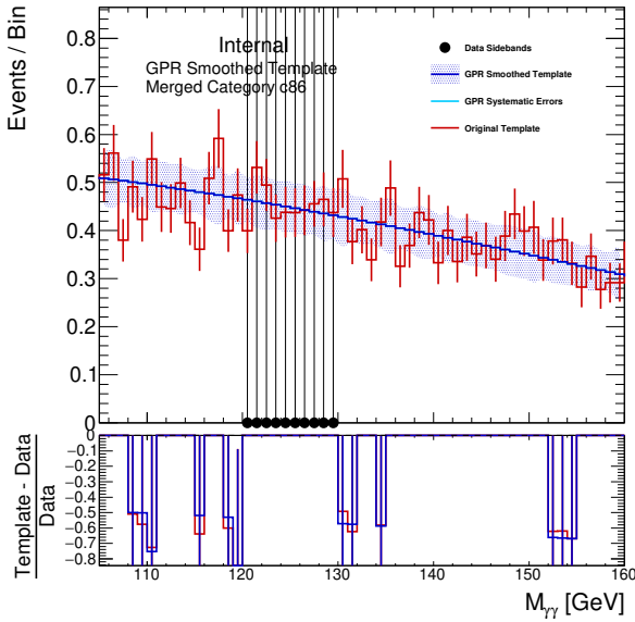
(a) TTH_PTH_200_300_0
