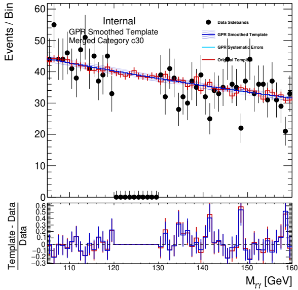
(a) GG2H_PTH_200_300_2
