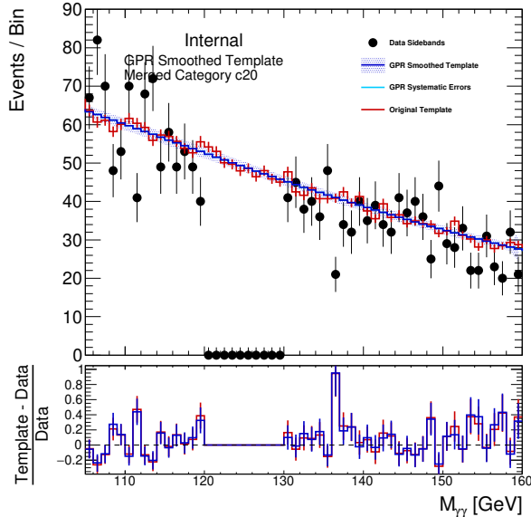
(c) GG2H_GE2J_MJJ_350_700_PTH_0_200_PTHJJ_GT25...1
