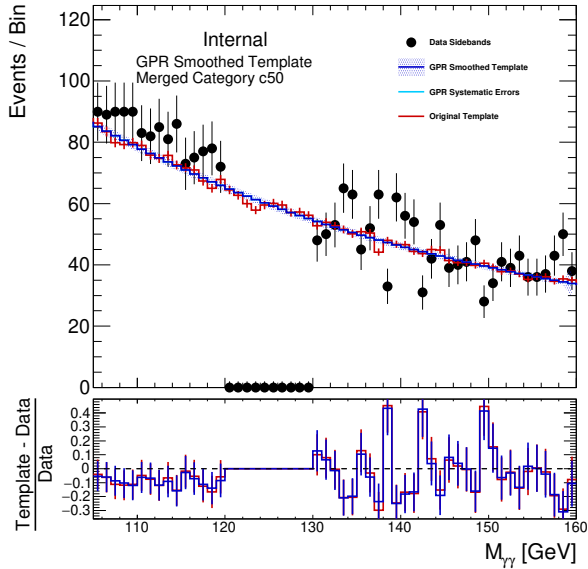
(a) QQ2HQQ_GE2J_MJJ_120_350...2
