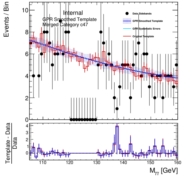
(b) QQ2HQQ_GE2J_MJJ_60_120_1
