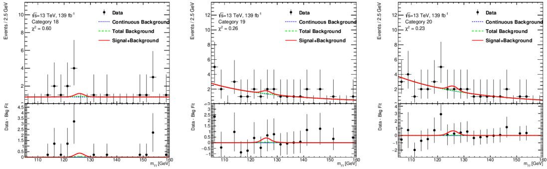
(f) Category 18: m_{\gamma\gamma} (GeV) (g) Category 19: m_{\gamma\gamma} (GeV) (h) Category 20: m_{\gamma\gamma} (GeV)
