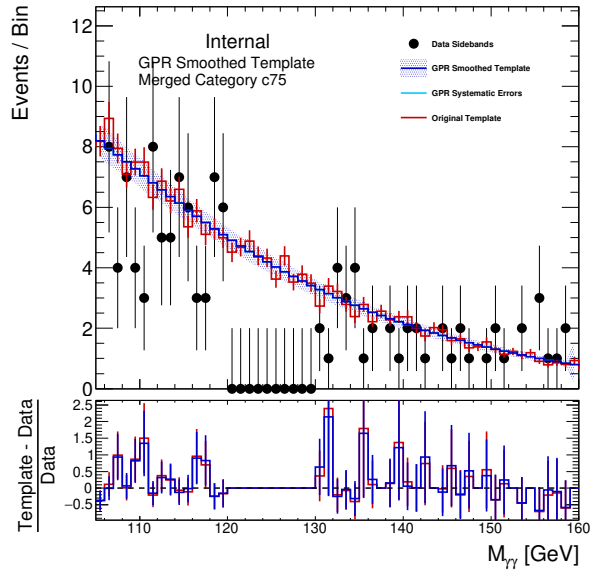
(b) HLL_PTV_75_150_1
