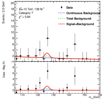
(a) Category 7: m_{\gamma\gamma} (GeV)
