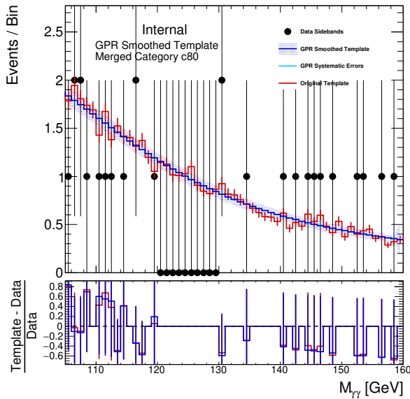
(c) TTH_PTH_0_60_0
