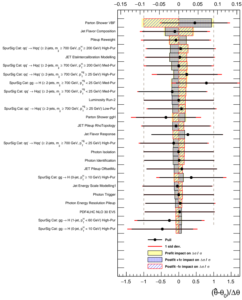
Figure C.3: Nuisance parameter "pull plots" for the VBF cross-section in the five-production-mode fit. The nuisance parameters are ranked by their impact on the cross-section measurement. These show the pre-fit and post-fit impact of various nuisance parameters on the cross-section measurement (colored and shaded boxes, corresponding to the top x-axis), as well as the "pull" (change in mean and spread between pre- and post-fit nuisance parameters, corresponding to the bottom x-axis).
