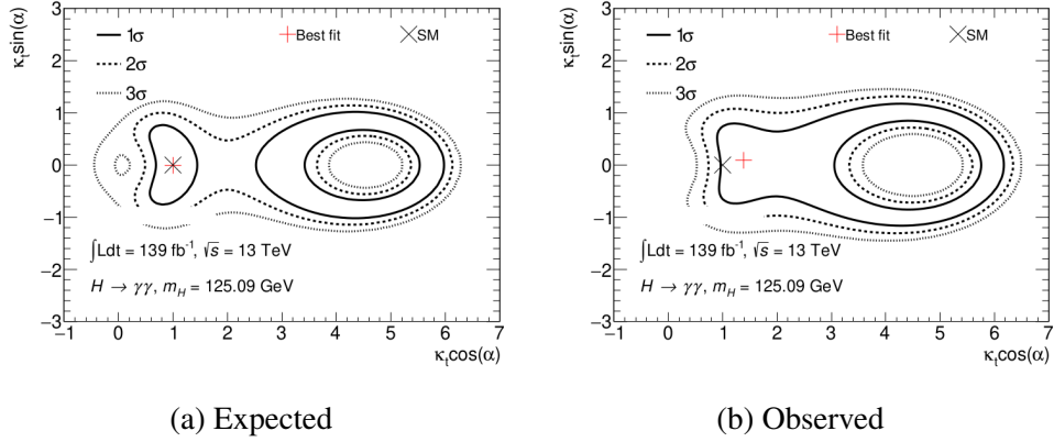
Figure 8.10: Two-dimensional likelihood contour of \kappa_t \cos \alpha and \kappa_t \sin \alpha , with ggF and H \rightarrow \gamma\gamma parameterized as function of \kappa_t and \alpha , on (a) post-fit Asimov data and (b) observed data.
