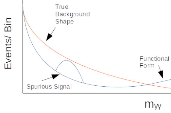
Figure 6.2: A cartoon depicting the spurious signal procedure. The true background shape in red is modeled by an analytic function in blue. The spurious signal resulting from this mismodelling is the maximum signal yield extracted from the blue “spurious signal” bump, fit over a window of 120 \text{ GeV} < m_{\gamma\gamma} < 130 \text{ GeV} .
