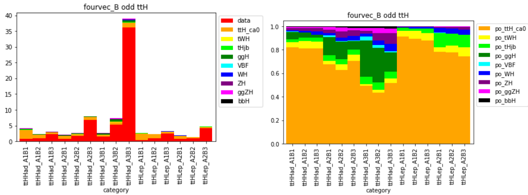
(c) Event yield (CP odd ttH )
