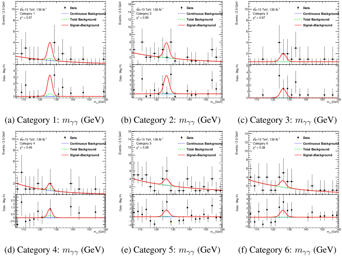
Figure 8.2: Diphoton invariant mass spectrum ( m_{\gamma\gamma} ) in the first six hadronic categories. The fitted continuum background is shown in blue the, total background including non-top Higgs processes is shown in green, and total fitted signal plus background is shown in red.
