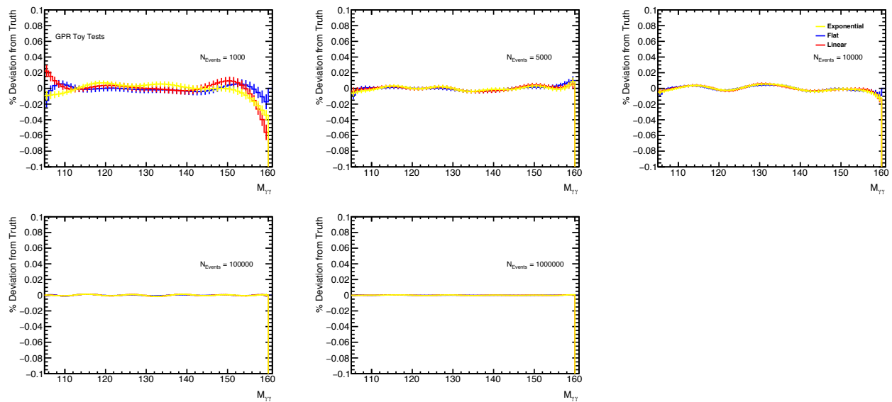
Figure E.9: The per-bin percent deviation of the smoothed template from the unsmoothed template for a variety of different choices of GP mean, using an ExpPoly2 function as the toy basis. The yellow shape shows the results using an Exponential mean, the blue shape shows the result uses a flat mean, and the red shape uses a linear mean. Templates contain, from left to right and top to bottom, 1000 events, 5,000 events, 10,000 events, 100,000 events, and one million events.
