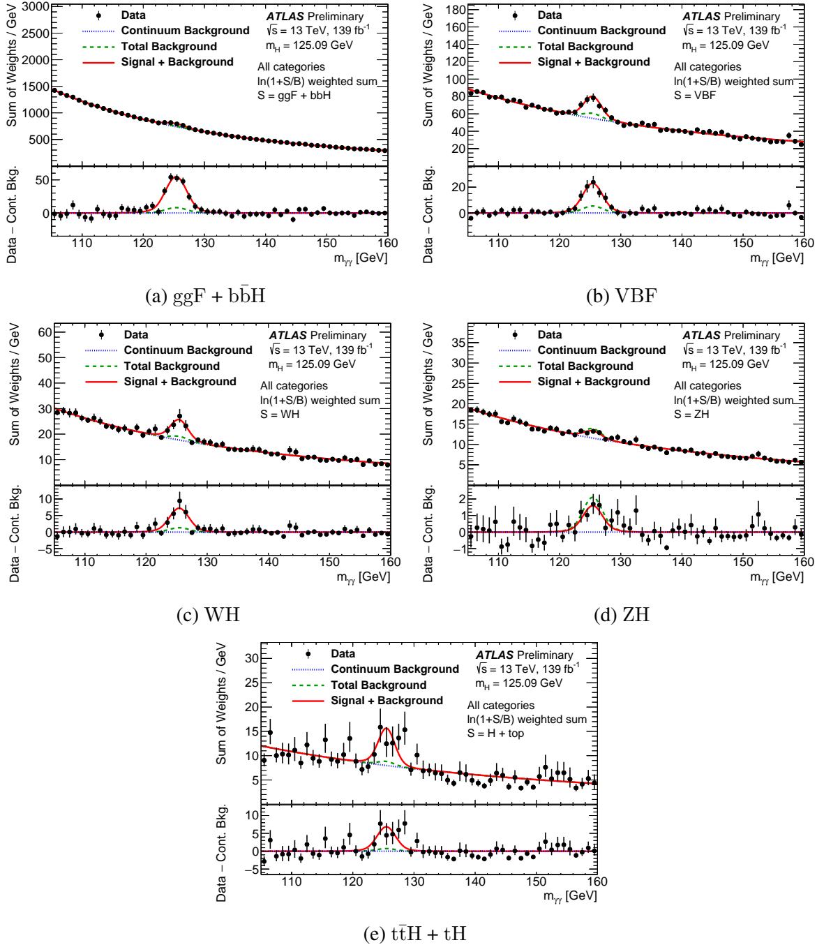
Figure 9.12: Combined diphoton invariant mass distributions for the five-production-mode fit. The events in each category are weighted by \ln(1 + S/B) , where S and B are the expected signal and background yields in this category within the smallest m_{\gamma\gamma} window containing 90% of the signal events. The weighted sum of the signal plus background fits is represented by the solid line, while the blue dotted line represents the weighted sum of the background functional forms. Only Higgs boson events from the targeted production processes in each category are considered as signal events in these plots; Higgs boson events from other processes are treated as part of the background.
