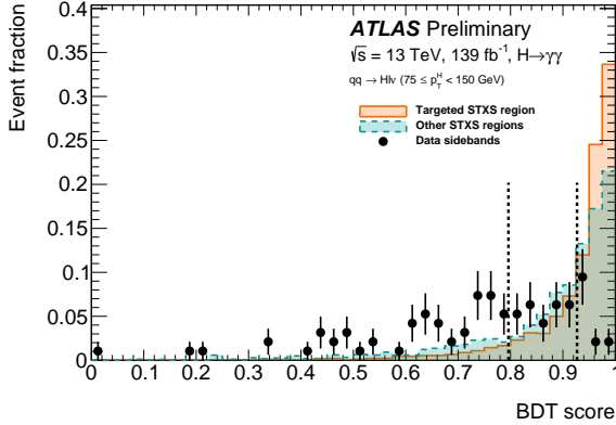
(c) qq \rightarrow Hlv ( 75 \leq p_T^H < 150 \text{ GeV} )
