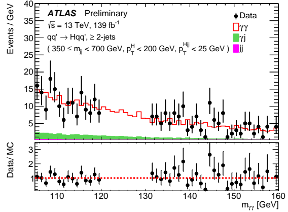
(b) qq' \rightarrow Hqq' ( \geq 2 -jets, 350 \leq m_{jj} < 700 GeV, p_T^H < 200 GeV, p_T^{Hjj} < 25 GeV)
