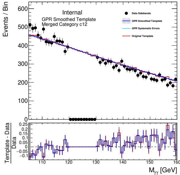
(c) GG2H_GE2J_MJJ_0_350_PTH_60_120_1
