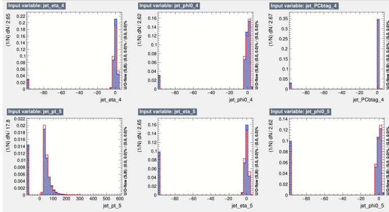
Figure B.6: Normalized training variables for the 4-vector BDT, output by TMVA. CP-odd ttH is denoted as "signal" (blue); CP-even ttH is denoted as "background" (red). Variables shown are, from left to right, top row to bottom row: \eta of fourth-highest b-tag scoring jet, \phi of fourth-highest btag-scoring jet (measured with respect to the Higgs candidate), pseudo-continuous b-tag score of fourth-highest btag-scoring jet, p_T of fifth-highest b-tag scoring jet, \eta of fifth-highest b-tag scoring jet, \phi of fifth-highest btag-scoring jet (measured with respect to the Higgs candidate)
