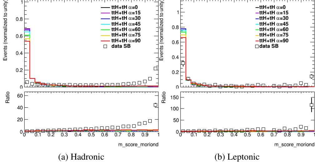
Figure 7.4: SB BDT score for the sum of ttH , tHjb and tWH , with relative weights according to their expected cross sections. Shown in (a) for the hadronic channel and (b) for the leptonic channel, for various CP mixing scenarios. The open squares show data in the NTI sideband region, which approximates the shape of the continuum background.
