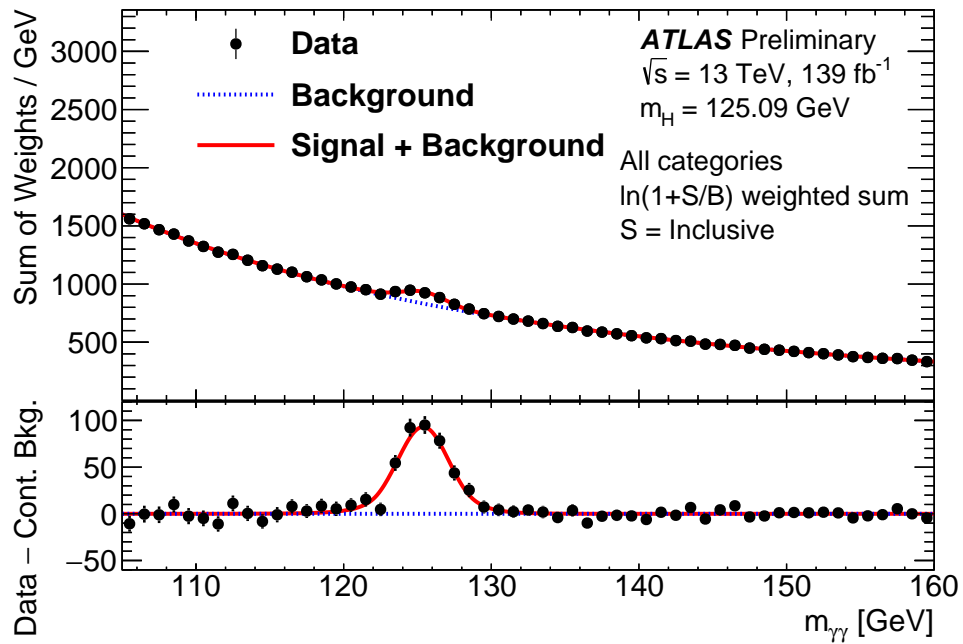
Figure 9.11: The inclusive diphoton invariant mass distribution of events from all analysis categories. The events in each category are weighted by \ln(1 + S/B) , where S and B are the expected signal and background yields in this category within the smallest m_{\gamma\gamma} window containing 90% of the signal events. The weighted sum of the signal plus background fits is represented by the solid line, while the blue dotted line indicates the weighted sum of the background functional forms.
