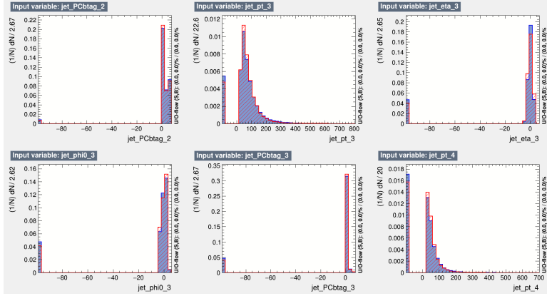
Figure B.12: Normalized training variables for the 4-vector BDT, output by TMVA. CP-odd t\bar{t}H is denoted as "signal" (blue); CP-even t\bar{t}H is denoted as "background" (red). Variables shown are, from left to right, top row to bottom row: pseudo-continuous b-tag score of second-highest btag-scoring jet, p_T of third-highest b-tag scoring jet, \eta of third-highest b-tag scoring jet, \phi of third-highest btag-scoring jet (measured with respect to the Higgs candidate), pseudo-continuous b-tag score of third-highest btag-scoring jet, p_T of fourth-highest b-tag scoring jet.
