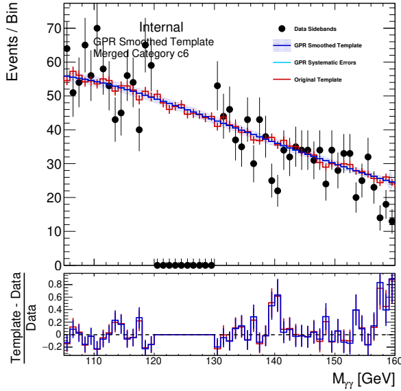
(a) GG2H_1J_PTH_120_200_0
