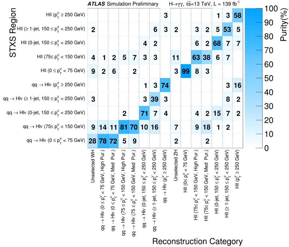
Figure 9.6: The correspondence between analysis category and STXS truth bins, in terms of the percentage contribution of a given STXS truth bin (y-axis) to the Higgs signal yield in a given analysis category (x-axis) for qq \rightarrow H\ell\ell and qq \rightarrow H\ell\nu categories and truth bins. Entries with a value below 1% are omitted.
