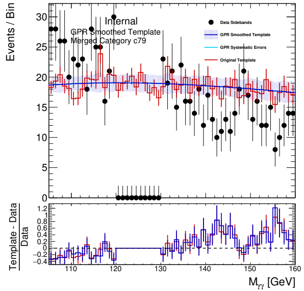
(b) UNSELECTED_TOP
