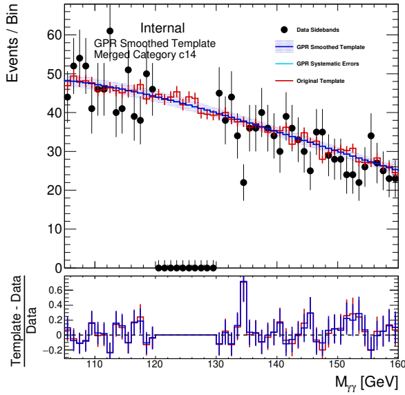
(a) GG2H_GE2J_MJJ_0_350_PTH_120_200_0
