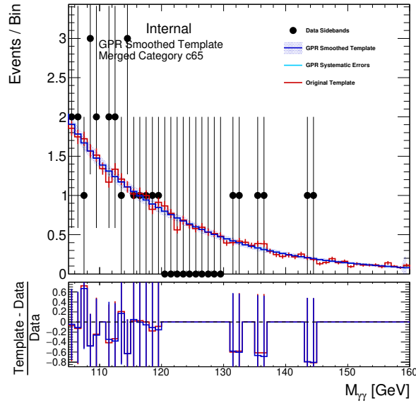
(c) QQ2HLNU_PTV_0.75_0
