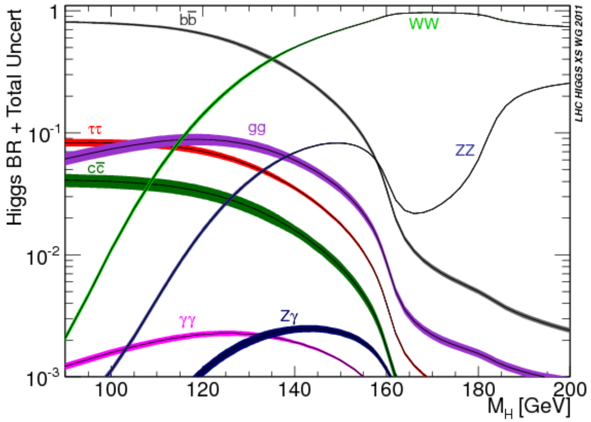
Figure 2.7: The branching ratio of the Higgs to various final state particles as a function of its mass (now known to be 125 GeV), from reference [18].
