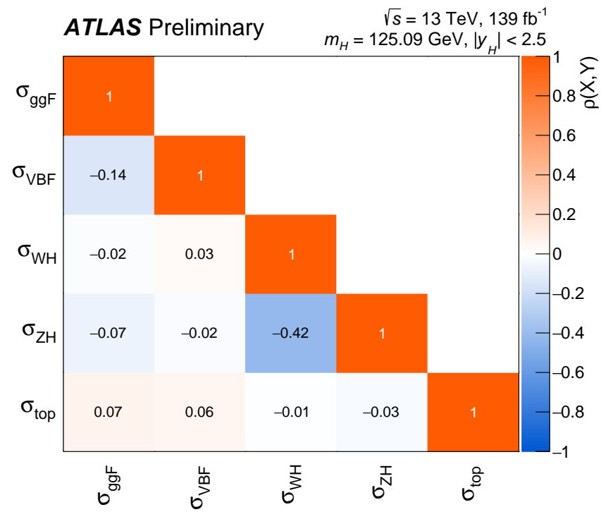
Figure 9.14: Correlation matrix for the five-production-mode fit.
