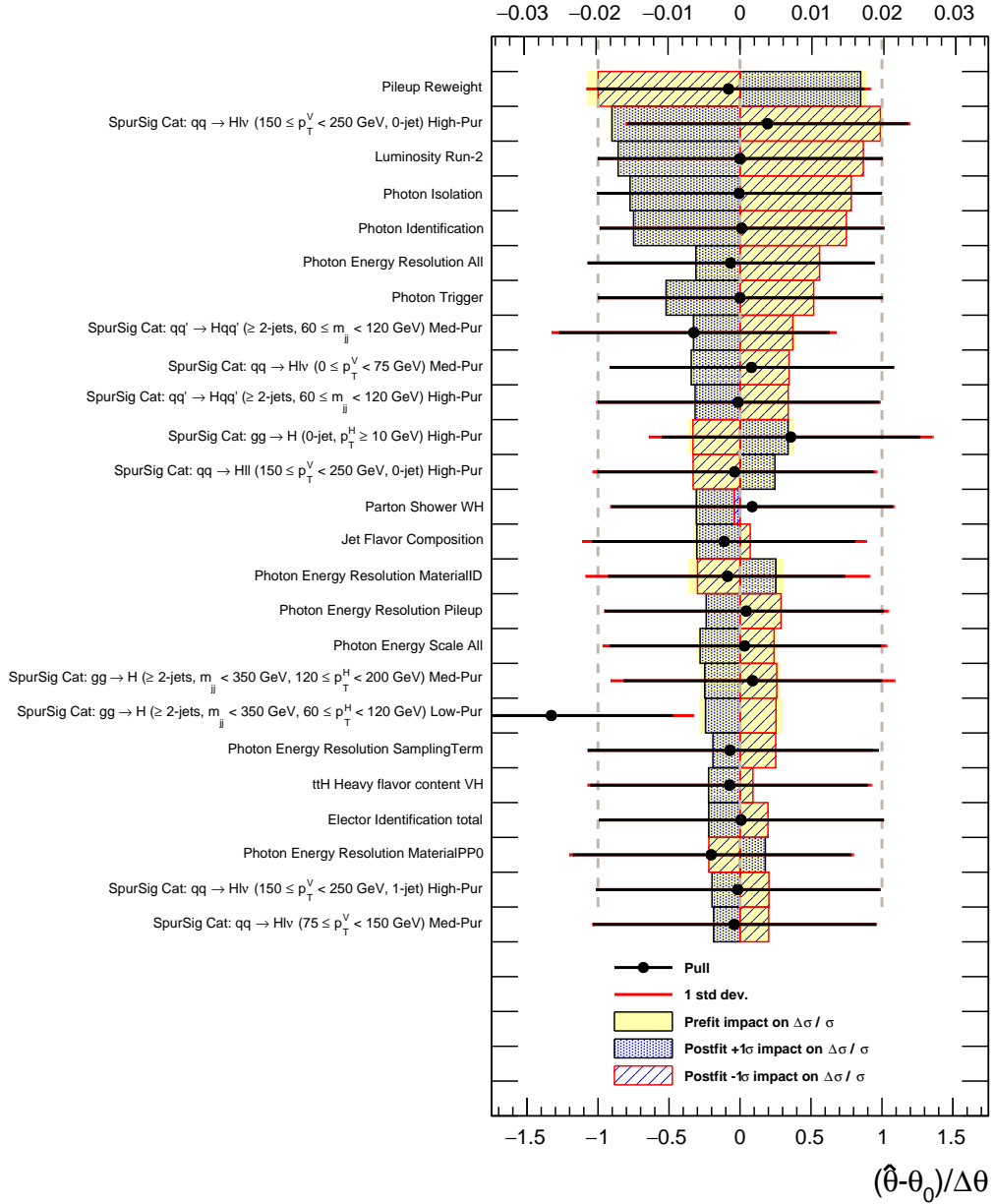
Figure C.4: Nuisance parameter "pull plots" for the WH cross-section in the five-production-mode fit. The nuisance parameters are ranked by their impact on the cross-section measurement. These show the pre-fit and post-fit impact of various nuisance parameters on the cross-section measurement (colored and shaded boxes, corresponding to the top x-axis), as well as the "pull" (change in mean and spread between pre- and post-fit nuisance parameters, corresponding to the bottom x-axis).
