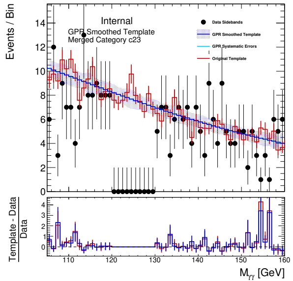
(b) GG2H_GE2J_MJJ_GT700_PTH_0_200_PTHJJ_0_25_1
