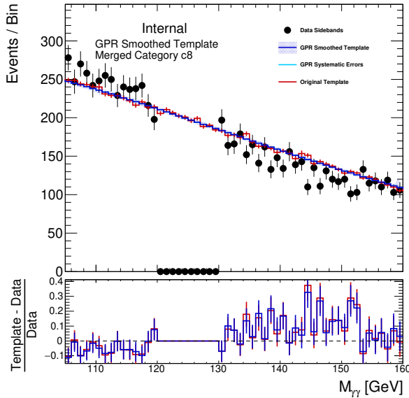
(c) GG2H_GE2J_MJJ_0_350_PTH_0_60_0
