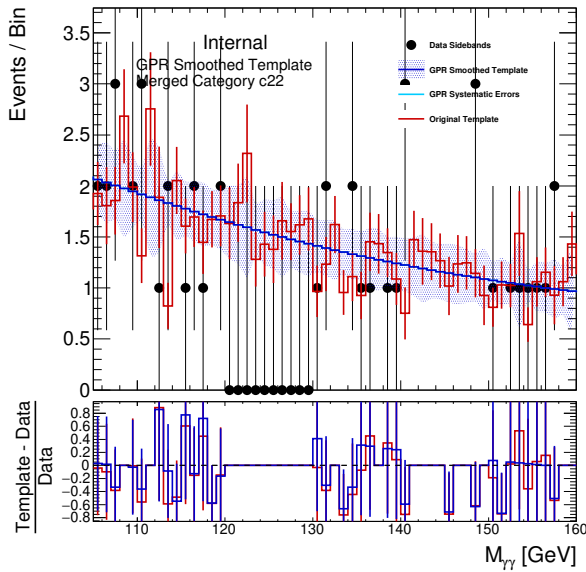
(a) GG2H_GE2J_MJJ_GT700_PTH_0_200_PTHJJ_0_25_0
