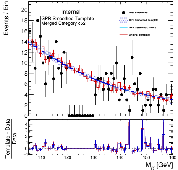
(b) QQ2HQQ_GE2J_MJJ_350_700_PTH_0_200_PTHIJ_0_25...1
