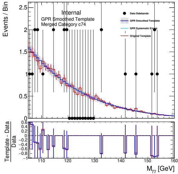
(a) HLL_PTV_75_150_0
