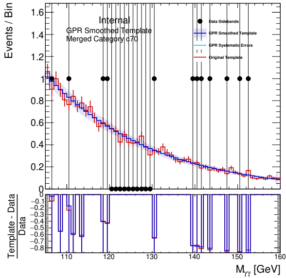
(a) QQ2HLNU_PTV_150_250_GE1J_0
