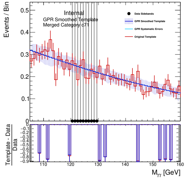
(b) QQ2HLNU_PTV_GT250_0
