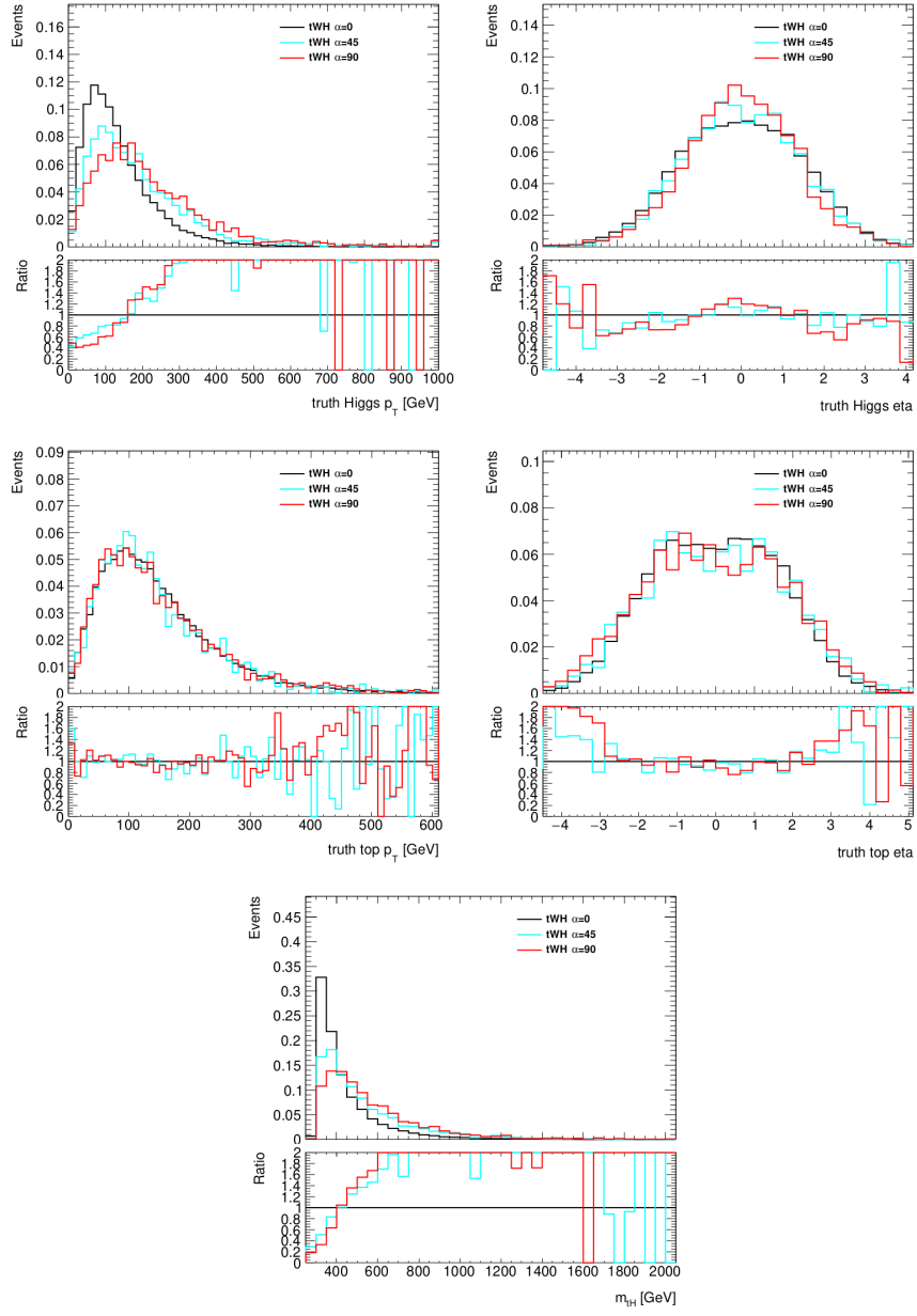
Figure 7.6: Truth-level distributions in tWH Monte Carlo of the Higgs boson p_T and \eta (top), top quark p_T and \eta (middle) and invariant mass of the top-Higgs system (bottom) for different values of the CP mixing angle \alpha .
