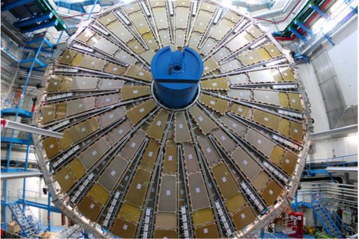
Figure 3.13: A photograph of the TGC wheels. [62]
