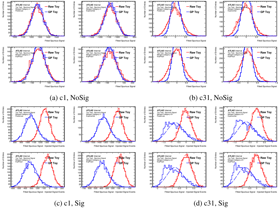
Figure E.29: The distribution of spurious signal for various functions for both the GPR and raw template with and without a Standard-Model expectation-sized signal injected, using the c1 and c31 templates as a basis.
