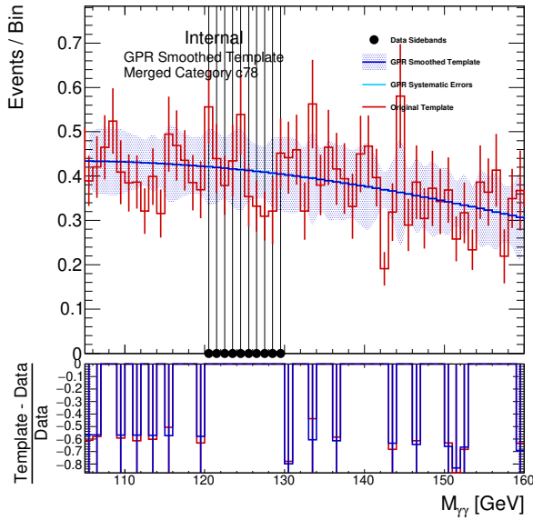
(a) HLL_PTV_GT250_0
