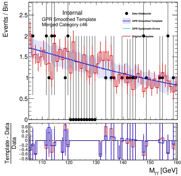
(a) QQ2HQQ_GE2J_MJJ_60_120_0
