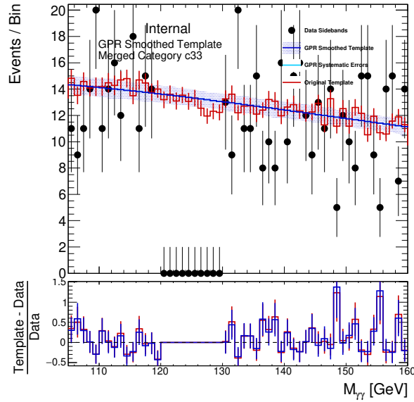
(c) GG2H_PTH_300_450_2
