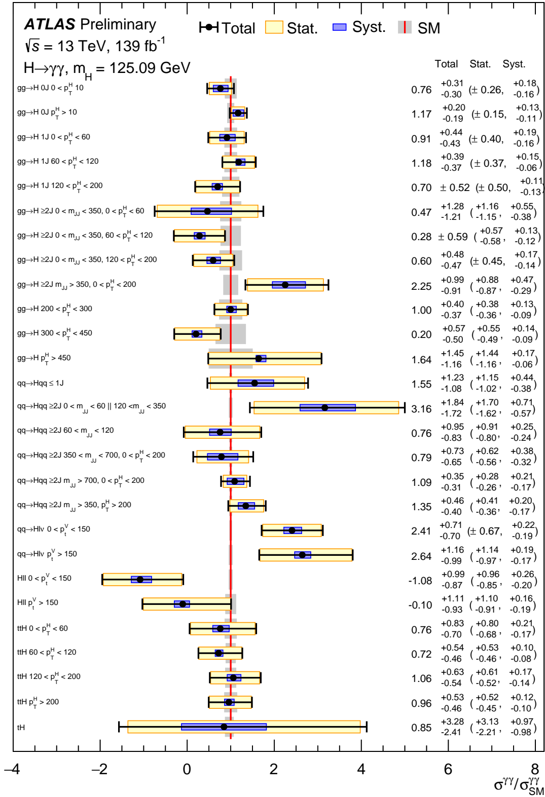
Figure 9.15: Measured cross sections times branching fraction for the cross sections in each analysis category. The black error bars, blue boxes and yellow boxes show the total, systematic, and statistical uncertainties, respectively, while the gray bands show the theory uncertainties.
