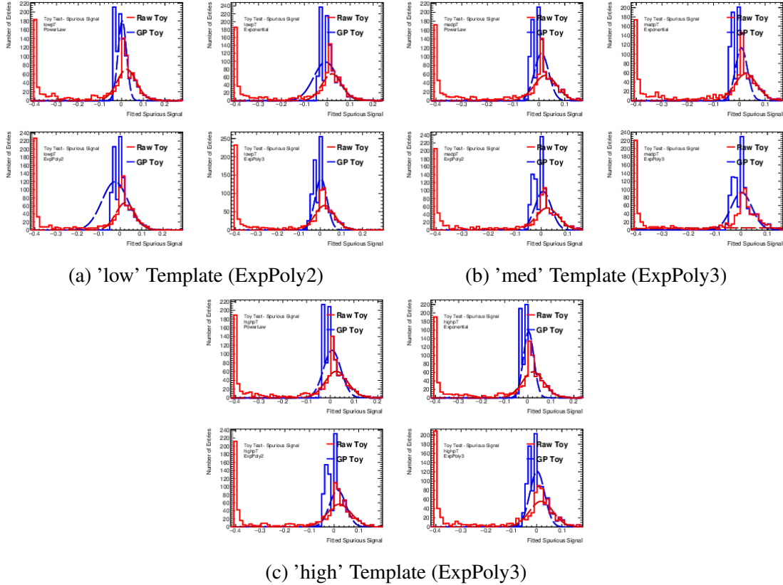
Figure E.18: The distribution of spurious signal for various functions for both the GPR and raw template, using (a) the expPoly2-derived 'low' template, (b) the expPoly3-derived 'med' template, (c) the expPoly3-derived 'high' template, extended by 5 GeV on either side, and fit using a linear error kernel. Each toy in this test has 10 events.
