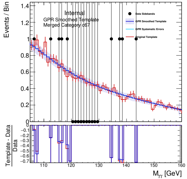
(b) QQ2HLNU_PTV_75_150_0
