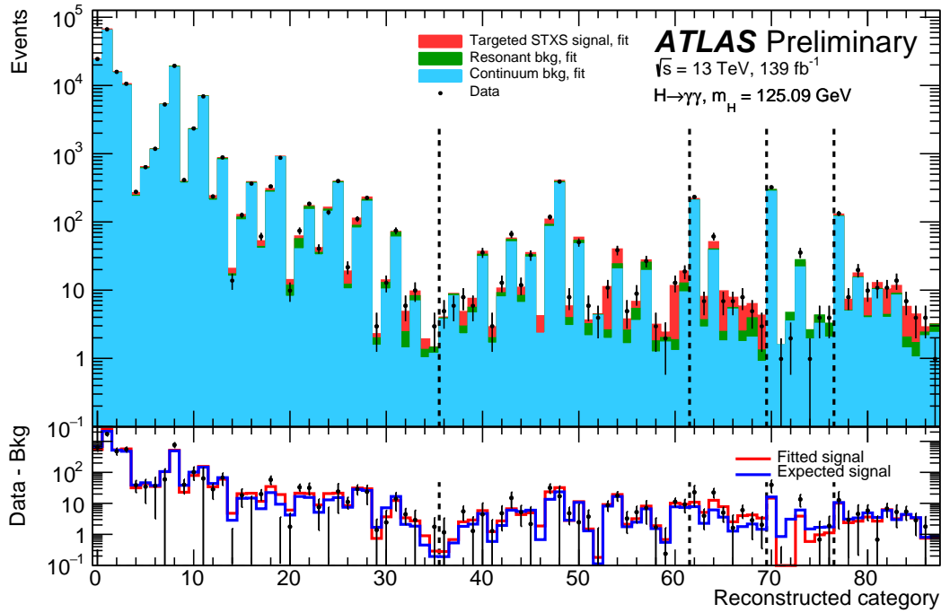
Figure 9.17: Event yields in the diphoton mass range containing 90% of the signal events for all 88 categories. In each category, the fitted targeted STXS-bin signal yield is shown in red, the yield of other Higgs boson processes is shown in green, and the fitted continuum background is shown in blue. The 27 STXS cross-sections are parameters of interest profiled in the fit. The vertical lines separate the ggF , VBF , WH , ZH , and t\bar{t}H and tH categories. In the top panel, the signal and backgrounds are stacked, while in the bottom panel, the background is subtracted from the data yield and only the fitted and expected signal is shown.
