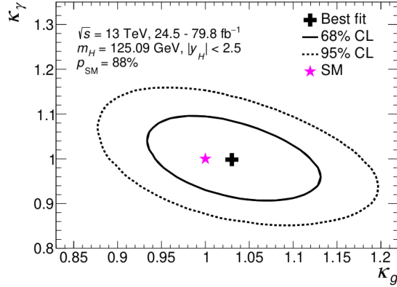
Figure 8.7: Two-dimensional contour from the ATLAS Higgs coupling combination. The best fit value of (\kappa_g, \kappa_\gamma) is shown with 1 and 2 \sigma contours. This is used as a constraint on ggF and H \rightarrow \gamma\gamma in the fit.
