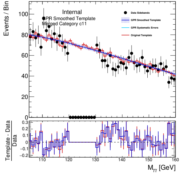
(b) GG2H_GE2J_MJJ_0_350_PTH_60_120_0
