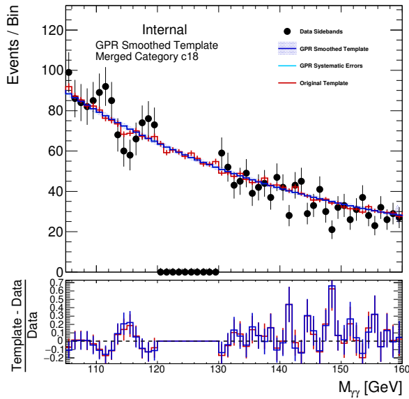
(a) GG2H_GE2J_MJJ_350_700_PTH_0_200_PTHJJ_0_25...2
