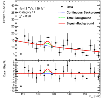
(e) Category 11: m_{\gamma\gamma} (GeV)
