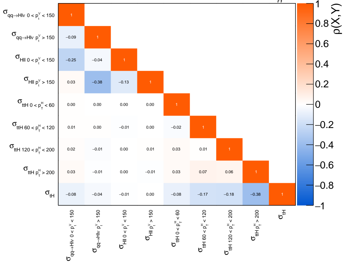
Figure 9.19: The subset of the correlation matrix of the STXS measurements shown in Figure 9.16 corresponding to the qq \rightarrow Hll , qq \rightarrow H\nu , t\bar{t}H , tWH , and tHjb STXS regions.
