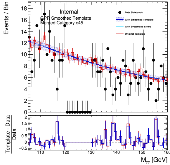
(c) QQ2HQQ_GE2J_MJJ_0_60_2
