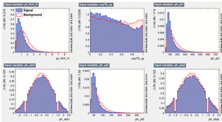
Figure B.9: Normalized training variables for the 4-vector BDT, output by TMVA. CP-odd ttH is denoted as "signal" (blue); CP-even ttH is denoted as "background" (red). Variables shown are, from left to right, top row to bottom row: Higgs candidate p_T (scaled by mass), \cos(\theta^*) , leading photon p_T , leading photon \eta , subleading photon p_T , and subleading photon \eta .
