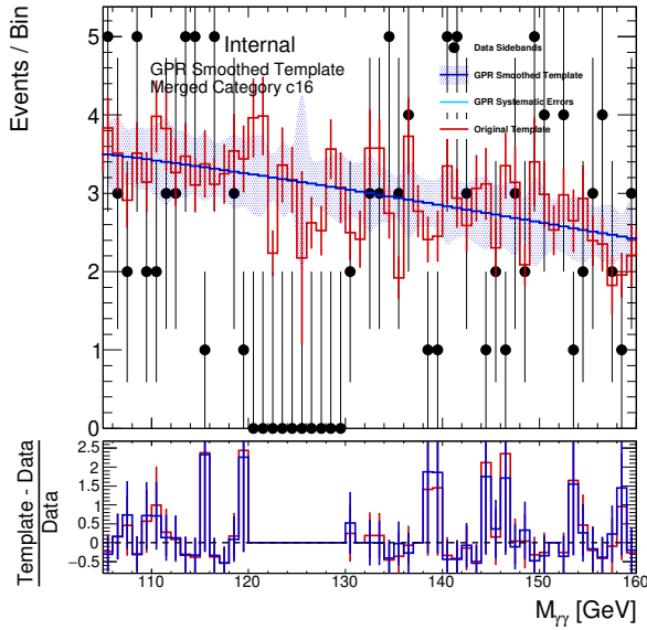
(c) GG2H_GE2J_MJJ_350_700_PTH_0_200_PTHJJ_0_25_0
