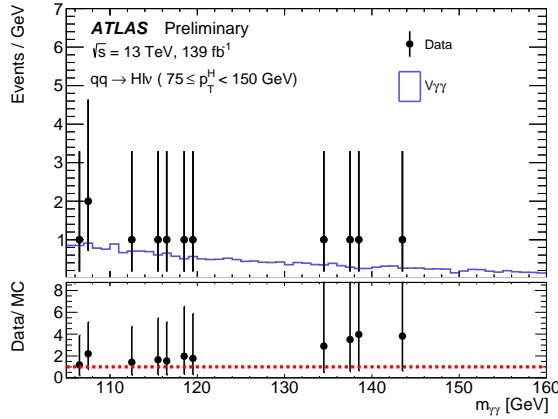
(c) qq \rightarrow H\nu ( 75 \leq p_T^H < 150 GeV)
