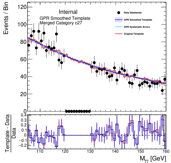
(b) GG2H_GE2J_MJJ_GT700_PTH_0_200_PTHJJ_GT25_2
