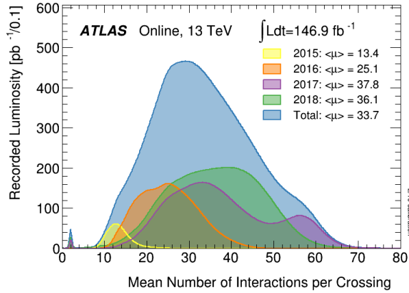
Figure 5.2: Pileup for the Run-2 ATLAS data-taking period.
