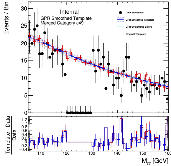
(c) QQ2HQQ_GE2J_MJJ_120_350_1
