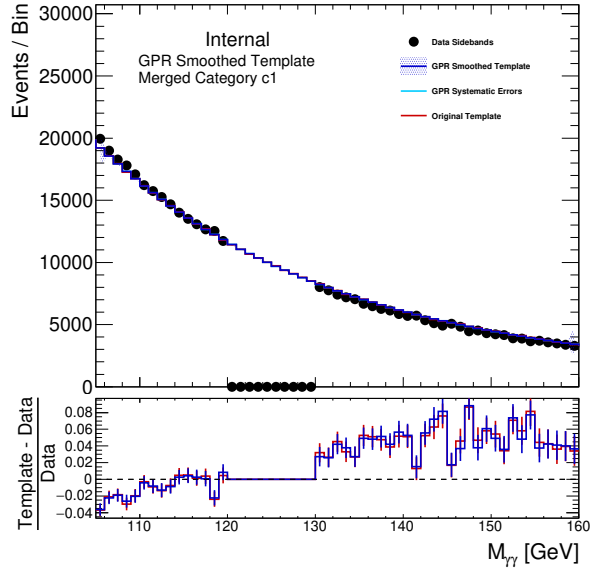
(b) GG2H_0J_PTH_GT10_0
