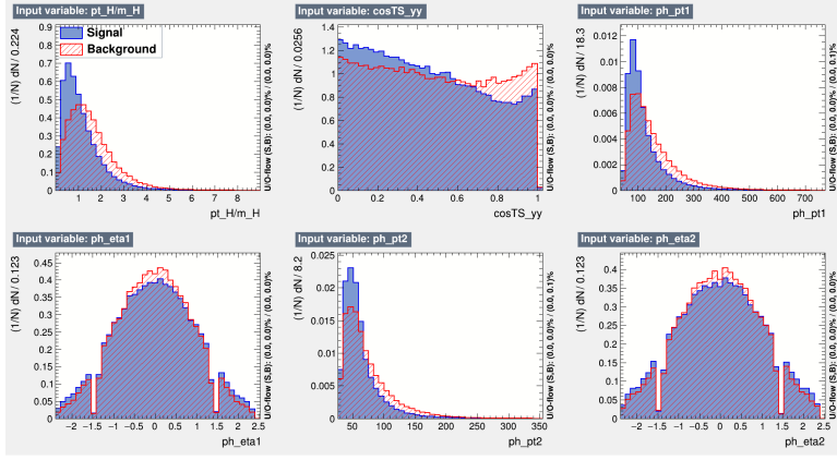
Figure B.2: Normalized training variables for the 4-vector BDT, output by TMVA. CP-odd ttH is denoted as "signal" (blue); CP-even ttH is denoted as "background" (red). Variables shown are, from left to right, top row to bottom row: Higgs candidate p_T (scaled by mass), \cos(\theta^*) , leading photon p_T , leading photon \eta , subleading photon p_T , and subleading photon \eta .
