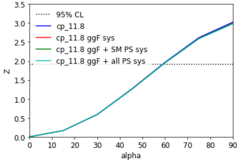
Figure 7.19: The impact of systematic uncertainties on the number counting limit. There is a small change of 0.3^\circ on the number-counting limit, thus indicating that systematics do not appreciably affect the categorization.
