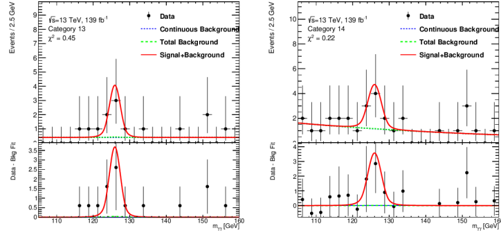
(a) Category 13: m_{\gamma\gamma} (GeV) (b) Category 14: m_{\gamma\gamma} (GeV)
