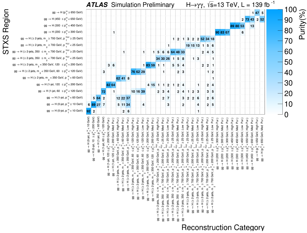
Figure 9.4: The correspondence between analysis category and STXS truth bins, in terms of the percentage contribution of a given STXS truth bin (y-axis) to the Higgs signal yield in a given analysis category (x-axis) for gg \rightarrow H categories and truth bins. Entries with a value below 1% are omitted.
