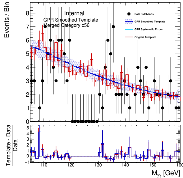
(a) QQ2HQQ_GE2J_MJJ_GT700_PTH_0_200_PTHIJ_0_25...1
