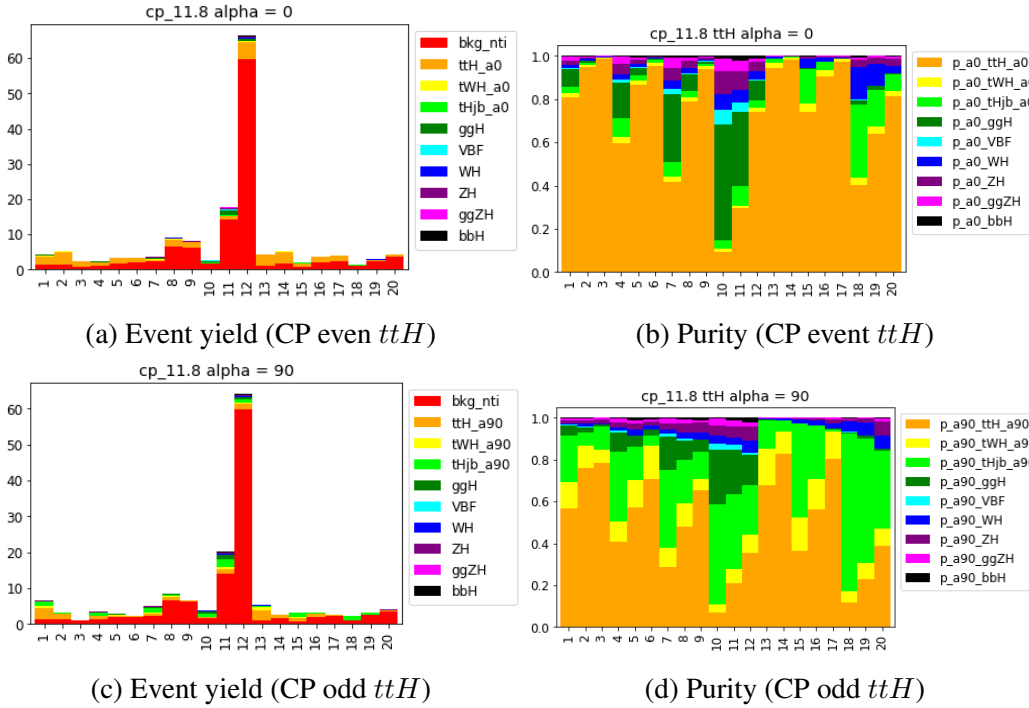
Figure 7.18: (Left) Event yields in the CP categories. Shown separately for \alpha = 0^\circ and \alpha = 90^\circ . (Right) purity of the Higgs yield in each category for \alpha = 0^\circ and \alpha = 90^\circ . Yields are calculated in the signal window m_{\gamma\gamma} = 125 \pm 2 GeV.
