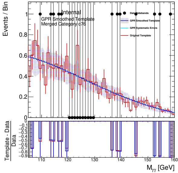
(c) HLL_PTV_150_250_0J_0
