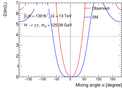
Figure 8.9: One-dimensional likelihood scan over possible values of the CP-mixing angle \alpha on post-fit Asimov data (blue) and observed data (red). ggF and H \rightarrow \gamma\gamma are constrained by the previous Higgs coupling combination result.
