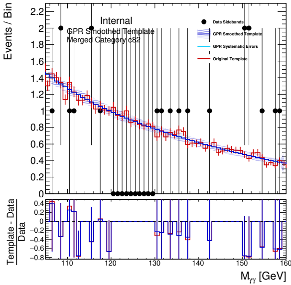
(a) TTH_PTH_60_120_0
