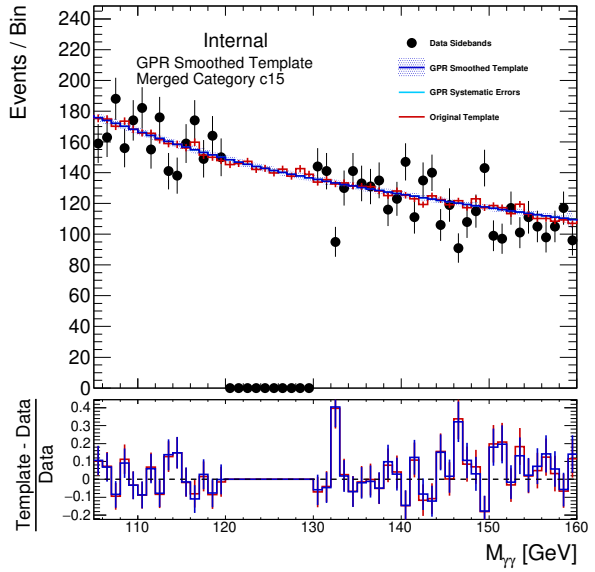
(b) GG2H_GE2J_MJJ_0_350_PTH_120_200_1
