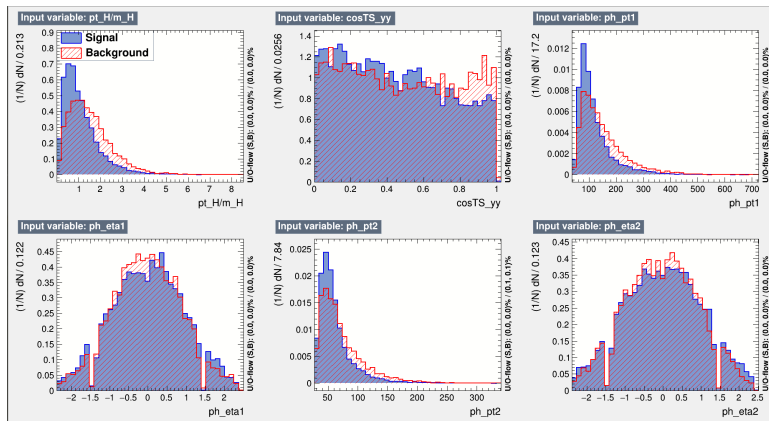
Figure B.18: Normalized training variables for the 4-vector BDT, output by TMVA. CP-odd ttH is denoted as "signal" (blue); CP-even ttH is denoted as "background" (red). Variables shown are, from left to right, top row to bottom row: Higgs candidate p_T (scaled by mass), \cos(\theta^*) , leading photon p_T , leading photon \eta , subleading photon p_T , subleading photon \eta .
