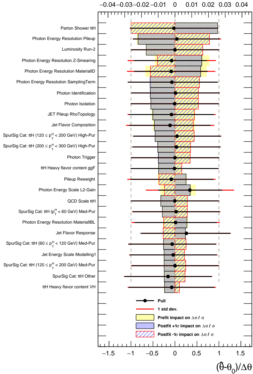
Figure C.6: Nuisance parameter "pull plots" for the ttH+ttH cross-section in the five-production-mode fit. The nuisance parameters are ranked by their impact on the cross-section measurement. These show the pre-fit and post-fit impact of various nuisance parameters on the cross-section measurement (colored and shaded boxes, corresponding to the top x-axis), as well as the "pull" (change in mean and spread between pre- and post-fit nuisance parameters, corresponding to the bottom x-axis).
