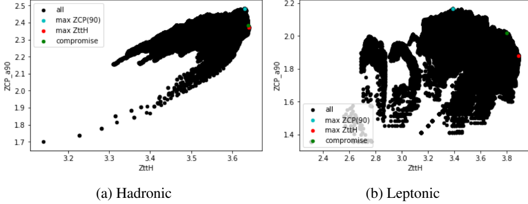
Figure 7.17: Z_{CP} vs. Z_{ttH} for all sets of boundaries considered.
