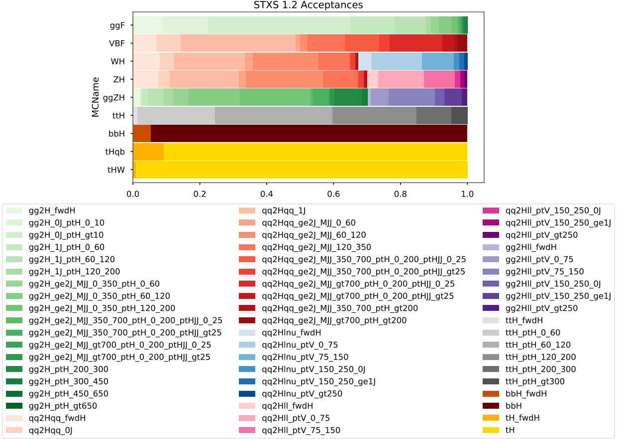
Figure 6.6: Stage 1.2 STXS bin acceptances for all Higgs production modes considered in the Couplings analysis. The FWDH bins target events outside the nominal acceptance, i.e. with |y_H| > 2.5 .
