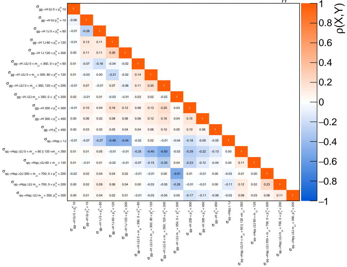
Figure 9.18: The subset of the correlation matrix of the STXS measurements shown in Figure 9.16 corresponding to the gg \rightarrow H and qq' \rightarrow Hqq' STXS regions.
