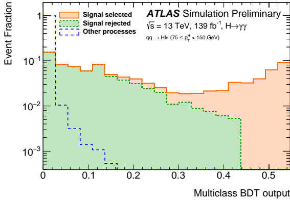
(c) qq \rightarrow H\ell\nu ( 75 \leq p_T^H < 150 GeV)
