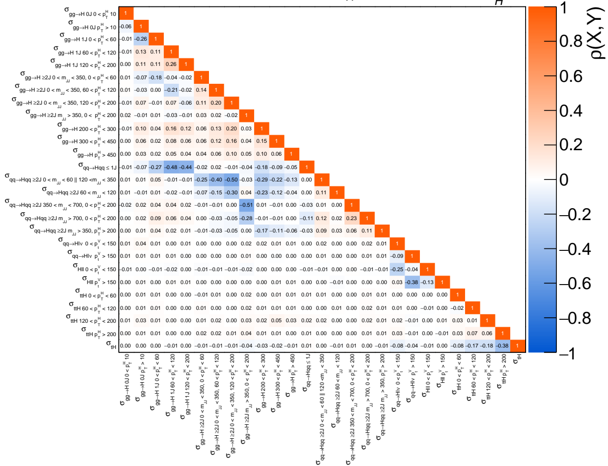
Figure 9.16: Correlation matrix for the full STXS measurement.
