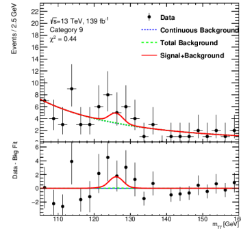
(c) Category 9: m_{\gamma\gamma} (GeV)
