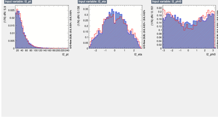
Figure B.21: Normalized training variables for the 4-vector BDT, output by TMVA. CP-odd ttH is denoted as "signal" (blue); CP-even ttH is denoted as "background" (red). Variables shown are, from left to right, top row to bottom row: p_T of subleading lepton, \eta of subleading lepton, \phi of subleading lepton (measured with respect to the Higgs candidate)
