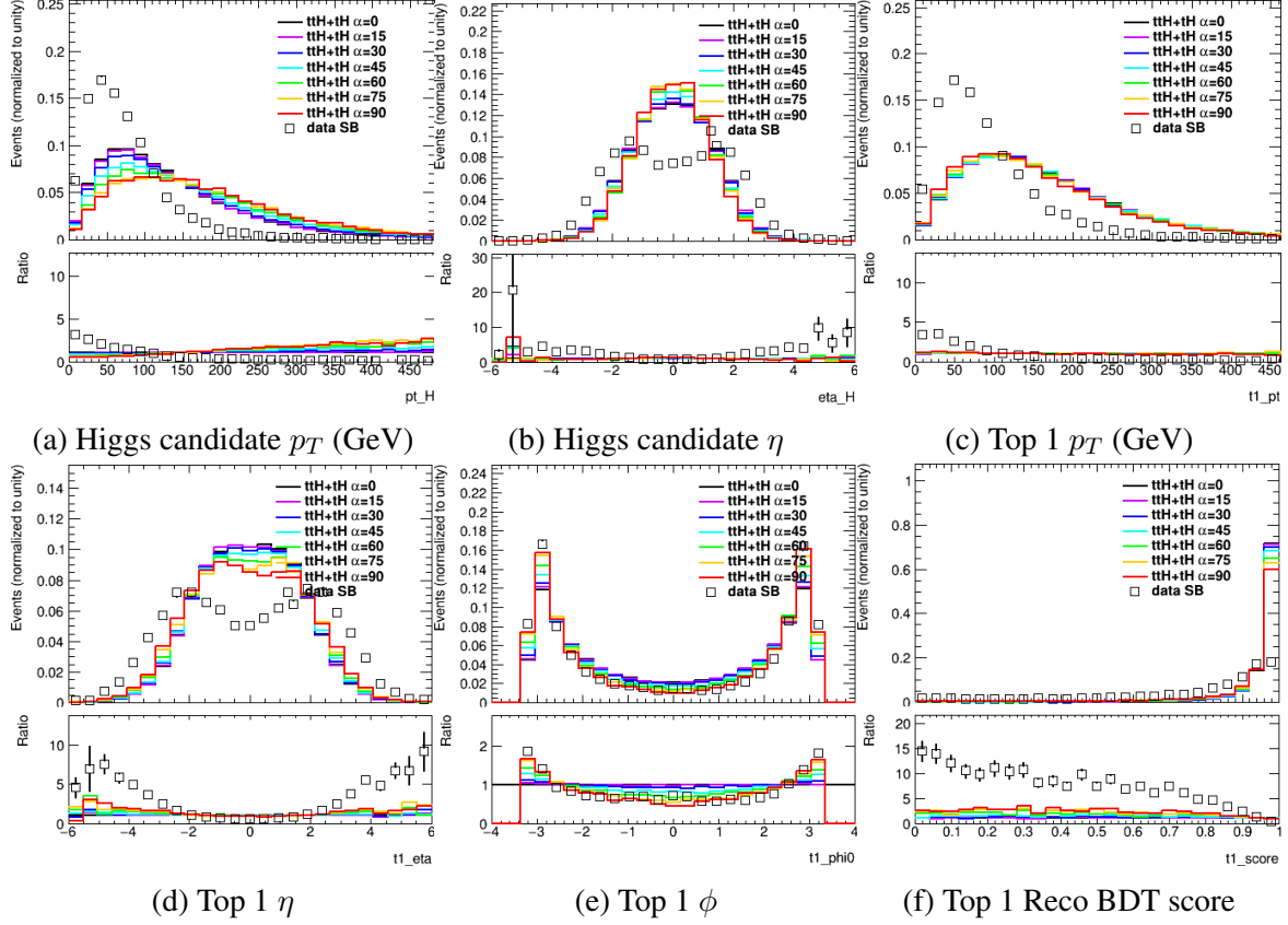
Figure 7.11: Hadronic BDT training variables. The top \phi is calculated with respect to the Higgs candidate. The open squares indicate data in the NTI sideband region, which approximates the shape of the continuum background.
