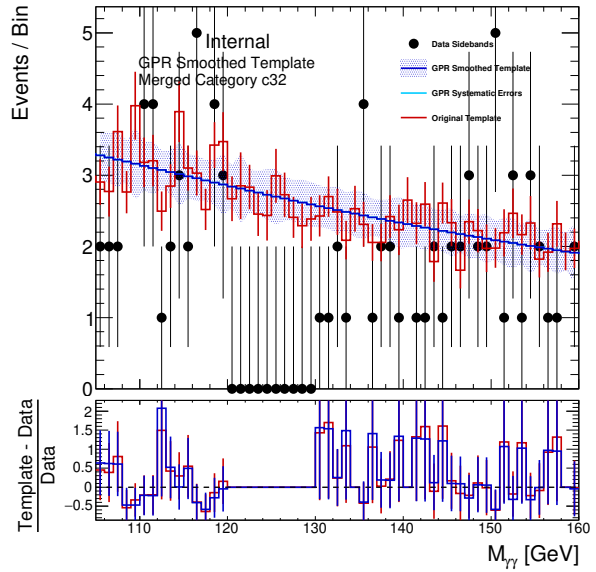
(b) GG2H_PTH_300_450_1
