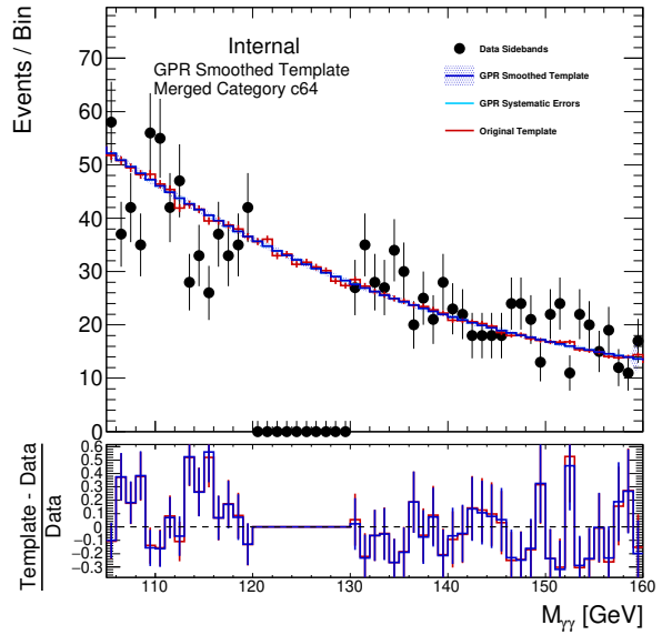
(b) UNSELECTED_WH
