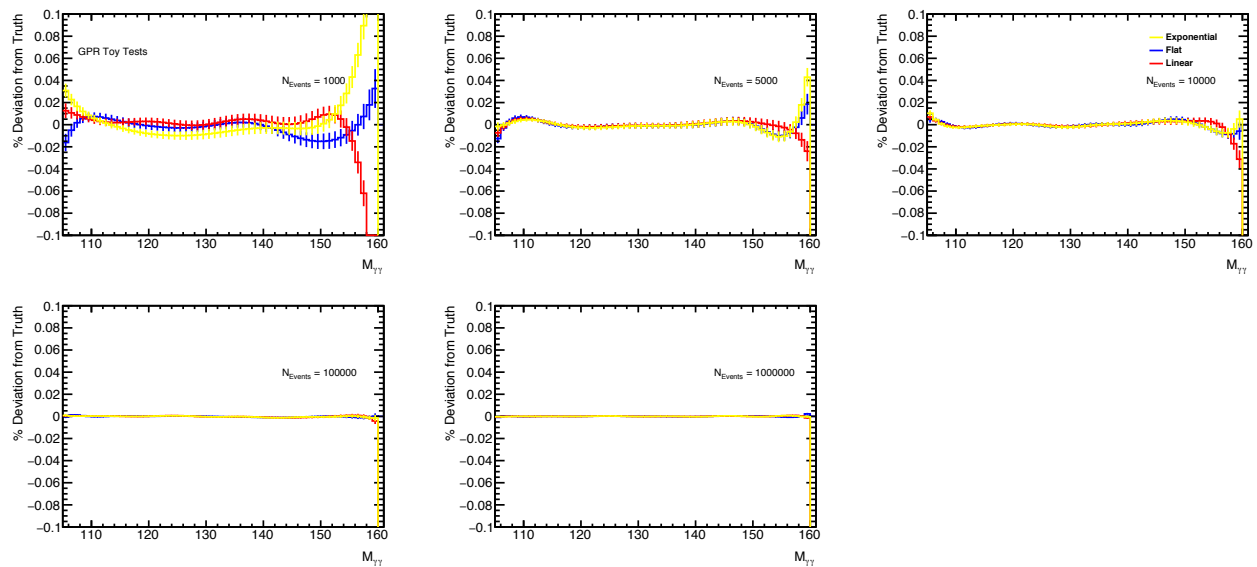
Figure E.10: The per-bin percent deviation of the smoothed template from the unsmoothed template for a variety of different choices of GP mean, using a Bernstein5 function as the toy basis. The yellow shape shows the results using an Exponential mean, the blue shape shows the result uses a flat mean, and the red shape uses a linear mean. Templates contain, from left to right and top to bottom, 1000 events, 5,000 events, 10,000 events, 100,000 events, and one million events.
