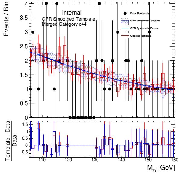
(b) QQ2HQQ_GE2J_MJJ_0_60_1
