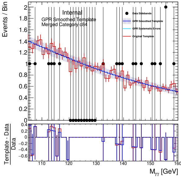
(c) TTH_PTH_120_200_0
