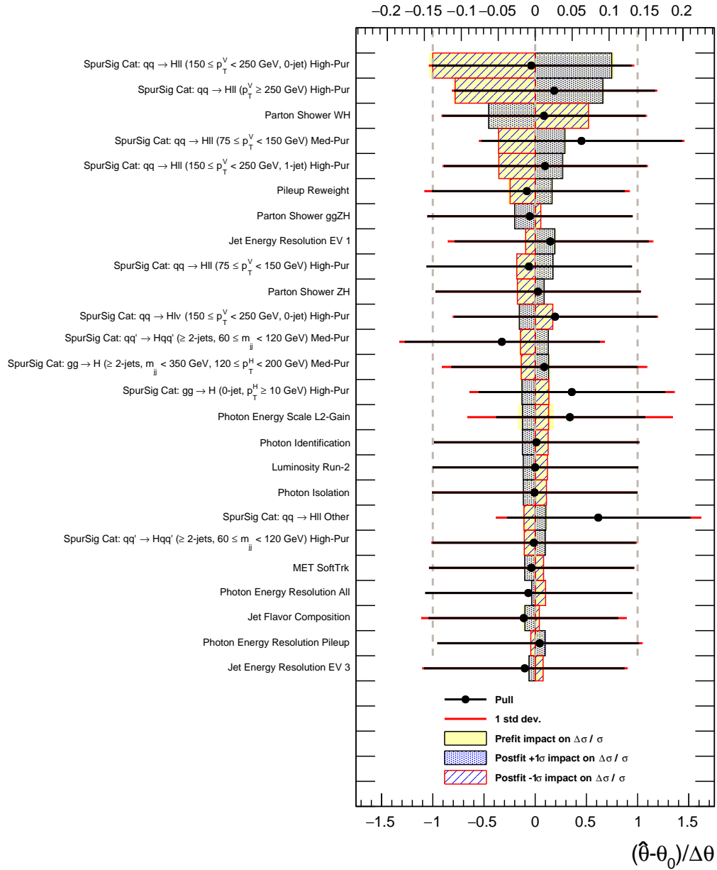
Figure C.5: Nuisance parameter "pull plots" for the ZH cross-section in the five-production-mode fit. The nuisance parameters are ranked by their impact on the cross-section measurement. These show the pre-fit and post-fit impact of various nuisance parameters on the cross-section measurement (colored and shaded boxes, corresponding to the top x-axis), as well as the "pull" (change in mean and spread between pre- and post-fit nuisance parameters, corresponding to the bottom x-axis).
