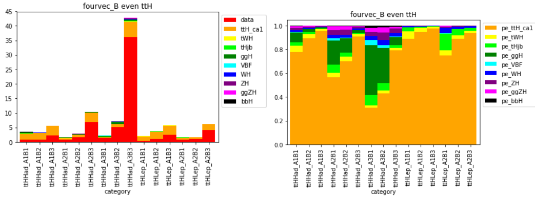
(a) Event yield (CP even ttH )
