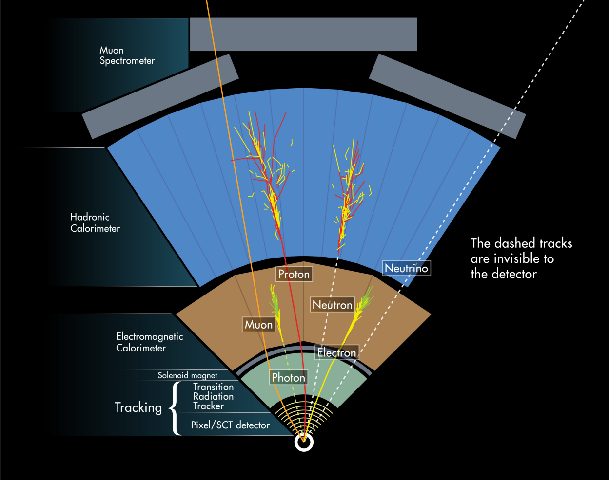
Figure 4.1: Shapes and signatures of a variety of objects in the detector [72]
