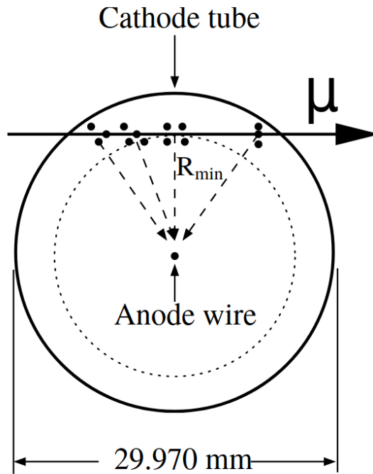
Figure 3.11: A diagram of a Monitored Drift Tube [43]
