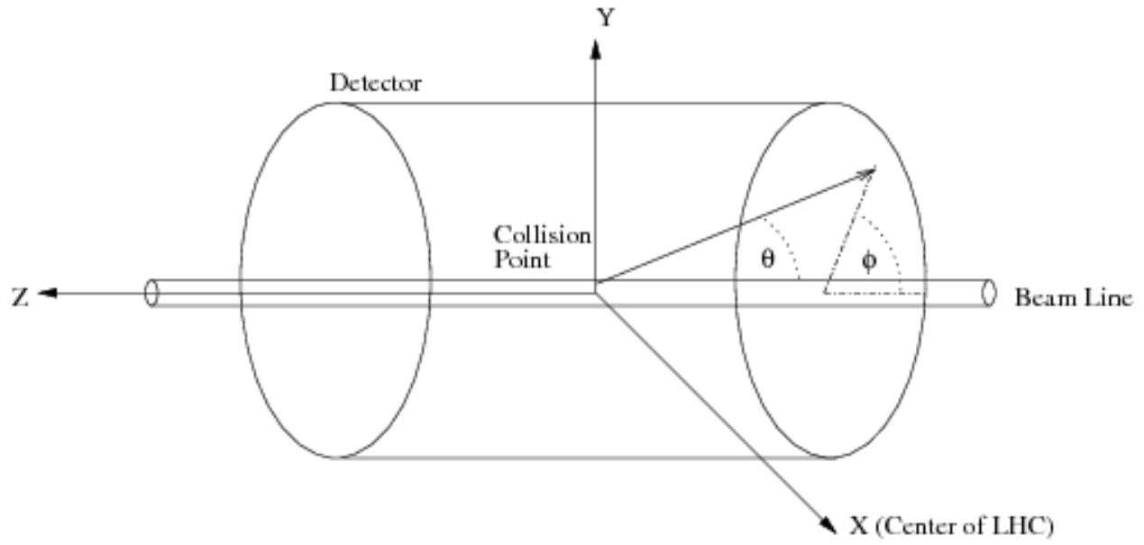
Figure 3.3: The coordinate system used to define the ATLAS detector geometry. [44]
