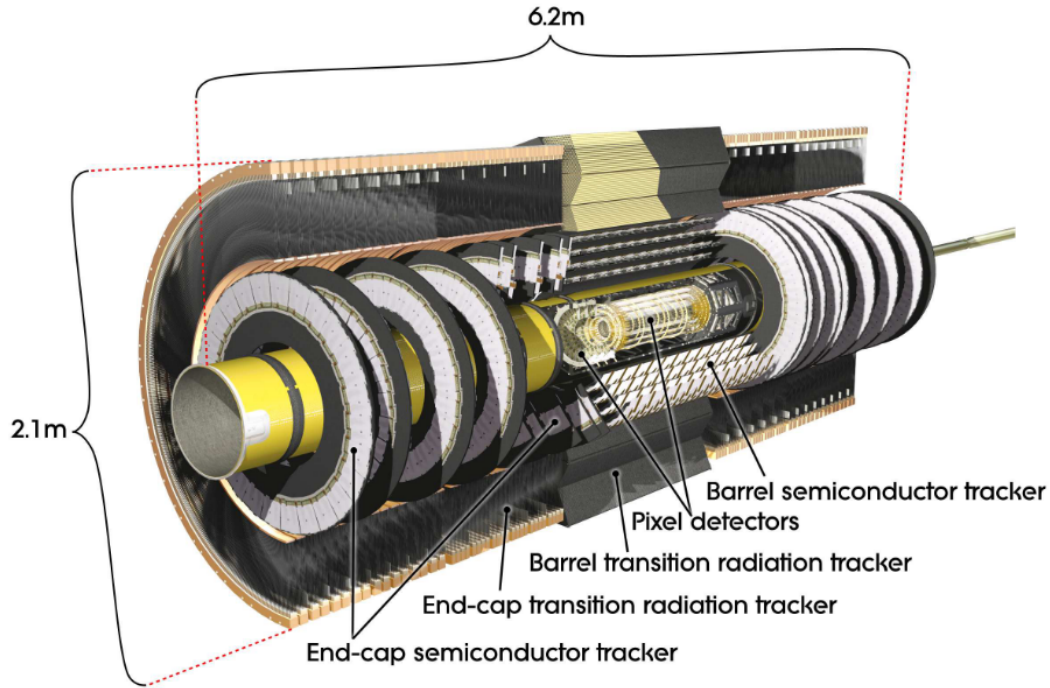
Figure 3.4: An illustration of the Inner Detector. [43]
