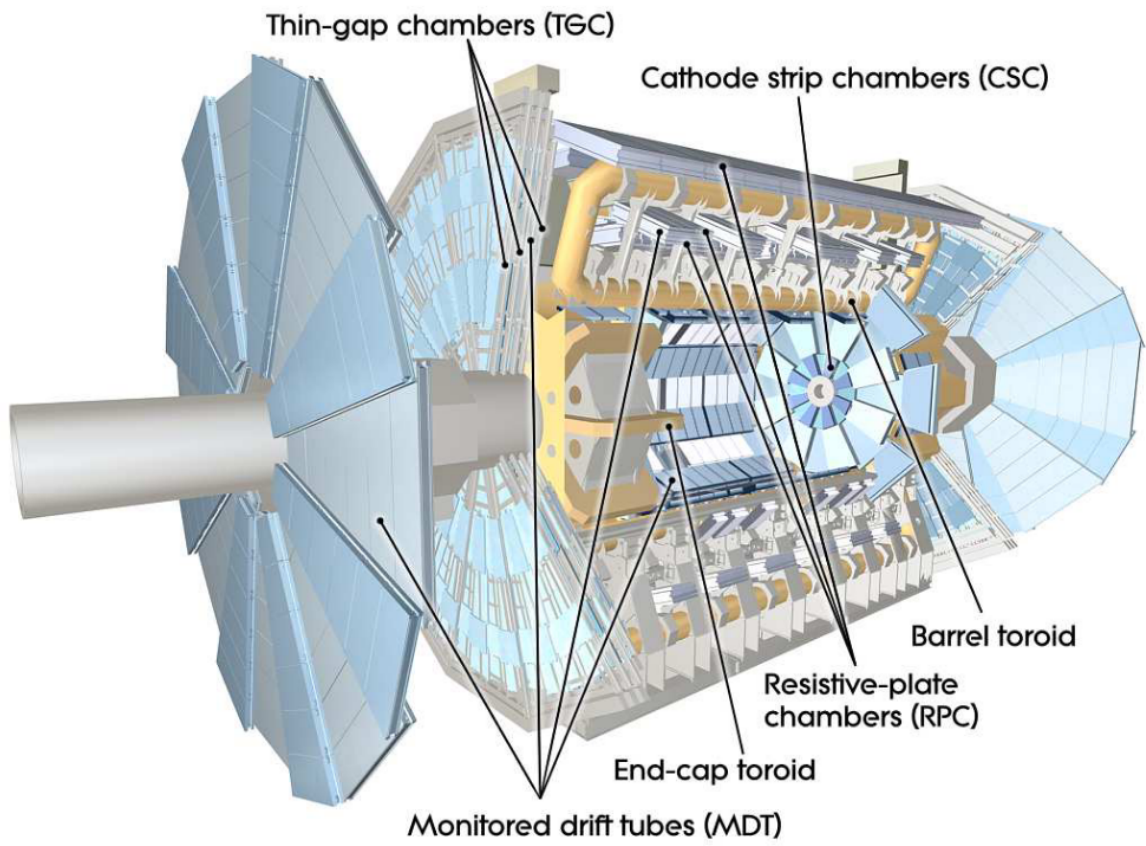
Figure 3.10: A diagram of the Muon System [43]
