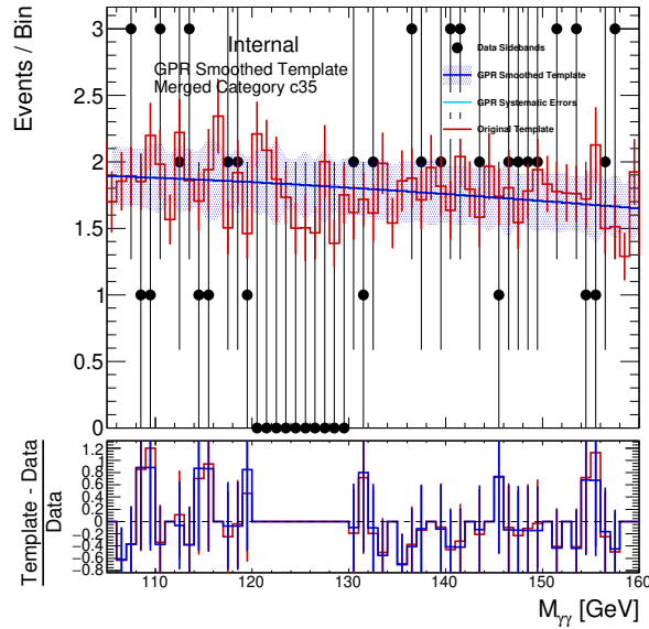
(a) GG2H_PTH_450_650_1
