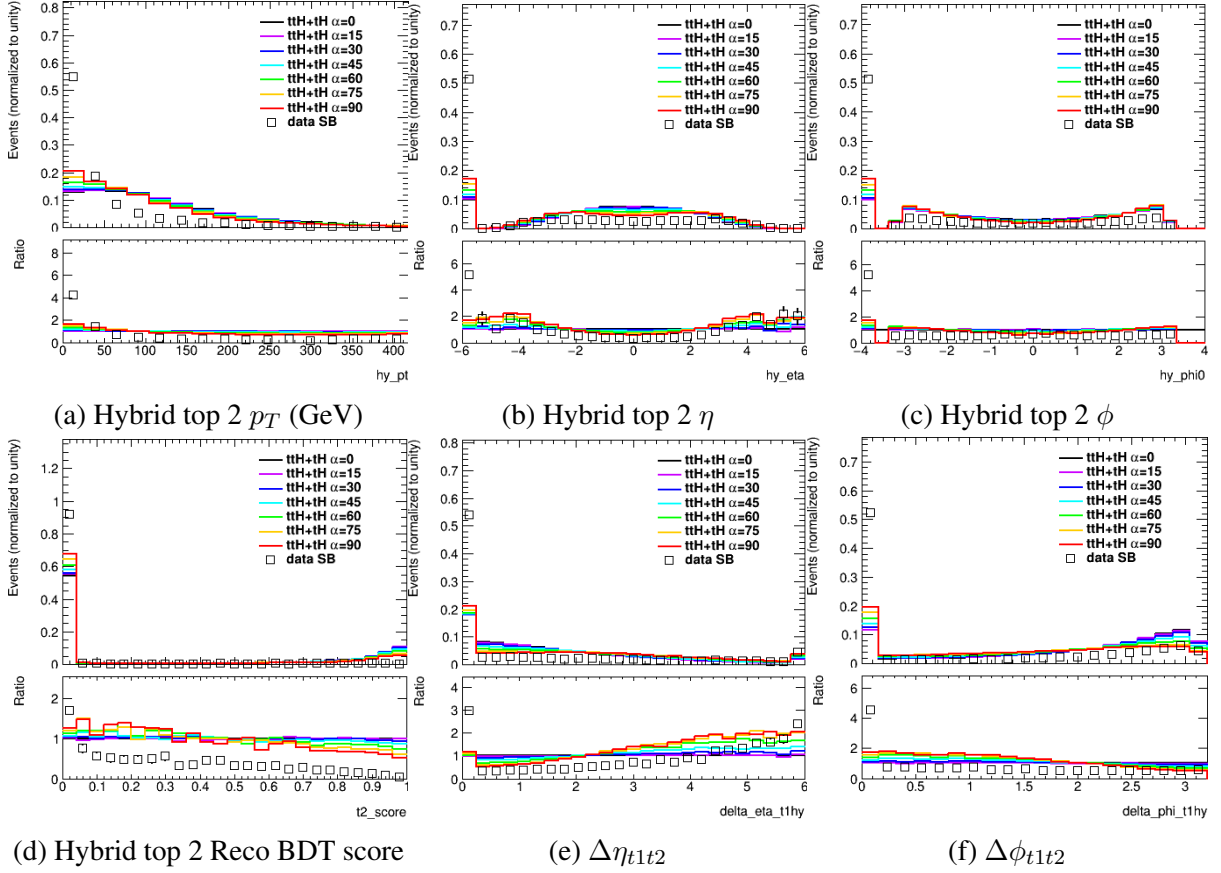
Figure 7.12: Hadronic BDT training variables. The top \phi is calculated with respect to the Higgs candidate. The underflow bins in top p_T/\eta/\phi and \Delta\eta_{t1t2}/\Delta\phi_{t1t2} contain events where no second (‘hybrid’) top is reconstructed, while the underflow bin in the BDT score contains events with fewer than six jets (i.e., events with either no hybrid top or a hybrid top that is reconstructed using the remaining-jets method). The open squares indicate data in the NTI sideband region, which approximates the shape of the continuum background.
