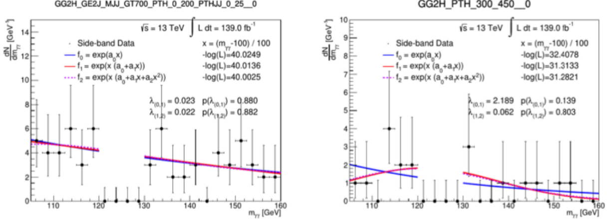
Figure 6.4: An example of the Wald test being performed in two low-statistics Couplings categories. The exponential functional form is chosen in both cases.
