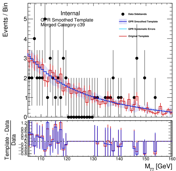
(a) QQ2HQQ_0J__1
