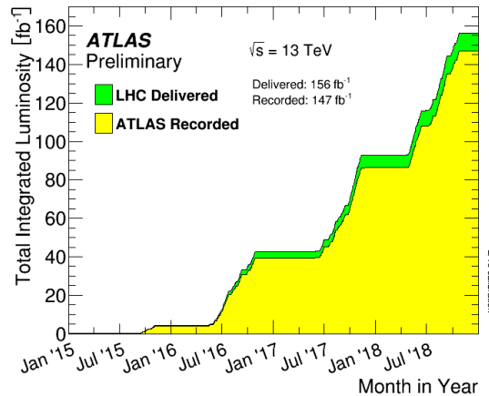
Figure 5.1: Integrated luminosity for the Run-2 ATLAS data-taking period.
