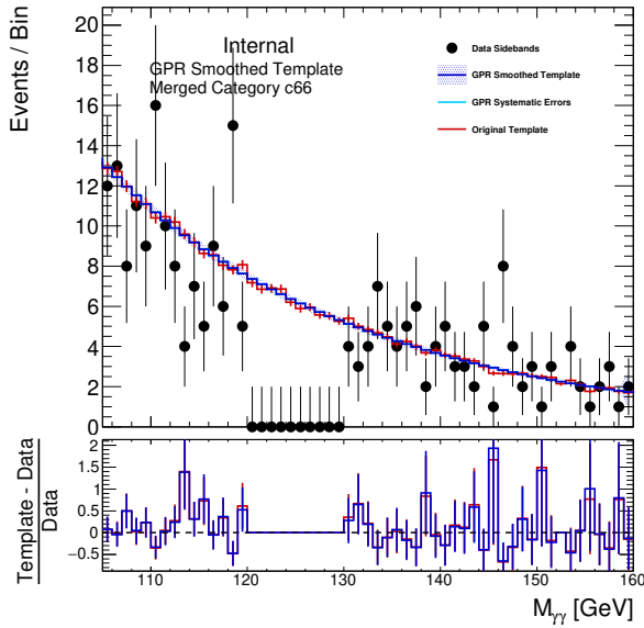
(a) QQ2HLNU_PTV_0_75_1
