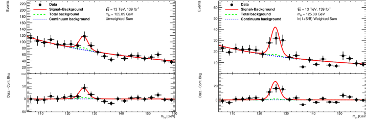
(a) Sum of categories (un-weighted): m_{\gamma\gamma} (GeV) (b) Sum of categories (weighted): m_{\gamma\gamma} (GeV)
