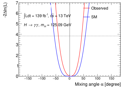
Figure 8.11: One-dimensional likelihood scan over possible values of the CP mixing angle \alpha on post-fit Asimov data (blue) and observed data (red). ggF and H \rightarrow \gamma\gamma are parameterized as functions of \kappa_t and \alpha .
