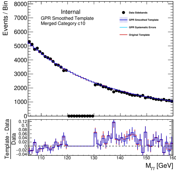
(a) GG2H_GE2J_MJJ_0_350_PTH_0_60_2
