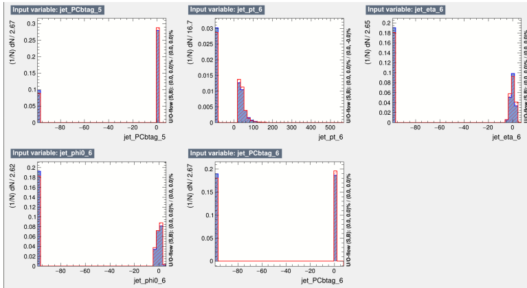
Figure B.7: Normalized training variables for the 4-vector BDT, output by TMVA. CP-odd ttH is denoted as "signal" (blue); CP-even ttH is denoted as "background" (red). Variables shown are, from left to right, top row to bottom row: Pseudo-continuous b-tag score of fifth-highest btag-scoring jet, p_T of sixth-highest b-tag scoring jet, \eta of sixth-highest b-tag scoring jet, \phi of sixth-highest btag-scoring jet (measured with respect to the Higgs candidate), pseudo-continuous b-tag score of sixth-highest btag-scoring jet.
