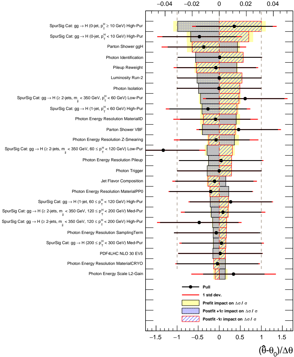
Figure C.2: Nuisance parameter "pull plots" for the ggH cross-section in the five-production-mode fit. The nuisance parameters are ranked by their impact on the cross-section measurement. These show the pre-fit and post-fit impact of various nuisance parameters on the cross-section measurement (colored and shaded boxes, corresponding to the top x-axis), as well as the "pull" (change in mean and spread between pre- and post-fit nuisance parameters, corresponding to the bottom x-axis).
