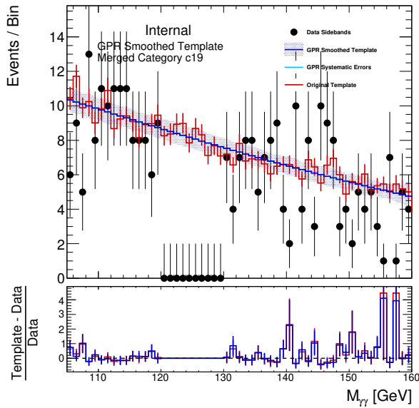
(b) GG2H_GE2J_MJJ_350_700_PTH_0_200_PTHJJ_GT25...0
