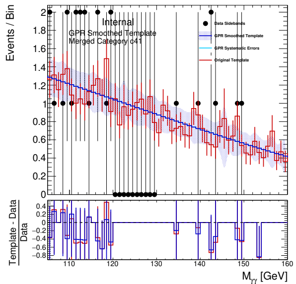
(b) QQ2HQQ_1J__1
