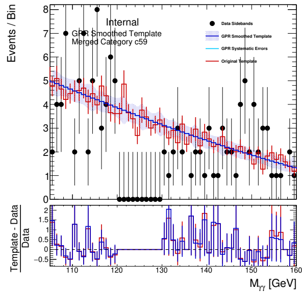
(a) QQ2HQQ_GE2J_MJJ_GT700_PTH.0_200_PTHJJ_GT25...2
