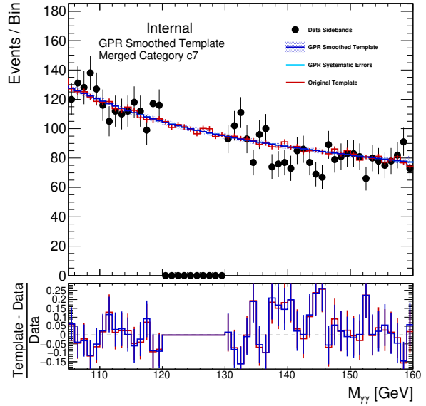
(b) GG2H_1J_PTH_120_200_1
