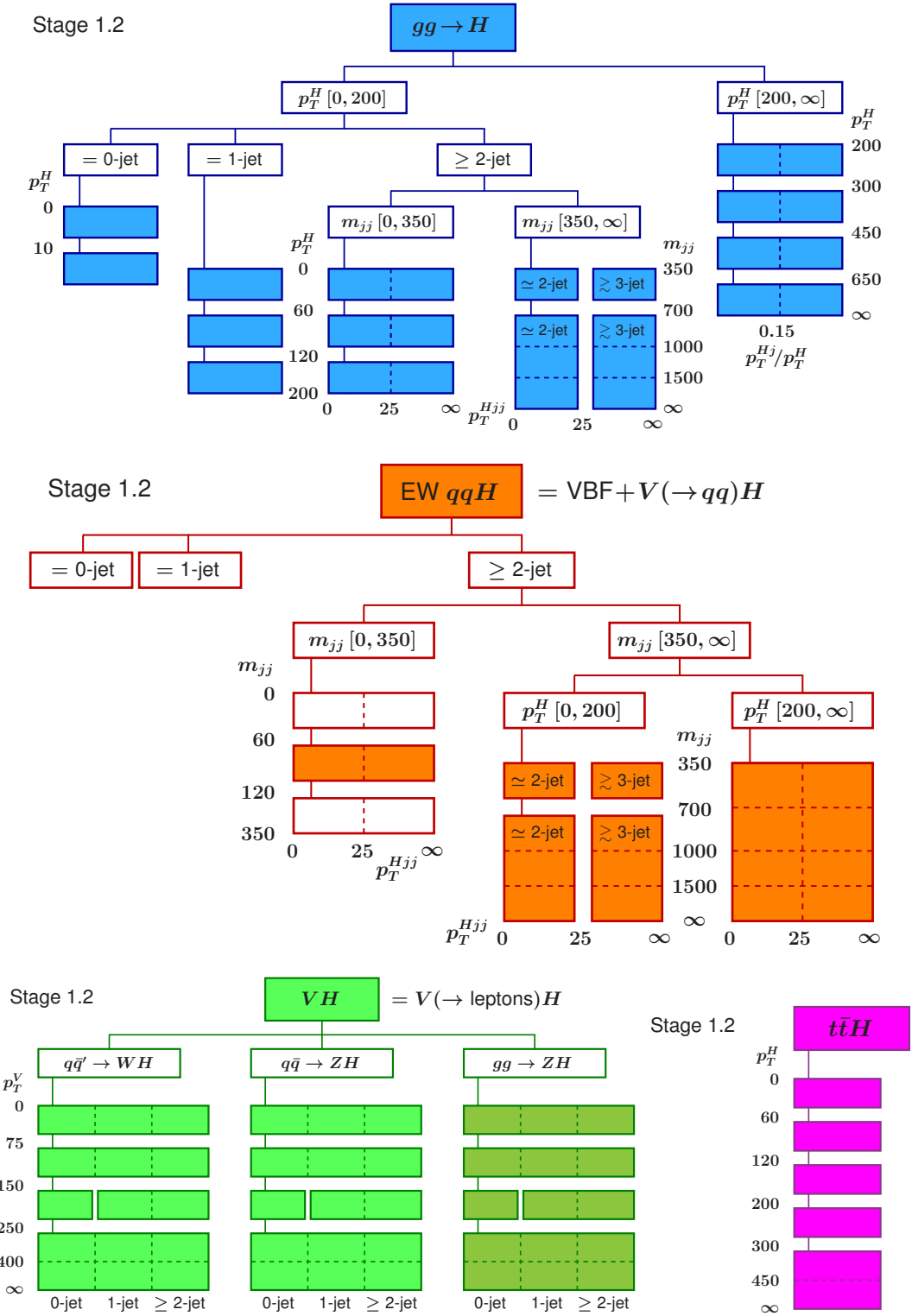
Figure 6.5: Stage 1.2 STXS bin definitions for the main production modes.
