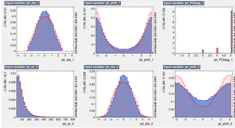
Figure B.4: Normalized training variables for the 4-vector BDT, output by TMVA. CP-odd ttH is denoted as "signal" (blue); CP-even ttH is denoted as "background" (red). Variables shown are, from left to right, top row to bottom row: \eta of highest b-tag scoring jet, \phi of highest btag-scoring jet (measured with respect to the Higgs candidate), pseudo-continuous b-tag score of highest btag-scoring jet, p_T of second-highest b-tag scoring jet, \eta of second-highest b-tag scoring jet, \phi of second-highest btag-scoring jet (measured with respect to the Higgs candidate).
