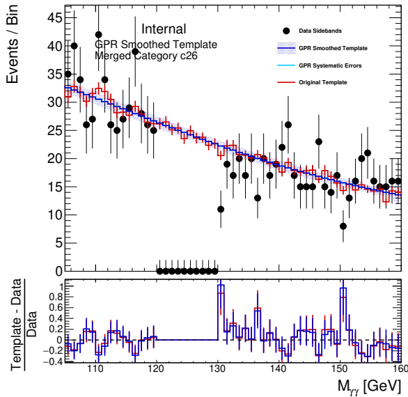
(a) GG2H_GE2J_MJJ_GT700_PTH_0_200_PTHJJ_GT25_1
