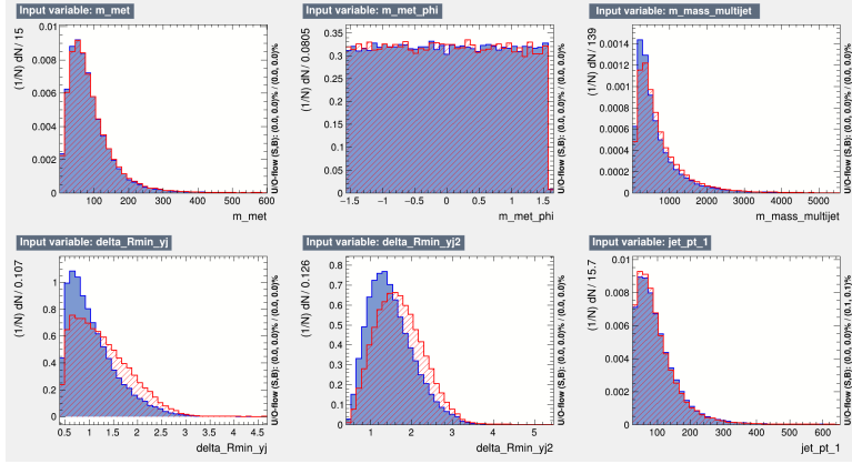
Figure B.10: Normalized training variables for the 4-vector BDT, output by TMVA. CP-odd ttH is denoted as "signal" (blue); CP-even ttH is denoted as "background" (red). Variables shown are, from left to right, top row to bottom row: Magnitude of E_T^{miss} , E_T^{miss} \phi (branch cut chosen to range from -\pi/2 to \pi/2 ), invariant mass of all jets in the event, minimum \Delta R between a photon and a jet, second-smallest \Delta R between a photon and a jet, p_T of highest b-tag scoring jet.
