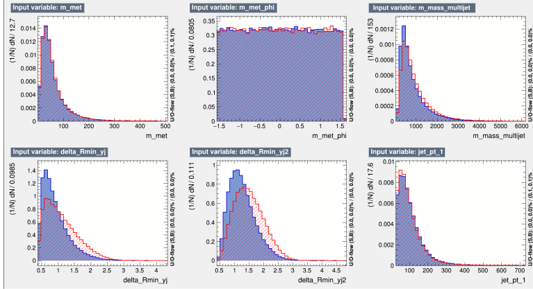
Figure B.3: Normalized training variables for the 4-vector BDT, output by TMVA. CP-odd ttH is denoted as "signal" (blue); CP-even ttH is denoted as "background" (red). Variables shown are, from left to right, top row to bottom row: Magnitude of E_T^{miss} , E_T^{miss} \phi (branch cut chosen to range from -\pi/2 to \pi/2 ), invariant mass of all jets in the event, minimum \Delta R between a photon and a jet, second-smallest \Delta R between a photon and a jet, p_T of highest b-tag scoring jet.
