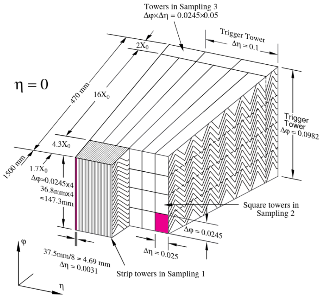
Figure 3.6: A cutaway diagram of the barrel ECAL depicting the “accordion” absorber geometry [43]
