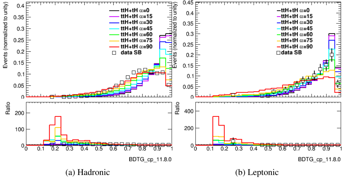
Figure 7.14: Hadronic and Leptonic CP BDT scores for ttH+tHjb+tWH , with relative weights according to their expected cross sections under various CP mixing scenarios. The open squares show data in the NTI sideband region.
