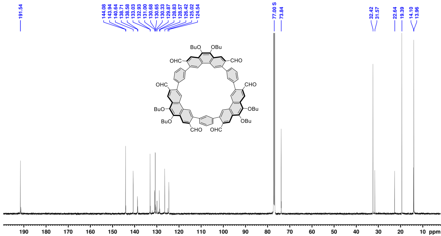
Figure S30. 13 C NMR spectrum of compound 11b (125 MHz, chloroform- d , 300 K).
