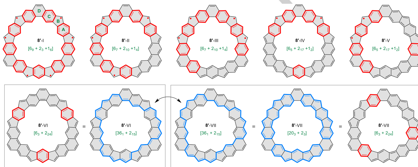
Scheme 3. Selected canonical structures of 8 -I . Formally aromatic and antiaromatic circuits are shown in red and blue, respectively. \pi -Electron partitioning (green labels) corresponds to the highlighted circuits.
