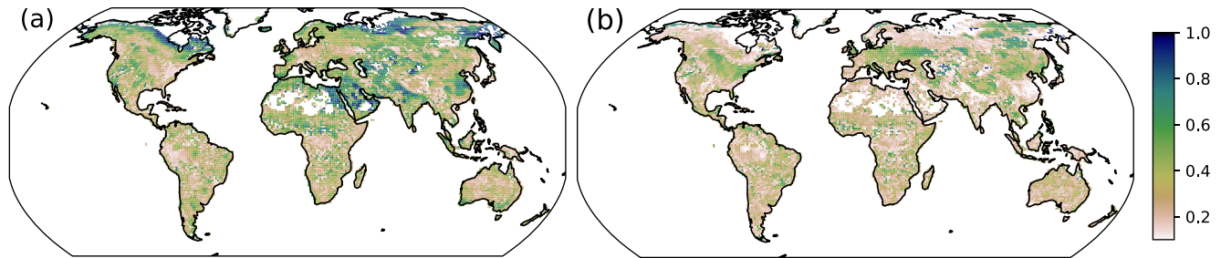
Figure 4. Fraction of variance in detrended net ecosystem production (NEP) anomalies that was explained by (a) seasonal amplification or (b) seasonal redistribution vectors. Globally, these two vectors explained 39% and 29% of the variance in monthly NEP anomalies, respectively.
