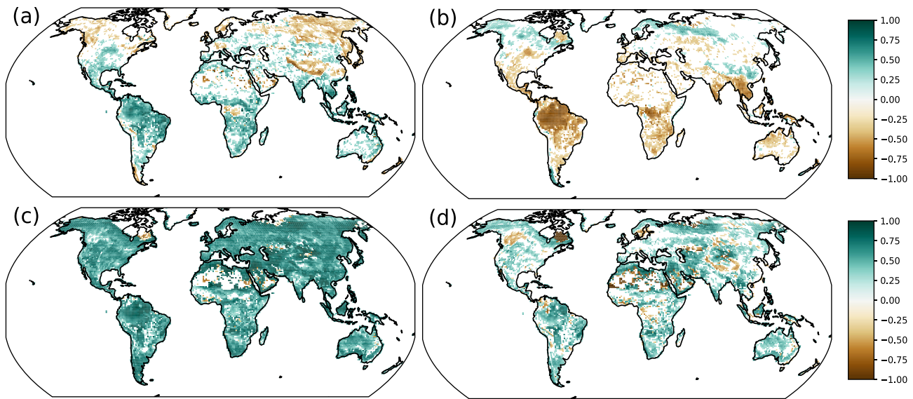
Figure 3. Correlation coefficients between detrended annual anomalies that are simulated by CESM2-esm from 1960 to 2014. Panels show the correlation between net ecosystem production (NEP) and (a) terrestrial water storage, (b) air temperature, (c) gross primary productivity (GPP), and (d) R_{eco} . Only statistically significant correlations ( p < 0.05 , when |r| > 0.226 for 55 years of data) are shown.
