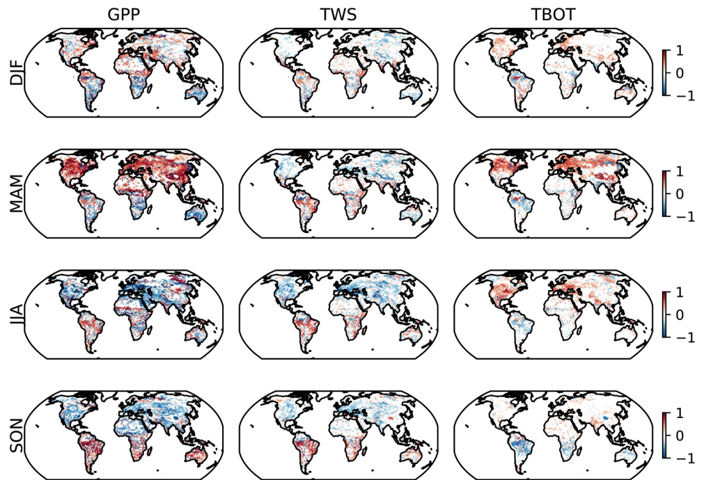
Figure 8. Pearson correlation coefficients between singular value decomposition (SVD) weights from the redistribution vector with seasonal anomalies of gross primary productivity (GPP), terrestrial water storage (TWS), and air temperature (TBOT) simulated by CESM2-esm from 1960 to 2014. Only statistically significant ( p < 0.05 ) correlations are shown ( |r| > 0.26 , two-tailed test, n = 55 ).
