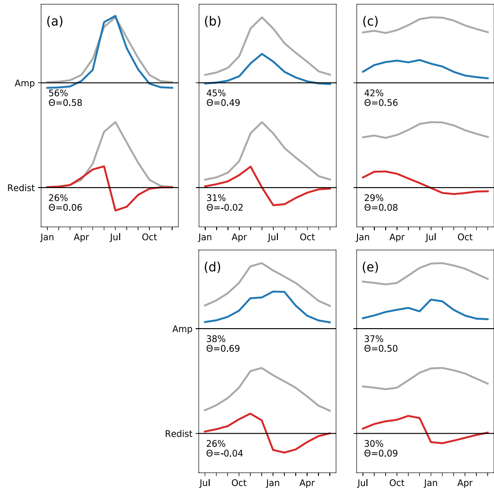
Figure 6. Zonal mean climatology of monthly gross primary productivity (GPP) and singular vectors associated with seasonal amplification and temporal redistribution of GPP (gray, blue, and red lines respectively) for the northern hemisphere and southern hemisphere (top and bottom rows, respectively). Panels organized as in Figure 5. Note x -axis was shifted for southern hemisphere plots to show the climatology for austral summer.
