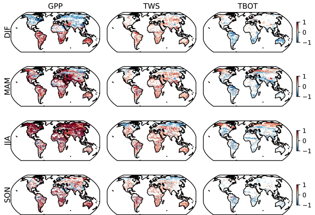
Figure 7. Pearson correlation coefficients between singular value decomposition (SVD) weights from the amplification vector with seasonal anomalies of gross primary productivity (GPP), terrestrial water storage (TWS), and air temperature (TBOT) simulated by CESM2-esm from 1960 to 2014. Only statistically significant ( p < 0.05 ) correlations are shown ( |r| > 0.26 , two-tailed test, n = 55 ).
