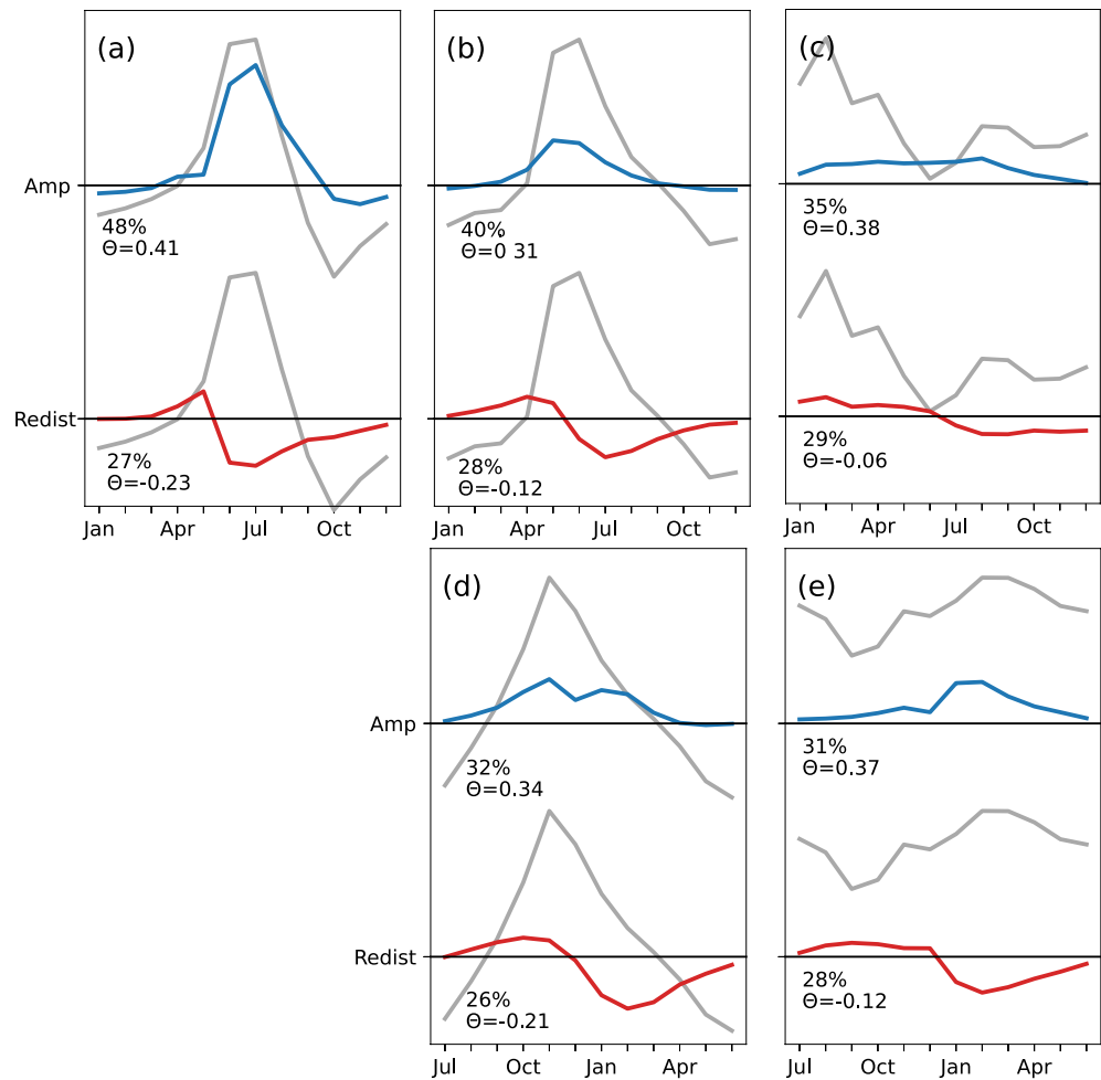
Figure 5. Zonal mean climatology of monthly net ecosystem production (NEP) and singular vectors associated with seasonal amplification and temporal redistribution of NEP (gray, blue, and red lines respectively) for the northern hemisphere and southern hemisphere (top and bottom rows, respectively). Panels show: (a) high latitude ecosystems, 50°–80°N; (b), (d) northern and southern temperate mid latitudes, 20°–50°N and 20°–50°S; and the (c), (e) tropics, 0°–20°N and 0°–20°S, respectively. The magnitude of the singular vectors is arbitrary (y-axis). Mean fraction of variance explained and \theta values, which indicate the net impact on the integrated seasonal signal of NEP for each singular vector, are also provided. Note x-axis was shifted for southern hemisphere plots to show the climatology for austral summer.
