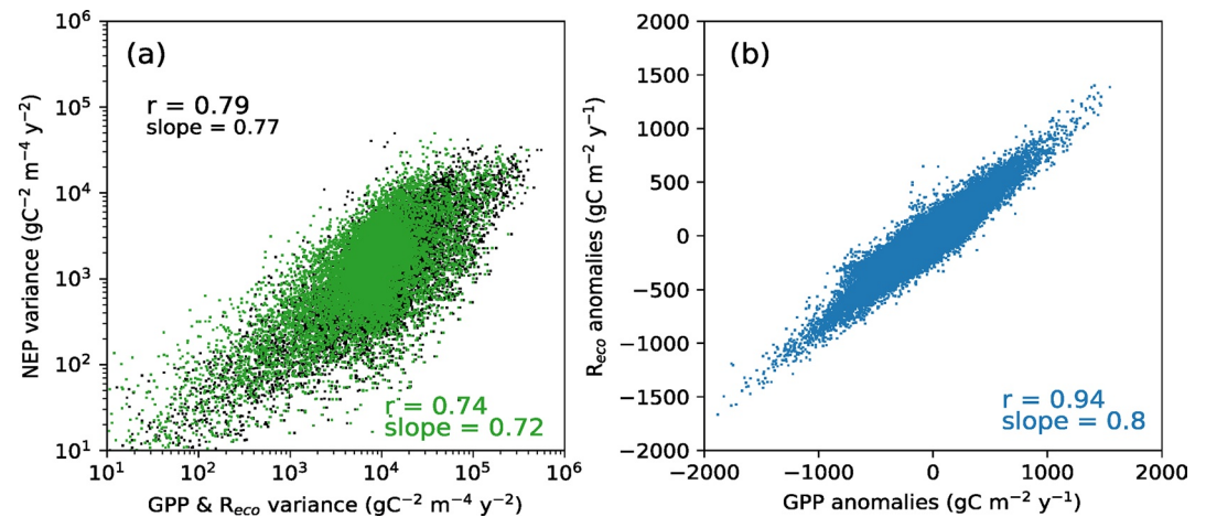
Figure 2. Correlations of grid cell carbon fluxes simulated by CESM2-esm from 1960 to 2015: (a) Variance in net ecosystem production (NEP) versus gross primary productivity (GPP) and R_{eco} (shown in black and green, respectively); and (b) Correlation of anomalies in R_{eco} and GPP. Pearson correlation coefficients and regression slopes from each relationship are provided in each panel, all correlations are significant ( p < 0.001 ).
