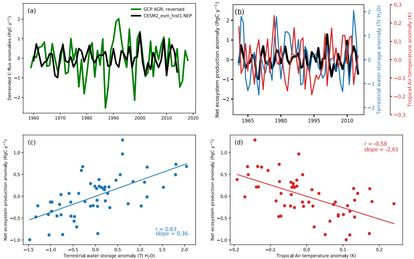
Figure 1. Detrended annual anomalies of global carbon fluxes, climate drivers, and their correlation. Upper panels show: (a) Atmospheric CO 2 growth rate reported by the global carbon project (Friedlingstein et al., 2019) and net ecosystem production (NEP) simulated CESM2-esm (green and black lines, respectively); (b) NEP, terrestrial water storage (TWS), and tropical air temperature anomalies simulated by CESM2-esm (black, blue, and red lines respectively). Lower panels show correlations between simulated: (c) TWS, which is positively correlated to simulated NEP anomalies; and (d) Tropical air temperature, which is negatively correlated to simulated NEP anomalies. Note, for convenience we inverted the sign of the atmospheric growth rate in (a) so that positive anomalies in C fluxes show net land C uptake for both the model and observations.
