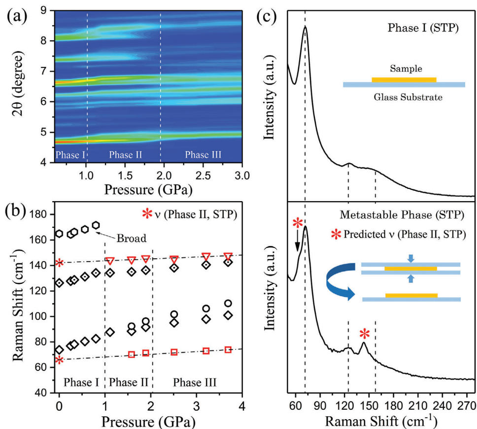
Figure 7. a) Expanded region of the 2D X-ray diffraction map between 0.6 and 3 GPa showing a new phase that covers the region between 1 and 2 GPa. b) The pressure-dependent Raman peak positions with dot-dashed lines giving predicted positions at standard temperature and pressure (STP) from linear extrapolation of the phase II peaks, indicated with * symbols. In the top panel of (c), the Raman spectrum of the original sample is shown while the spectrum of a sample after compression between glass slides is given in the bottom panel. The appearance of additional peaks is indicated by the * symbols. Compression between the glass slides brings the samples into phase II and a part of the sample is maintained in this phase after release of pressure (metastable phase II).
