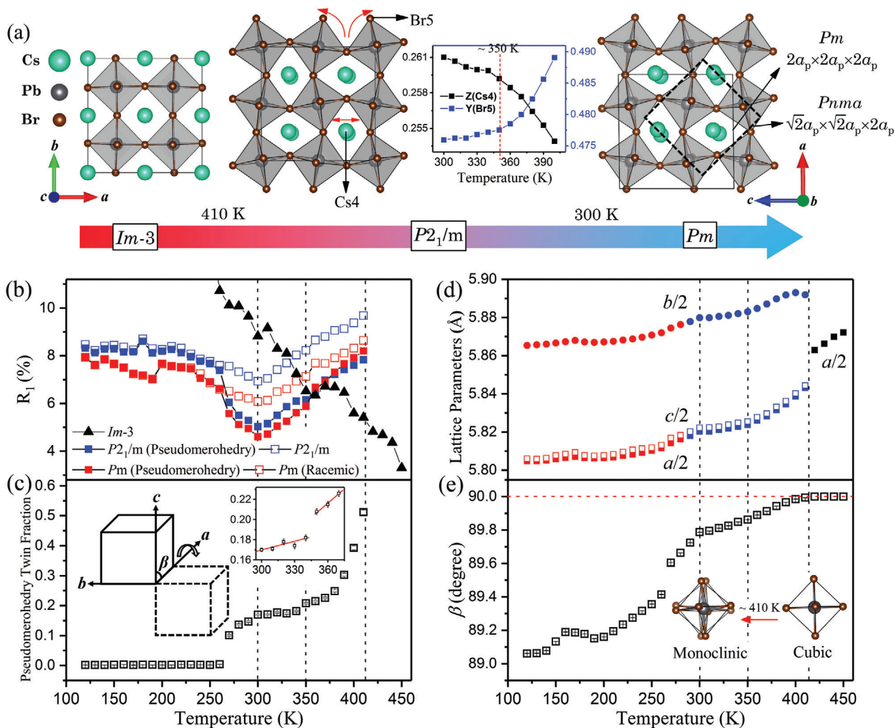
Figure 2. a) The temperature-dependent structure of CsPbBr 3 from single-crystal synchrotron X-ray diffraction measurements. Above 410 K, the space group is cubic Im \bar{3} . Between 410 and 300 K, the structure is monoclinic P2 1 / m . The inset shows the Z fractional coordinate of Cs4 and the Y fractional coordinate of Br5 as a function of temperature. An isostructural phase transition is observed at 350 K. Below 300 K, the space group is Pm . The Pm and previously reported Pnma unit cells are given as the solid and dotted lines, respectively. b) The quality-of-fit parameter, R 1 , of Pm , P2 1 / m , and I - \bar{3}m structures. The solid squares indicate the R 1 parameters which incorporate a pseudomerohedry twin law matrix (1 0 0, 0 -1 0, 0 0 -1), while the open squares are the R 1 parameters of racemic twinning for Pm structure and no twinning for P2 1 / m structure. The temperature-dependent pseudomerohedry twin domain fraction is shown in (c). The single-crystal diffraction derived lattice parameters as a function of temperature are given in (d) and (e).
