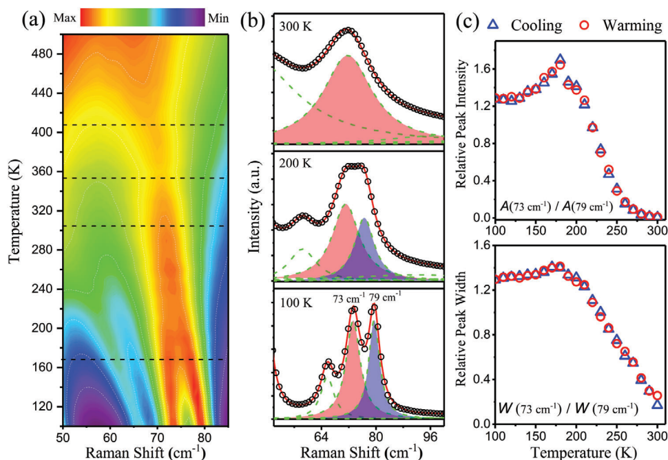
Figure 1. a) Contour plot of the temperature dependence of the Raman spectra. b) Low energy region of Raman spectra fitted by a sum of Lorentzian functions. The black open circles give the experimental data, the solid red line represents the sum of the fitting functions, and the dashed lines show the individual fitting components. A double-peak structure is shown, which is shaded in red and blue, for the modes at 73 and 79 \text{cm}^{-1} , respectively. The ratio of fitted peak area and peak width are shown in panel (c), indicating a phase transitions onset near 170 and 300 K.
