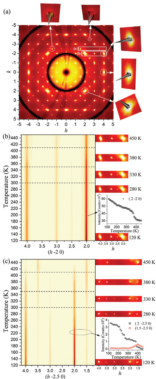
Figure 3. a) Single-crystal X-ray diffraction reciprocal lattice image of the (hk0) plane at 450 K. The (hkl) grid corresponds to the previously reported Pm\bar{3}m space group with lattice-constant a_p \approx 5.87 Å. The insets show the 3D intensity of some selected reflections with an asymmetric diffuse scattering background. Diffraction spots with half-integer h and k values are observed, indicating the correct lattice constant should be doubled. The temperature-dependent intensity of (h-2, 0) and (h-2.5, 0) reflections are given in panels (b) and (c), respectively, which are the selected regions shown in panel (a).
