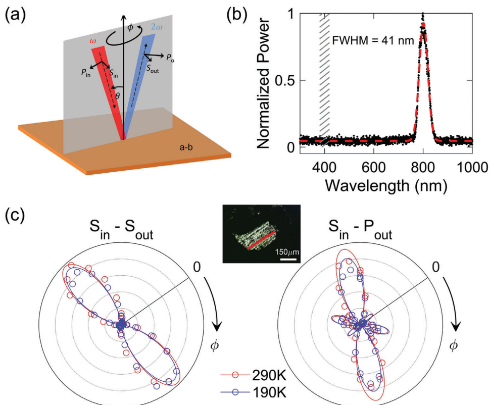
Figure 4. a) Diagram of the RA-SHG setup. The fundamental beam is focused on the ab plane of the crystal with a fixed small incident angle \theta . The scattering plane rotates about the surface normal by an angle \phi . b) The spectrum of the incident fundamental light, centered at 800 nm with a FWHM of 41 nm. The shaded area at 400 \pm 20 nm represents the bandpass region of the filter used to only collect SHG signals. c) The RA-SHG patterns in S_{in} - S_{out} and S_{in} - P_{out} channels under 190 K (blue) and 290 K (red). \phi = 0 represents the direction of a natural edge of the sample. SHG barely shows any difference between data sets at these two temperatures. Inset: the picture of a measured CsPbBr 3 sample. The red bar marks its natural edge.
