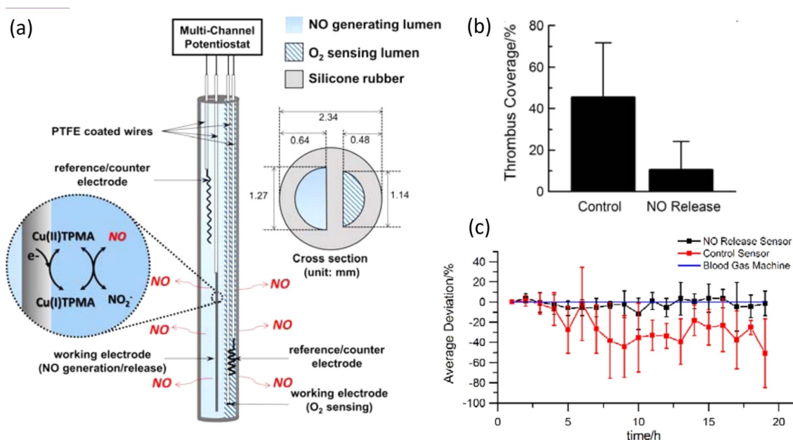
Fig. 3. (a) Cross-sectional schematic view of dual-lumen catheter-type amperometric NO generating/releasing PO_2 sensor; (b) degree of thrombus coverage of control and NO releasing PO_2 sensors after implantation in sheep veins/arteries for 18 h; (c) the comparison of relative deviation in measuring oxygen levels in blood using electrochemical NO releasing sensors (black square) and a control sensors (NO release not turned on) (red square) implanted in pig arteries for 19 h benchmarked to in vitro test values (blue line). (Adapted from [130] with permission; copyright 2015, the American Chemical Society).
