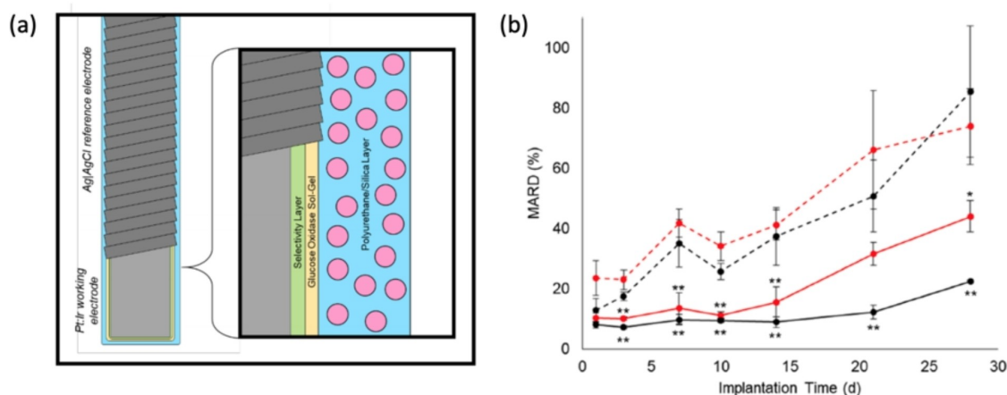
Fig. 6. (a) Schematic of needle-type NO releasing electrochemical glucose biosensor, modified to store NO by doping NO releasing silica nanoparticles into the outermost, glucose flux-limiting polyurethane layer; (b) Comparison of MARD for the sensors measured percutaneously using a diabetic swine model, with 14 d (red) and 30 d (black) NO releasing (solid) vs. the corresponding control (dashed) sensor membranes. Statistical significance from control at a given time point is denoted by asterisks (* p < 0.05 ; ** p < 0.01 ). (Reproduced from [145] with permission; copyright 2019, the American Chemical Society).
