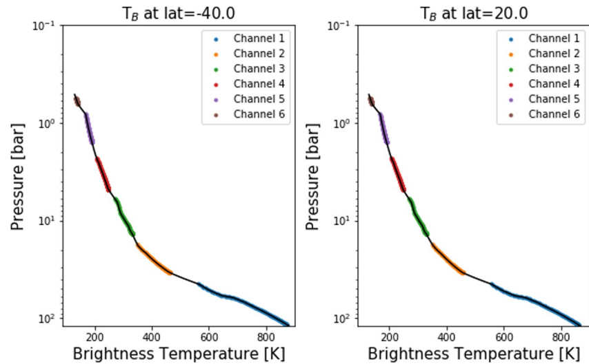
Figure 7. Vertical profiles of T_B at two different latitudes, estimated by assigning limb-darkened microwave radiometer (MWR) measurements to discrete pressure levels using the contribution function peaks in Figure 6. The y-axis indicates the pressure of the contribution peak at different emission angles, and different colors indicate different channels, with a smooth interpolation over regions without MWR sensitivity (retaining emission angles smaller than 70^\circ ). Note that this is not from a spectral inversion, therefore does not represent kinetic temperatures—it is simply a reprojection of the MWR measurements.
