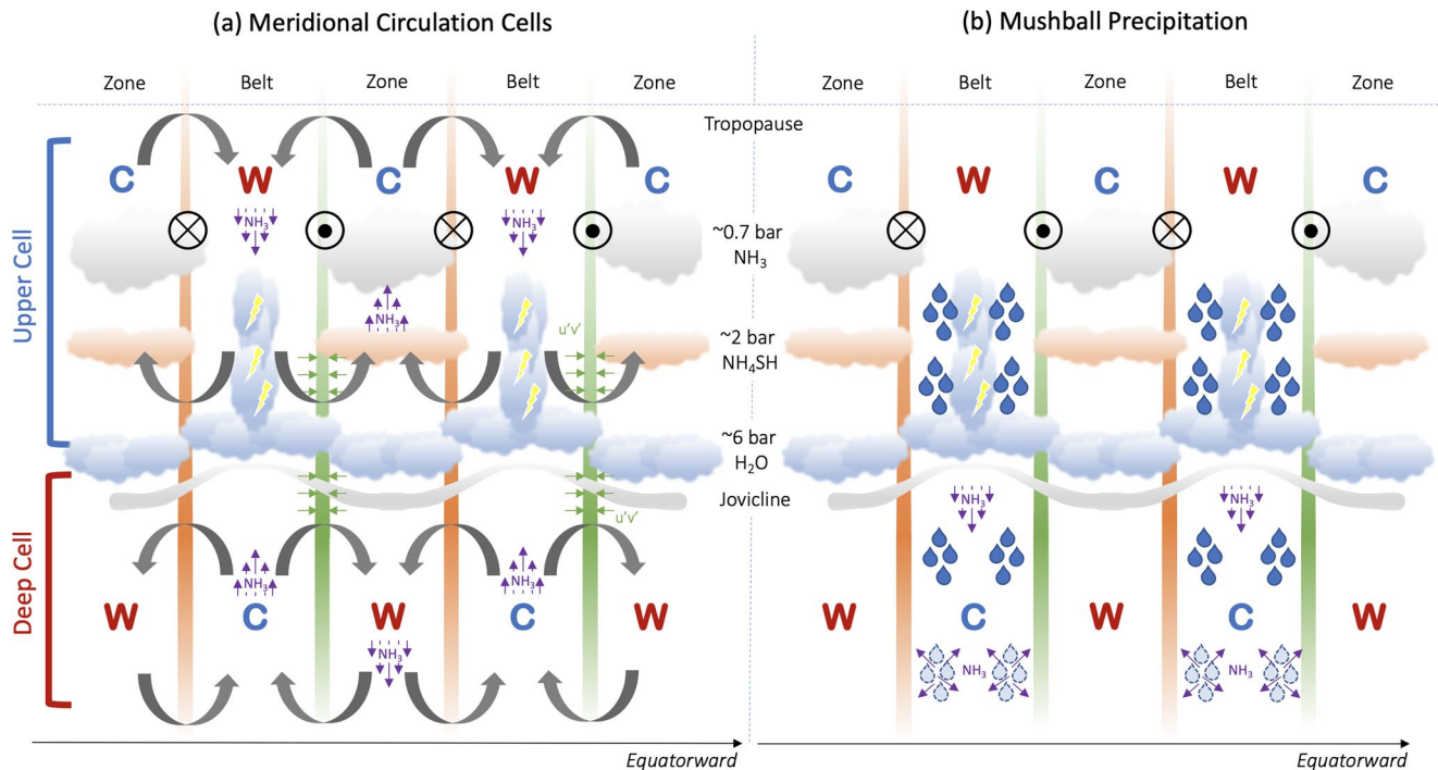
Figure 12. Conceptual diagrams of (a) the stacked system of meridional cells (adapted from Fletcher et al., 2020; Showman & de Pater, 2005), and (b) mushball precipitation (Guillot, Li, et al., 2020). We stress that reality is likely to combine both of these concepts, and all altitudes are qualitative. In both diagrams, high microwave brightness is denoted by a red “W” (warm), low microwave brightness is denoted by a blue “C” (cool); storm plumes are indicated as rising clouds with lightning flashes. The equator is to the right, such that belts have prograde jets on their equatorward edges. Eastward prograde jets are green (with a circular dot indicating motion out of the page) with eddy-momentum flux convergence (small green arrows); westward retrograde jets are orange (with a circular cross indicating motion into the page). The coloration of the green and orange bars indicate wind strengthening through the upper cell and wind decay with depth in the deep cell (“dry convective layer”). The jovicline is shown in gray, co-located with the stable stratification of the water cloud. Purple arrows indicate general ammonia depletion or enrichment, either as a consequence of meridional circulation (gray curved arrows, left) or as a consequence of sequestration in “mushballs,” precipitation, and re-evaporation at great depth (droplets, right), leading to steep vertical NH 3 gradients in the belts.
