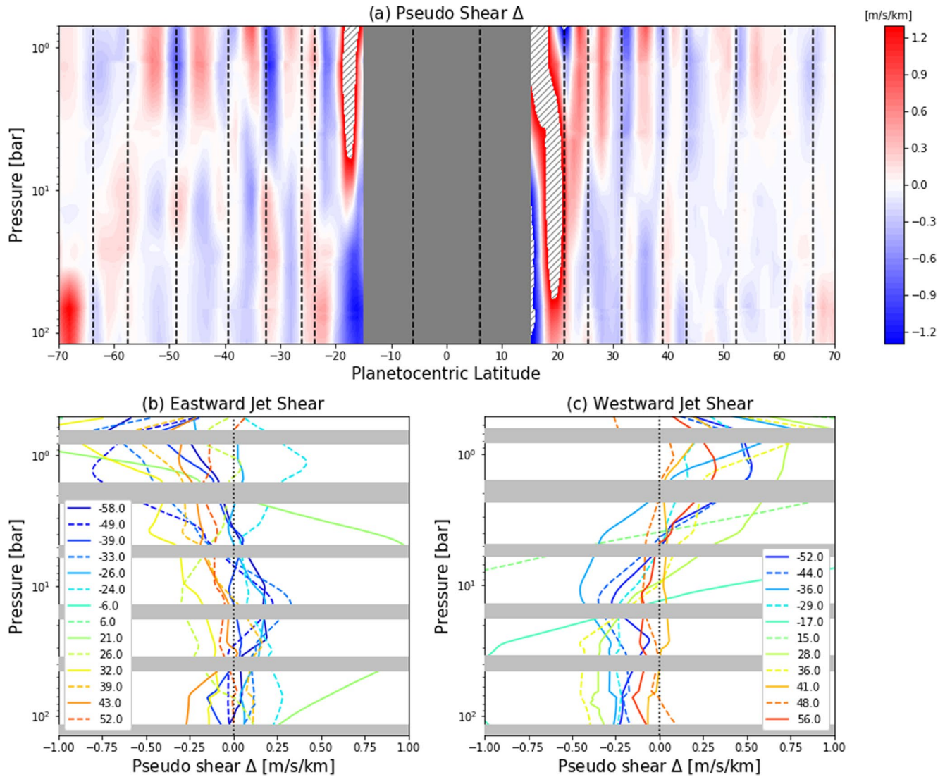
Figure 9. (a) 2D cross section of microwave radiometer (MWR) brightness gradient \Delta_{\mu}(\phi, p) , or pseudo shear, in units of m/s/km, constructed from the T_B(\phi, p) cross section in Figure 8. The color scale is saturated at \pm 1.3 m/s/km to emphasise gradients at midlatitudes, values of \Delta_{\mu} exceeding this range are shown as gray hatches. Tropical regions at latitudes less than 15^{\circ} are omitted. Vertical dashed lines indicate the locations of the cloud-top prograde jets. (b and c) Extracting the MWR pseudoshear \Delta_{\mu} from (a) near to the locations of the eastward (b) and westward (c) jets, as shown by the planetocentric latitudes in the legends. Gray horizontal bars indicate regions without MWR vertical sensitivity (as defined by Figure 6) and discontinuities in the calculation of \Delta_{\mu} . Tropical pseudoshears exceed \pm 1 m/s/km over much of the domain, so cannot be seen on this figure. The pseudoshear generally reverses sign near the 10-bar level, especially for southern-hemisphere jets.
