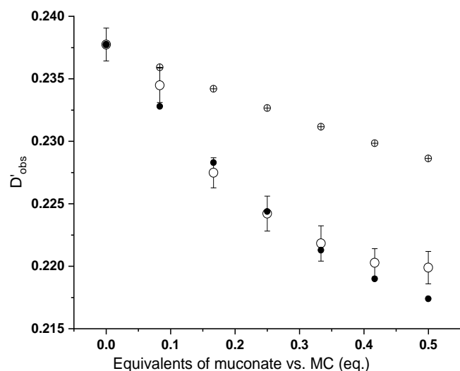
Figure 3: Regression analysis of the NMR titration of Eu-MC with muconate. Open circles: observed D'_{\text{obs}} values for the titration of Eu-MC with up to 0.5 eq. of muconate. Black dots: calculated D' at the points of the titration using the speciation of EuMC provided by calorimetric data (2:1 species present in the speciation). Crossed circles: calculated D' at the points of the titration using the speciation of SmMC provided by calorimetric data (2:1 species not present in the speciation).
