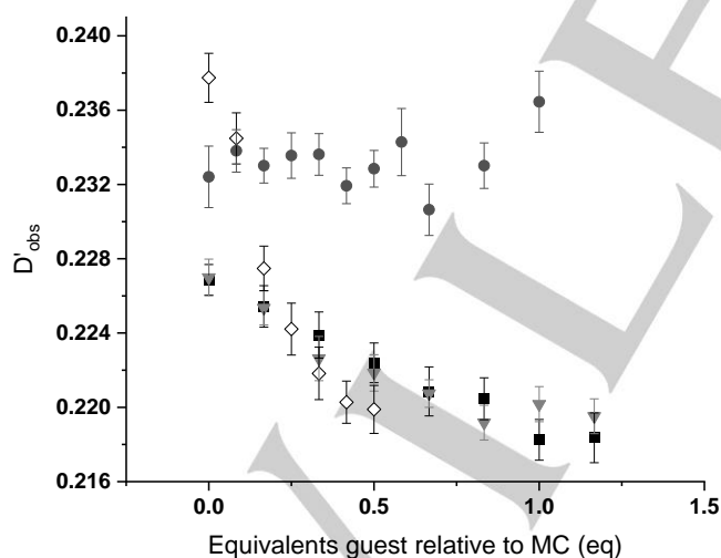
Figure 2: Change in diffusion coefficient of the Ln III [15-MC Cu II (L- pheHA )-5] 3+ species, characterized by D'_{obs} = D_{obs}/D_{DMSO} as it is titrated with muconate or sorbate guest as determined by NMR. Black squares: Nd-MC (2 mM) with 40 mM Muc; gray triangles: Sm-MC (2 mM) with 40 mM Muc; open diamonds: Eu-MC (6 mM) with 60 mM Muc; dark gray circles: Eu-MC (6 mM) with 60 mM sorbate. Each point was calculated as the ratio of the exponential decay parameters determined by fit of combined data of multiple PGSE 1 H NMR experiments. Eu-MC/Muc titration at 6 mM resulted in significant precipitation after 0.5 eq muconate added.
