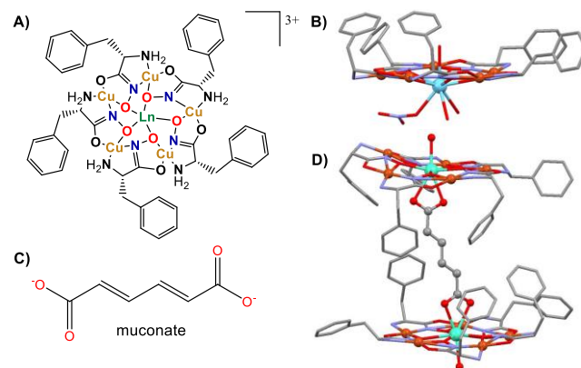
Scheme 1: Illustrations of (\text{Ln}^{\text{III}}[\text{15-MC}_{\text{Cu}^{\text{II}}\text{N}(\text{L-pheHA})-5}])^{3+} (A and B), [4a] dicarboxylate guest (C), and host-guest-host dimeric compartment (D). [4c]
