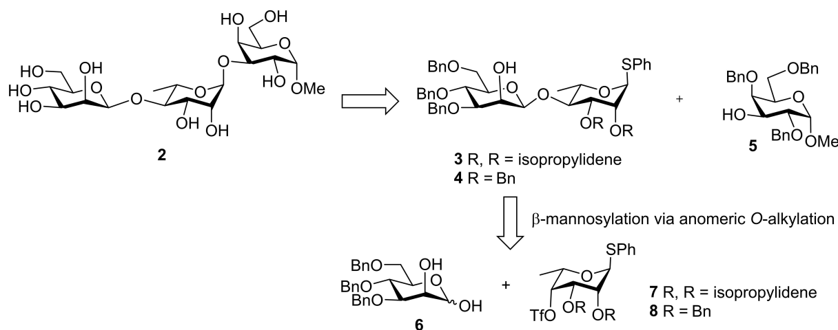
Scheme 1. Synthetic strategy for trisaccharide (2).
