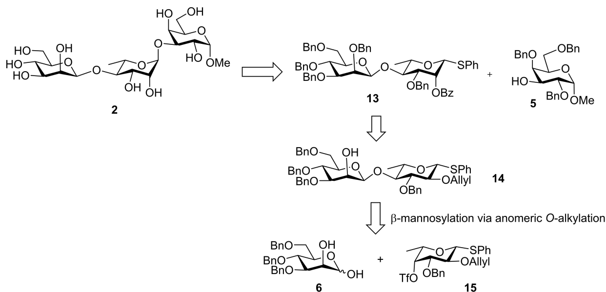
Scheme 3. Revised synthetic strategy for trisaccharide ( 2 ).
