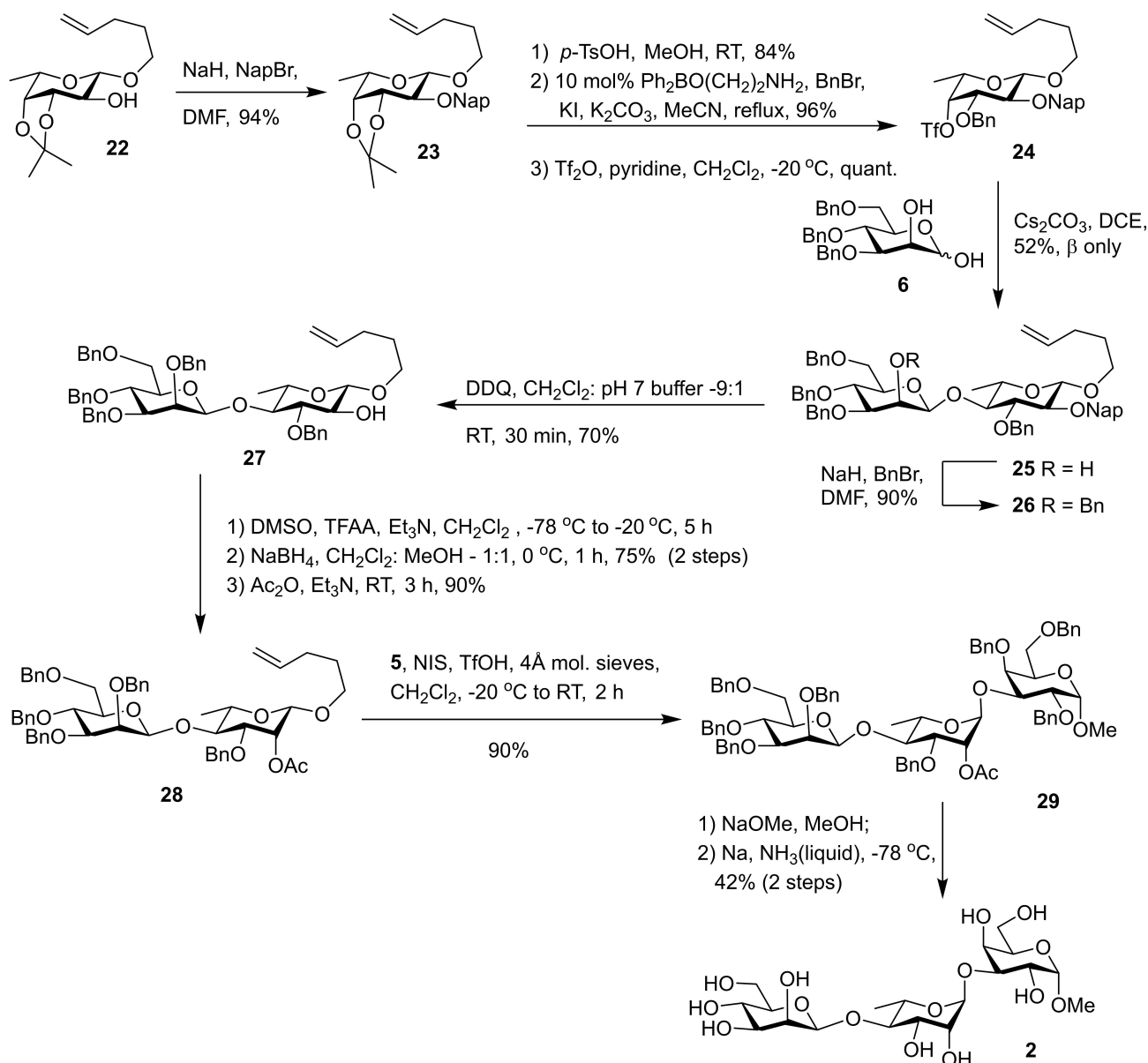
Scheme 6. Synthesis of trisaccharide (2).
