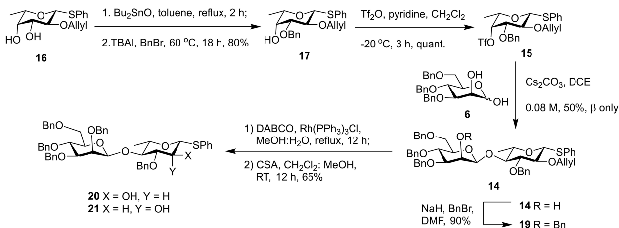
Scheme 4. Anomeric O -alkylation of D-mannose with L-fucose-derived triflate 15 .
