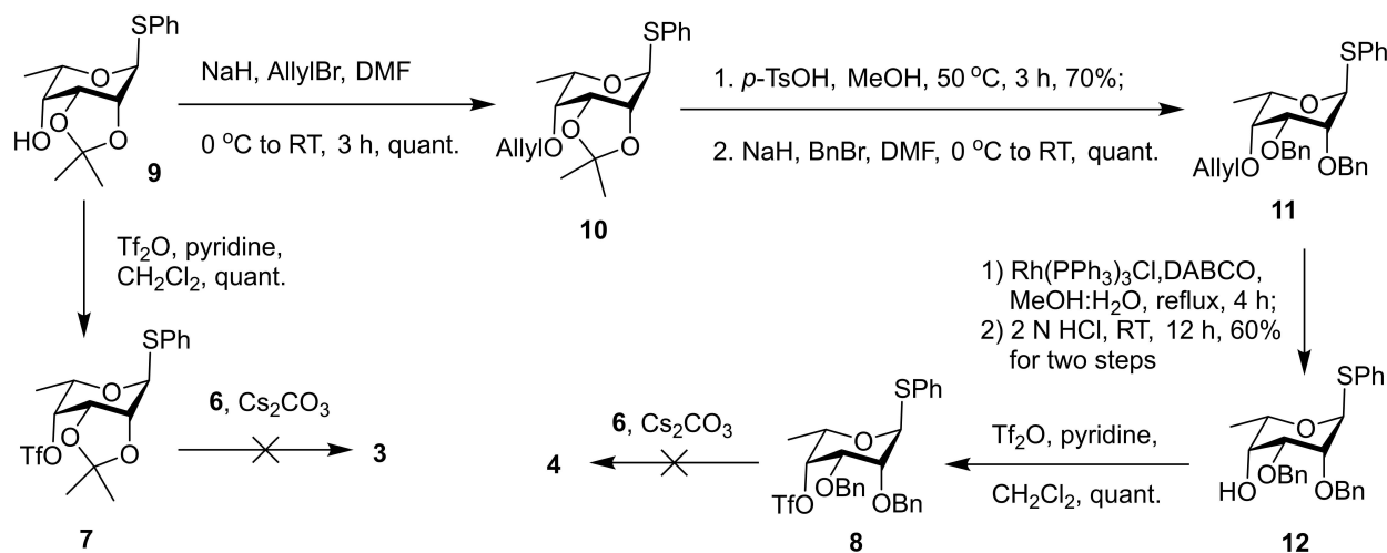
Scheme 2. Attempted anomeric O-alkylation of D-mannose with 6-deoxy-L-talose-derived C4-triflates 7 and 8 .
