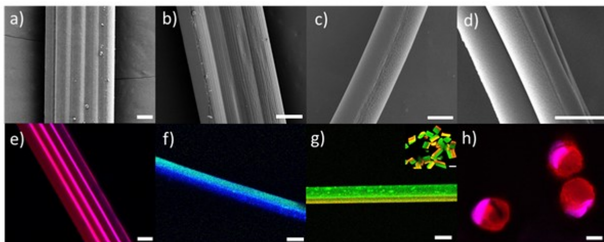
Figure 3. FE-SEM and CLSM images of biphasic microstructures in diverse polymer combinations. a, e) TPU and PMMA, b, f) PLGA and PVCi, c, g) PLGA and PMMA, d, h) PMMA and PVCi. The scale bar is 10 \mu\text{m} in all images.
