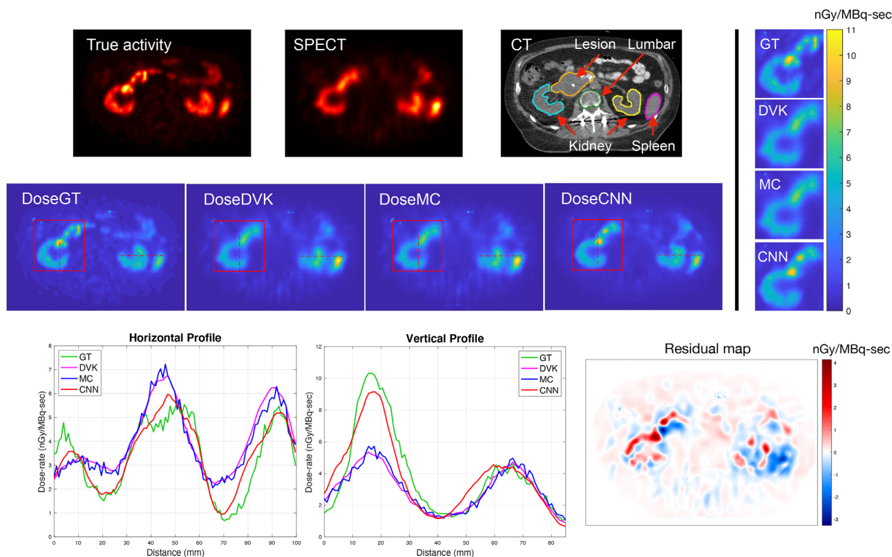
FIGURE 4 One slice of the test virtual patient phantom #2. The top two branches show the true activity map defined based on Ga-68 PET, SPECT, and CT images, the ground truth dose-rate map, and the dose-rate images from the different methods (DVK, MC, and CNN). The bottom branch shows line profiles across the kidney and the residual map (the difference between CNN and DVK dose-rate map). The dose-rate units were normalized to 1 MBq in the field-of-view in all figures
