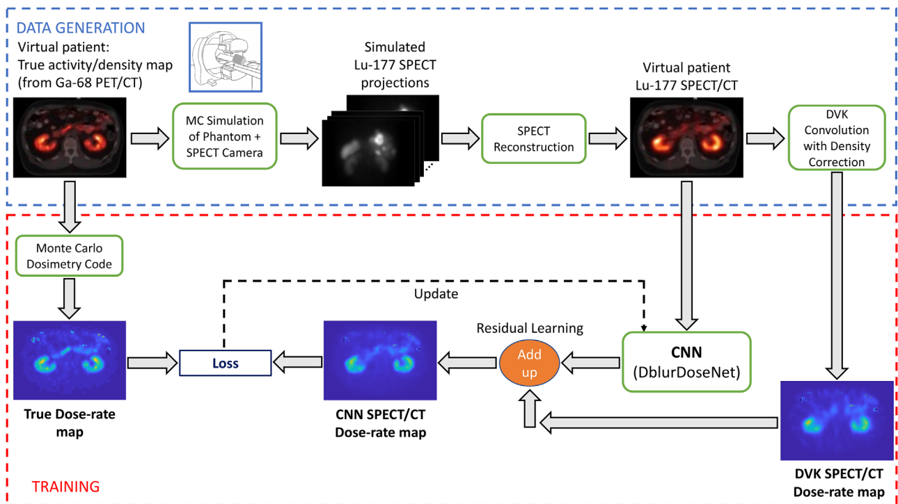
FIGURE 2 Overview of phantom data generation for training/testing and the network training process
