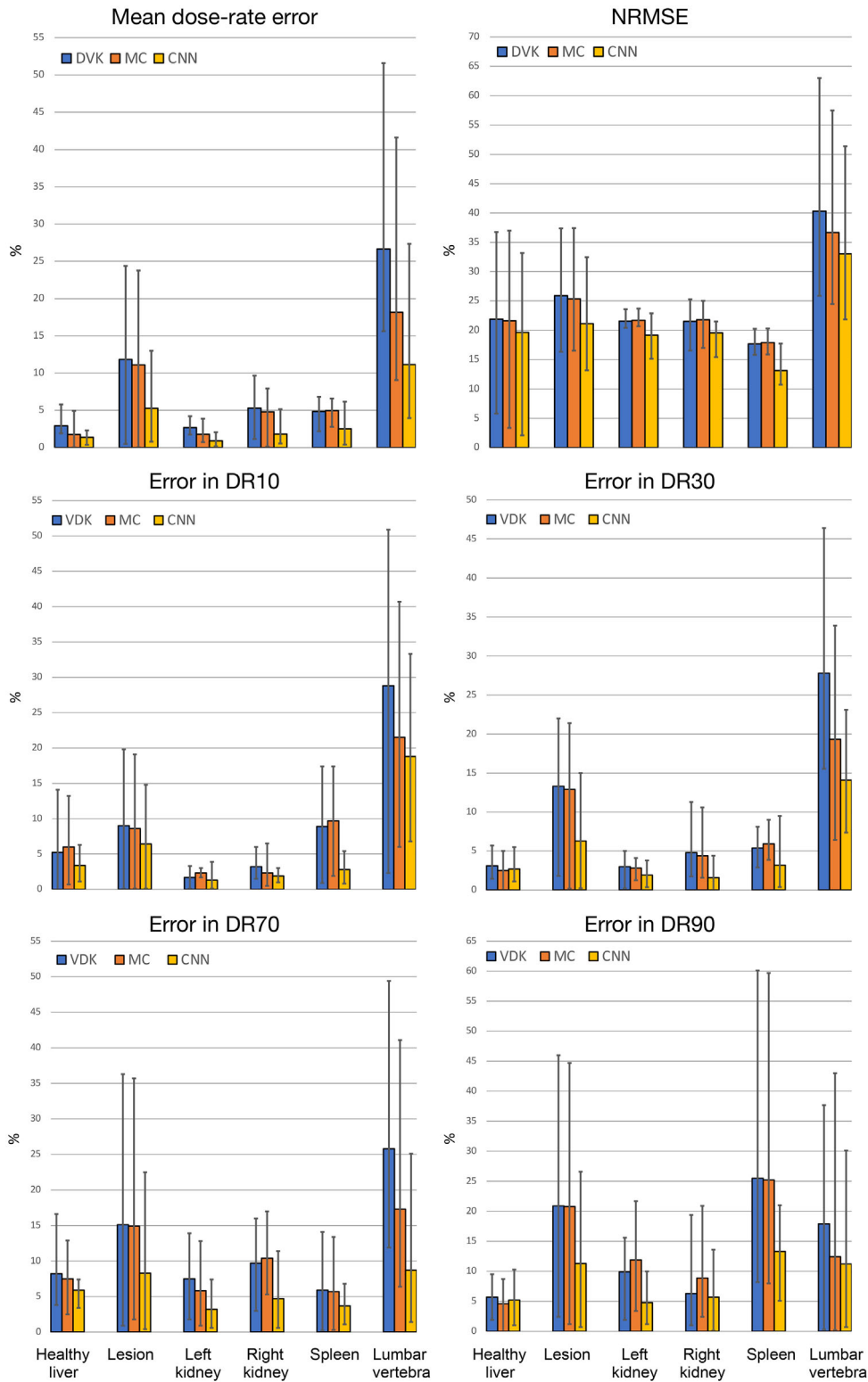
FIGURE 7 Mean dose-rate error, NRMSE, and error in DRVH statistics (DR10, DR30, DR70, DR90) comparison of DVK, MC, and CNN relative to ground-truth dose-rate map across all test phantoms. Median (range) VOI volumes are as follows: healthy liver (liver minus lesions): 1607 ml (1164–2262 ml); lesion: 16 ml (4–181 ml); left kidney: 177 ml (98–211 ml); right kidney: 156 ml (76–249 ml); spleen: 191 ml (131–467 ml); lumbar vertebra L2 to L5: 54 ml (34–68 ml)
