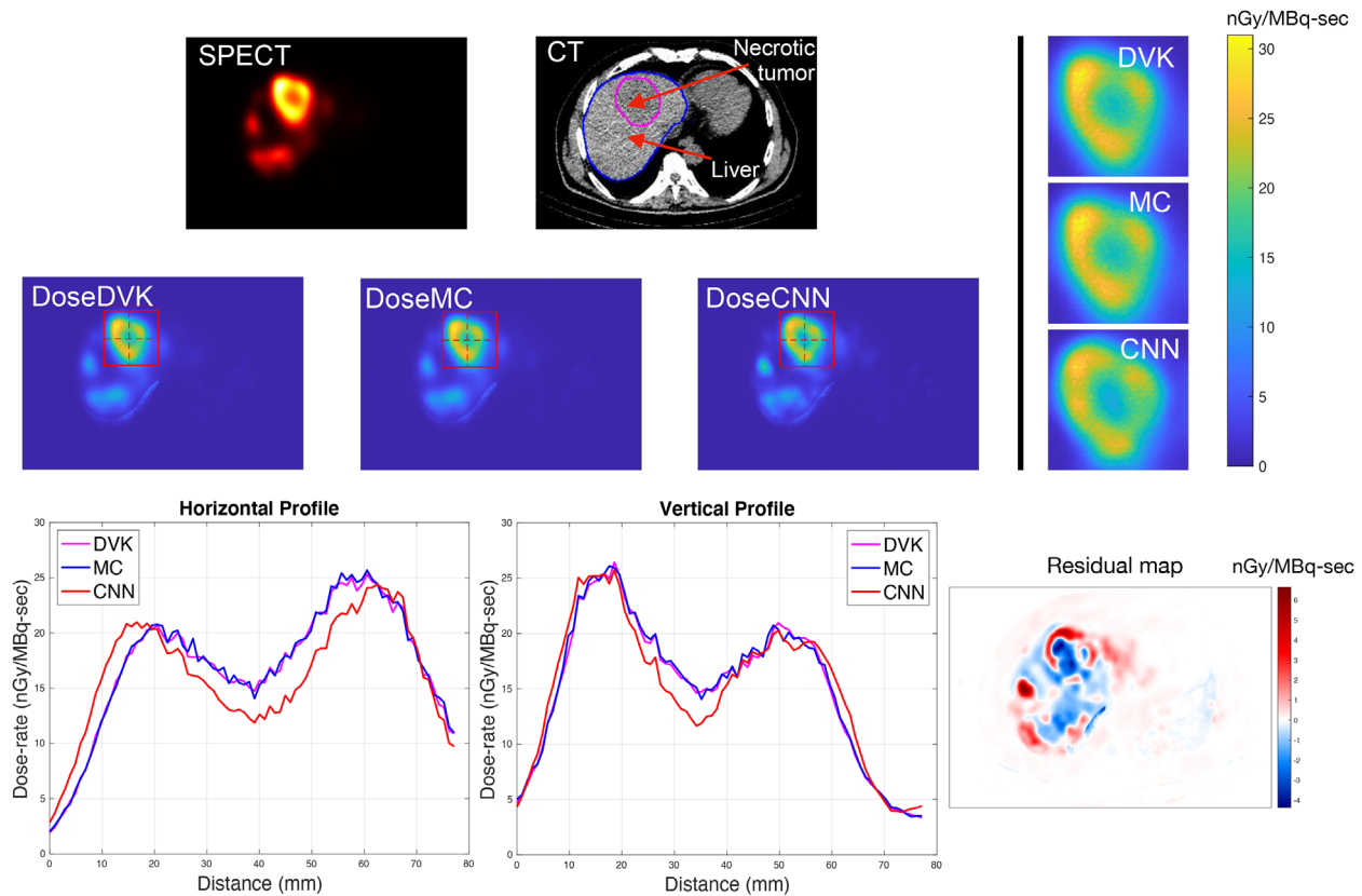
FIGURE 9 One slice across lesion of the input images (SPECT, CT) and output DVK, MC, and CNN dose-rate maps and line profiles for a patient imaged after Lu-177 DOTATATE (at day 7 post-therapy). The residual map is the difference between CNN and DVK dose-rate map
