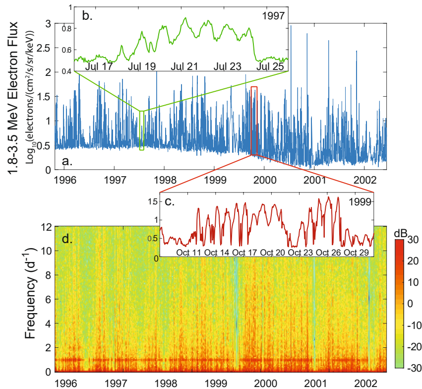
Figure 1. Electron flux (1.8–3.5 MeV) timeplot (a) over 1996–2002, (b) timeplot of quiet period. (16–25 July 1997), (c) timeplot of disturbed period (8–30 October 1999), and (d) spectrogram over 1996–2002 showing strong signal at 24 hr (1 day -1 ) frequency with a weaker signal at 12 hr.
