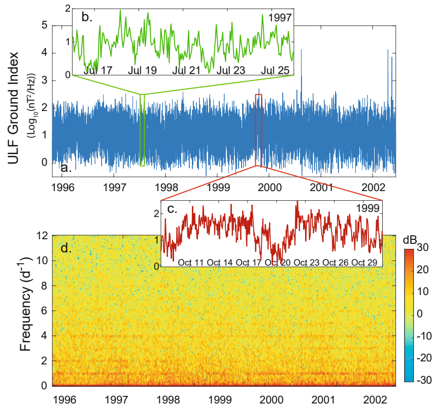
Figure 2. ULF index timeplot (a) over 1996–2002, (b) timeplot of quiet period (16–25 July 1997), (c) timeplot of disturbed period (8–30 October 1999), and (d) spectrogram over 1996–2002 showing weak signals at 24 hr (1 day -1 ), and 12, 8, and 6 hr (1/2, 1/3, and 1/4 days -1 ).
