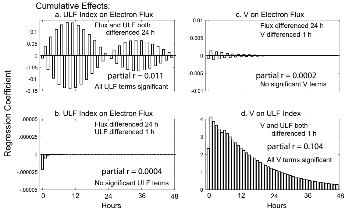
Figure 13. Cumulative lag effects from ARIMAX models: (a) the ULF index on electron flux (Model A: both differenced at 24 hr), (b) the ULF index on electron flux (Model B: flux differenced at 24 hr, ULF differenced at 1 hr), (c) solar wind velocity (differenced at 1 hr) on electron flux (differenced at 24 hr), and (d) V on the ULF index (both differenced at 1 hr). Partial correlation calculated by taking the square root of the difference in the R^2 between a base ARIMA model and the ARIMAX model with added predictor terms.
