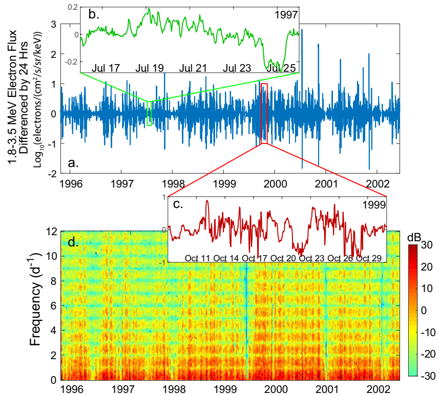
Figure 7. Electron flux (1.8–3.5 MeV) differenced by 24 hr ( y_i - y_{i-24} ): (a) 1996–2002, (b) a quiet period (16–25 July 1997), (c) a disturbed period (8–30 October 1999), and (d) spectrogram over 1996–2002 showing strong signal at 24 hr ( 1 \text{ day}^{-1} ) frequency and weaker 12 hr signal have been removed, as well as cyclicity at higher frequencies.
