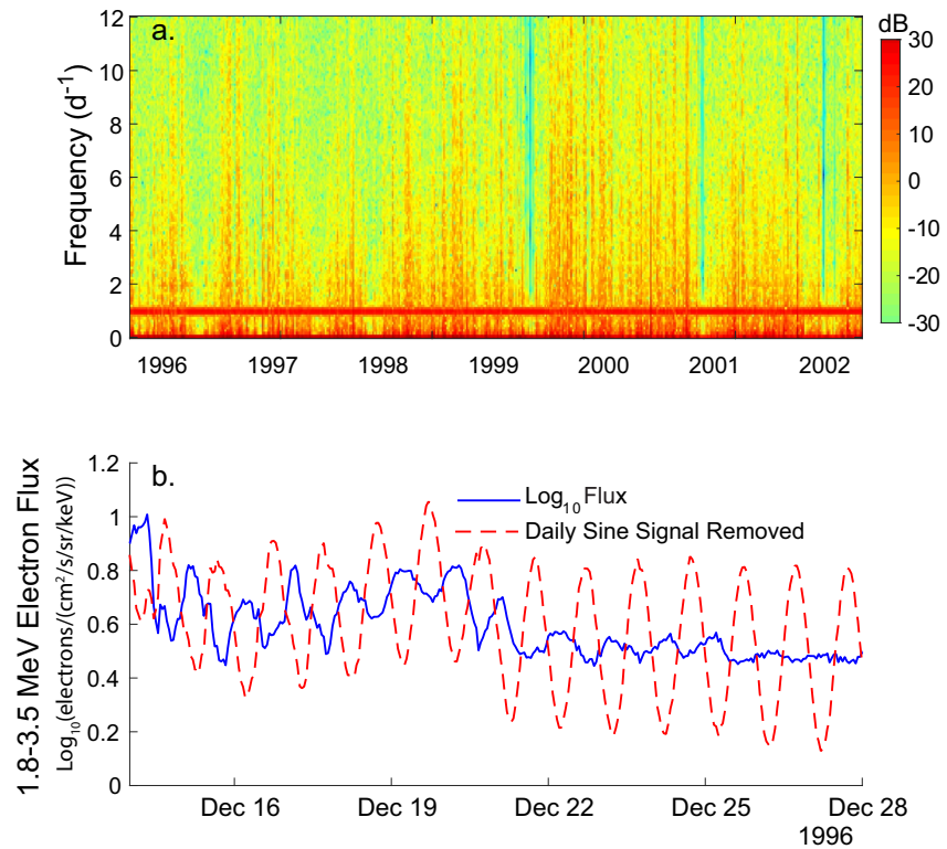
Figure 3. (a) Spectrogram of electron flux with daily sine signal removed showing the introduction of an even stronger diurnal signal. (b) Timeplot of 15–27 December 1996 period original flux (blue line) and series with daily sine wave subtracted (dashed red line).
