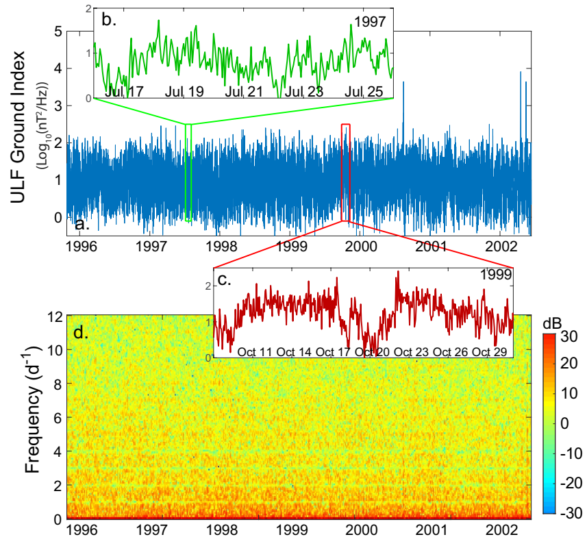
Figure 6. ULF index with daily and faster cycles removed using a bandstop filter: (a) 1996–2002, (b) a quiet period (16–25 July 1997), (c) a disturbed period (8–30 October 1999), and (d) spectrogram over 1996–2002 showing signal at 24 hr ( 1 \text{ day}^{-1} ) and weaker signals at 12, 8, and 6 hr ( 1/2 , 1/3 , and 1/4 \text{ days}^{-1} ) have been removed.
