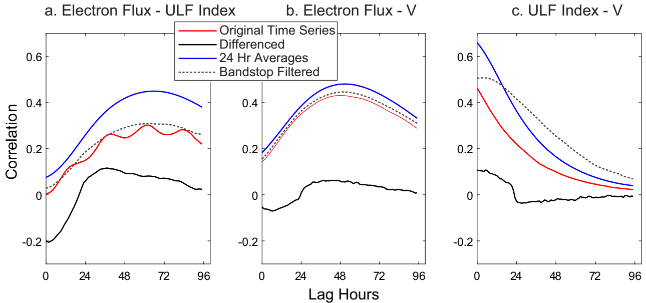
Figure 9. Correlations between electron flux, the ULF index, and solar wind velocity (V) at hourly lags over entire time series (1996–2002). The original time series (red), which may show a diurnal pattern, has lower correlations than the 24 hr averaged series (blue). Differencing by 24 hr (solid black) removes cycles and trends and results in lower correlations. Bandstop filtering (dashed line) successfully removes the diurnal cycle but not longer term trends. The bandstop filter is therefore not appropriate for long term correlation analysis.
