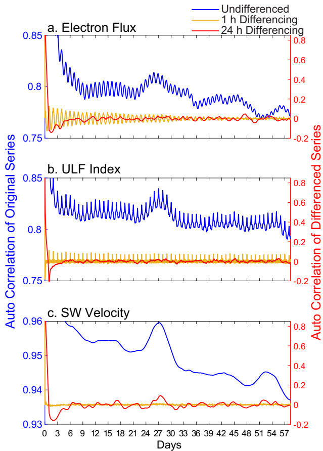
Figure 8. Autocorrelation of (a) electron flux (1.8–3.5 MeV), (b) ULF index, and (c) solar wind velocity. The high autocorrelation in each of the original time series (blue lines; left hand blue axis) can be removed by differencing at either 1 hr ( y_t - y_{t-1} ; orange line and right hand red axis) or 24 hr ( y_t - y_{t-24} ; red line and right hand red axis). Either differencing also removes the 27 days solar cycle. Differencing by 24 hr removes the diurnal cycle from both electron flux and the ULF index, but 1 hr differencing does not.
