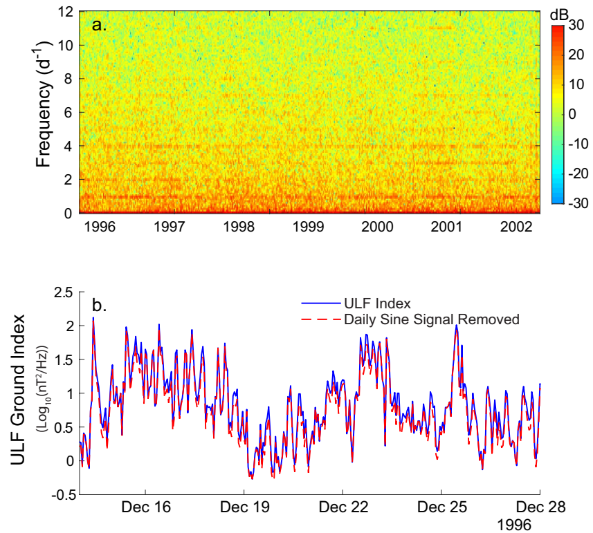
Figure 4. (a) Spectrogram of ULF index with daily sine signal removed showing the introduction of an even stronger diurnal signal, (b) timeplot of 15–27 December 1996 period original flux (blue line) and series with daily sine wave subtracted (dashed red line).
