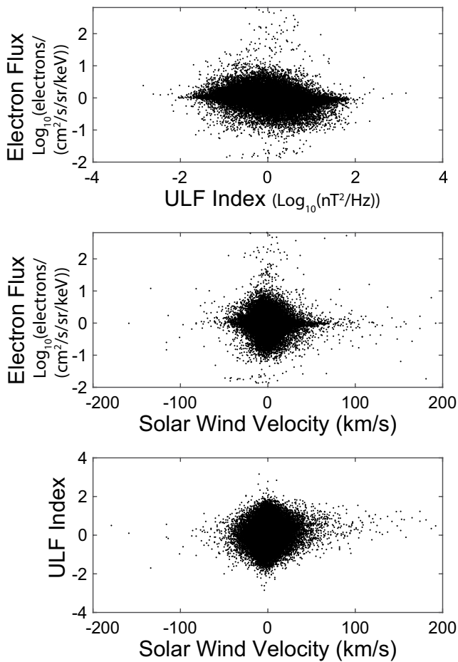
Figure 10. Lag scatterplots of the differenced time series. (a) Electron flux (differenced by 24 hr) vs. ULF index (differenced by 24 hr and measured 1 hr previous), (b) electron flux (differenced by 24 hr) vs. solar wind velocity (differenced by 1 hr and measured 1 hr previous), (c) ULF index (differenced by 24 hr) vs. solar wind velocity (differenced by 1 hr and measured 1 hr previous). There is little correlation between the differenced variables, showing that most of the correlation between the undifferenced variables is due to the common diurnal cycle and/or the 27 days solar cycle.
