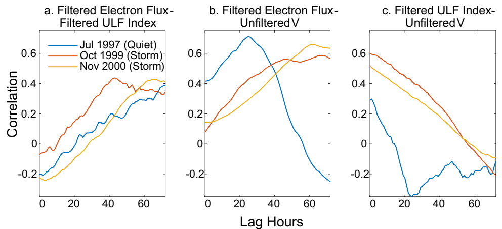
Figure 12. Correlations between electron flux, the ULF index (both with diurnal cycle removed using a bandstop filter), and unfiltered solar wind velocity (V) over 3 short time periods.
