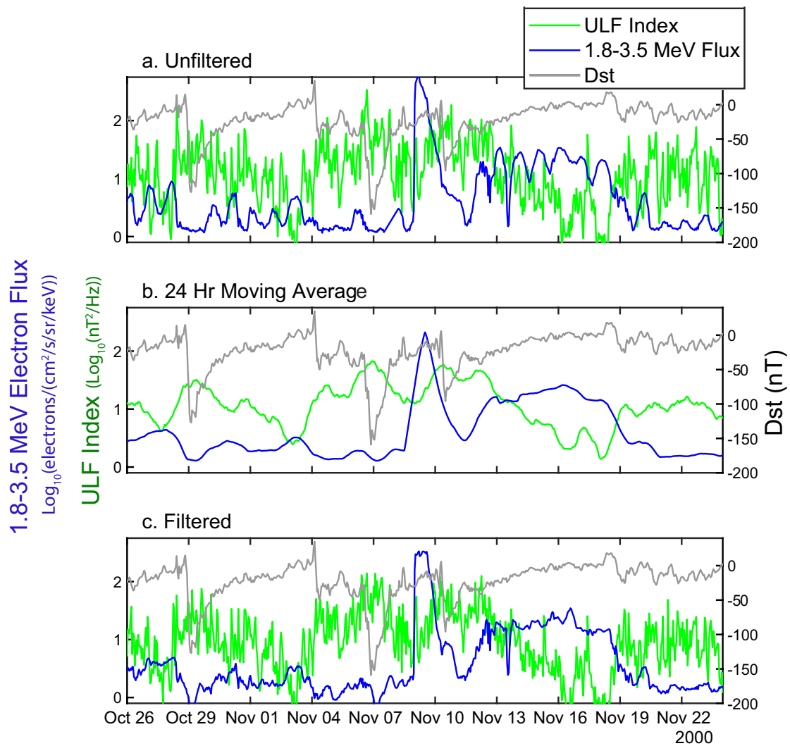
Figure 11. Timeplots of one month (26 October to 24 November 2000). (a) Original ULF index (green) and electron flux (blue) time series, with Dst (gray). (b) 24 h moving average of ULF and flux smooths the time series. (c) Bandstop filtering of ULF and flux removes the diurnal cycle.
