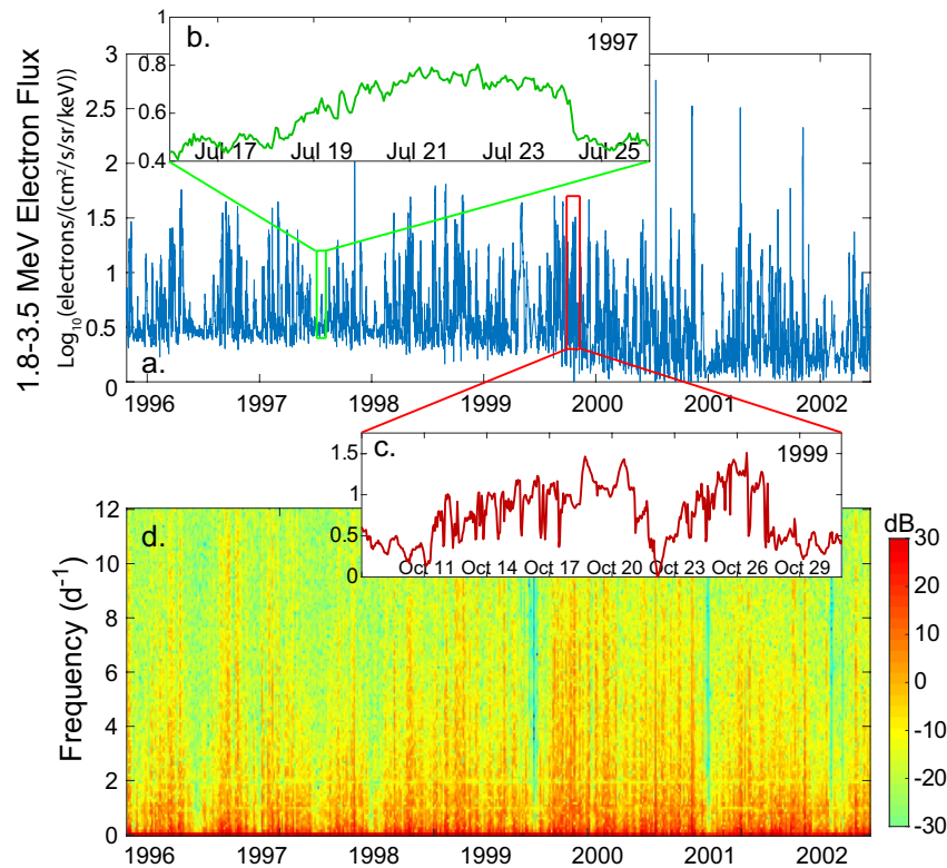
Figure 5. Electron flux (1.8–3.5 MeV) with daily and half-day cycles removed using a bandstop filter. (a) 1996–2002, (b) a quiet period (16–25 July 1997), (c) a disturbed period (8–30 October 1999), and (d) spectrogram over 1996–2002 showing strong signal at 24 hr ( 1 \text{ day}^{-1} ) frequency and weaker 12 hr signal have been removed.
