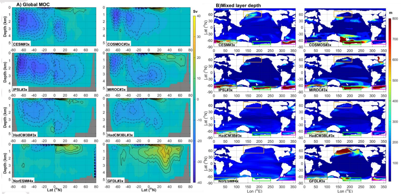
Fig. 2 A) Global meridional overturning circulation (MOC) (contour interval: 4 Sv) showing mostly anticlockwise overturning circulation, and B) mixed layer depth (MLD) (m) for the Eocene-3x(4x) simulations. Colored boxes indicate regions used in the freshwater calculation.
