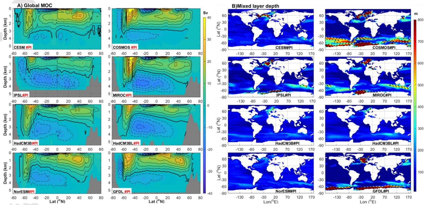
Fig. 1 A) Global meridional overturning circulation(MOC), showing overturning streamfunction in the unit of Sverdrups (Sv, contour interval: 4 Sv) for the pre-industrial simulations (PI-1x), consisting of the NADW (positive values indicate clockwise circulation using solid lines) and Antarctic bottom waters AABW (negative values indicate anticlockwise circulation using dashed lines, and the zero contour is bold). B) maximum mixed layer depth (MLD, in m), indicative of deepwater formation sites. Dashed lines mark 500 m contour.
