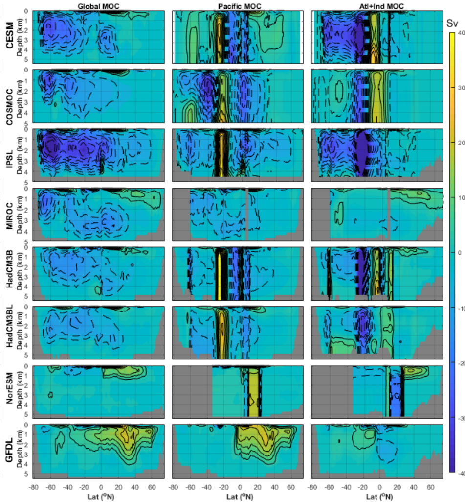
Fig. 3 Separation of AMOC and PMOC from the global MOC in Eocene-3x simulations to show overturning circulation in two basins. Large values in the tropics indicate inter-basin exchanges, and a northward shift of these values in NorESM likely due to their more north tropical gateway that probably relate to their paleomagnetic reference bathymetry frame. NB, AMOC and PMOC in the CESM, COSMOS, IPSL and MIROC models are calculated offline.
