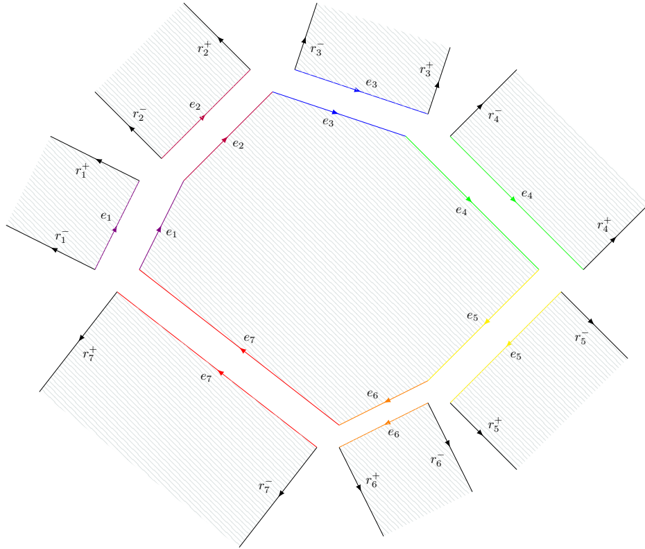
FIGURE 9. A non-degenerate 7-polygon with the corresponding half-strips.
