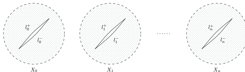
FIGURE 1. Sequential slit construction
