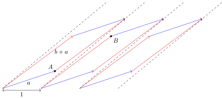
FIGURE 25. For sufficiently large n , horizontal translates of the parallelogram formed by a and b+na by 1 unit are disjoint. In this example, n = 1 . The dotted line depicts a new fundamental domain for the infinite half cylinder with base e_j from which a parallelogram with sides a and b+na can be cut out.
