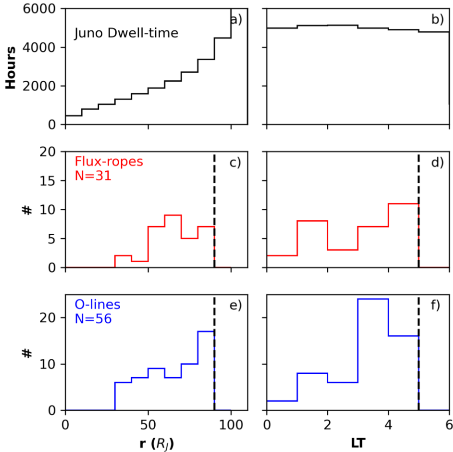
Figure 11. Histograms of the locations of the identified flux-rope and O-line events in radial distance and local time. Time spent by the Juno spacecraft in each bin is shown in panels a) and b). The dashed lines mark the limits of the detection algorithm.
