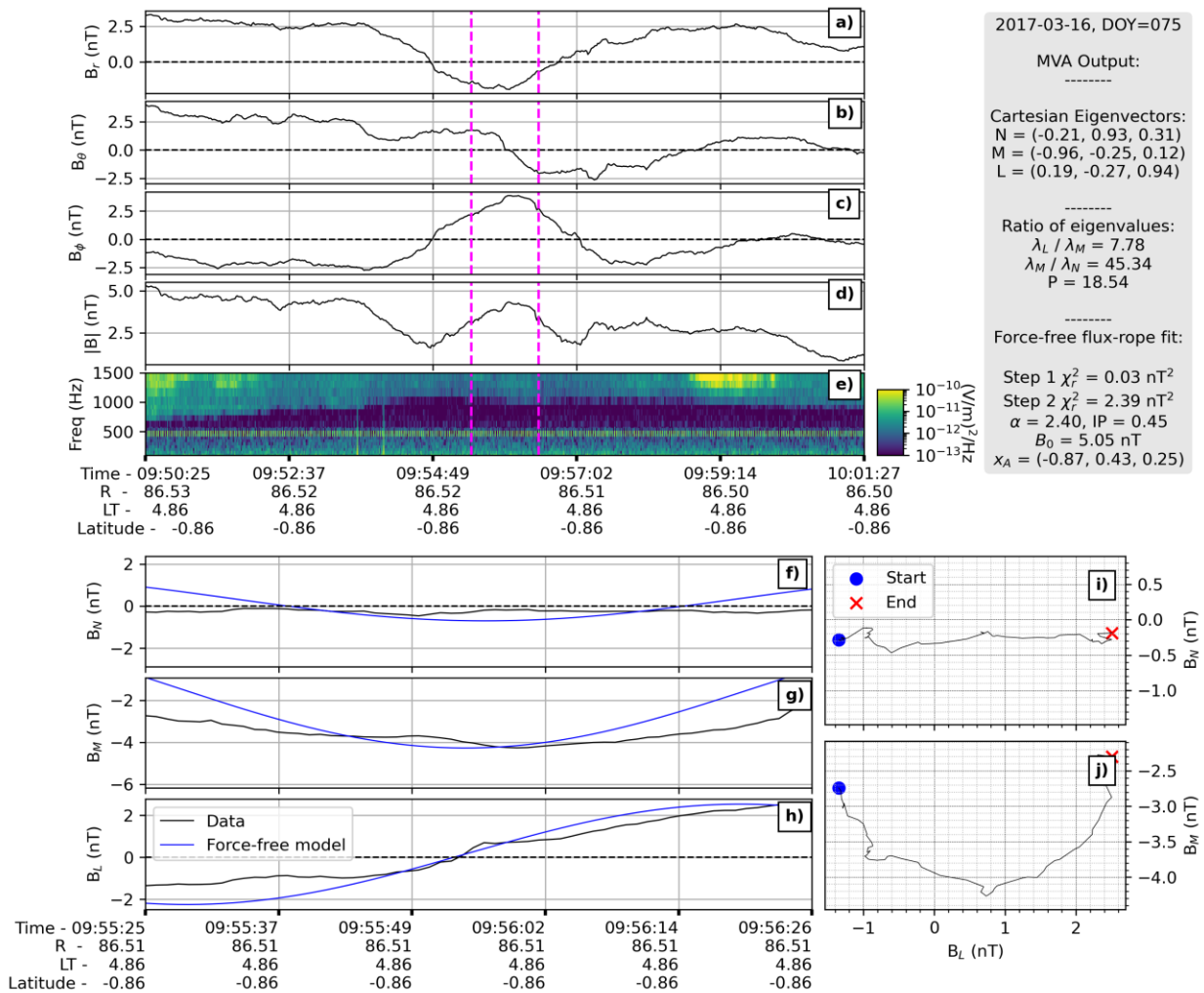
Figure 3. Magnetic field observations of a magnetic flux-rope event on DOY 75, 2017 by the Juno spacecraft in the dawnside magnetotail. Panels (a)-(d) show the magnetic field intensity in the spherical JSS coordinate system. The Waves electric field spectra is shown in Panel (e). Panels (f)-(g) show the components of the magnetic field in the minimum-variance coordinate system corresponding to the minimum, intermediate and maximum eigenvector. The magnetic signature of the best-fit modeled force-free flux-rope is shown in blue. Panels (h)-(i) show the
