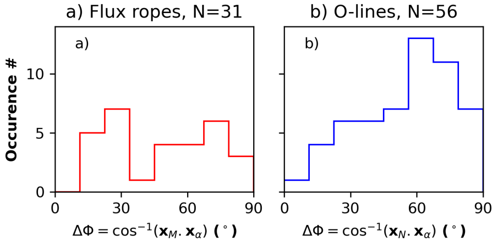
Figure 14. Histograms showing the acute angle between the core-field direction and the local bend-back plane for a) flux-rope and b) O-lines identified by the algorithm.
