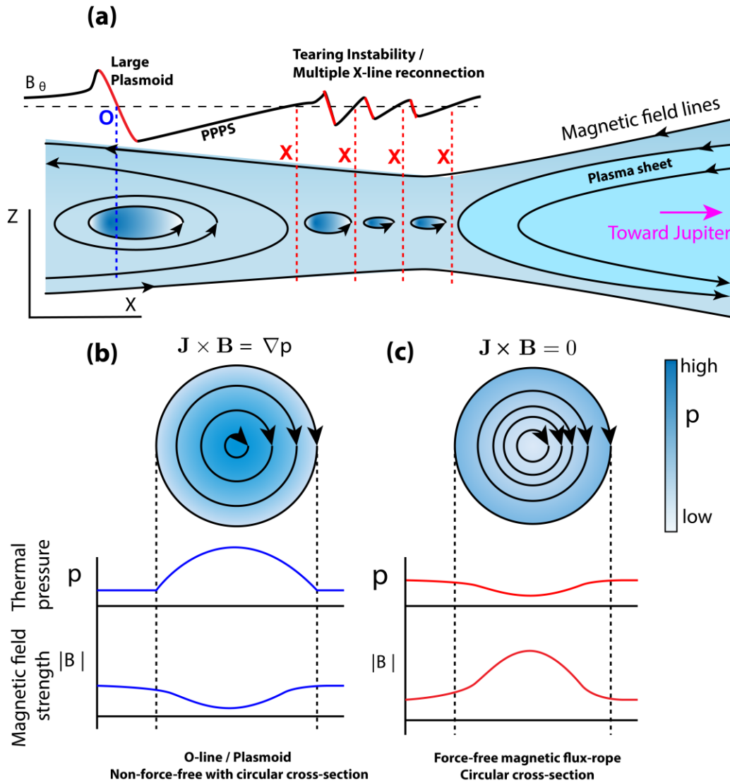
Figure 2. (a) Magnetic signature and representative geometry of a tailward moving plasmoid with a post-plasmoid plasma sheet. (b-c) Schematics showing the different magnetic field and thermal pressure profiles of magnetic O-lines (b) and force-free flux-ropes (c) with circular cross-sections. In (a), the magnetic signature in the north-south component is shown for the specific case when all plasmoids are moving tailward with respect to the spacecraft.
