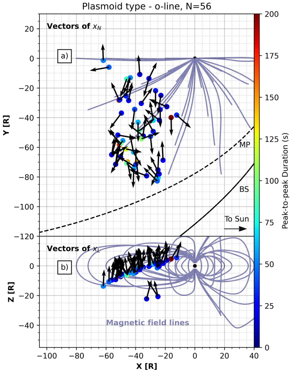
Figure 13. Eigenvectors of the minimum and maximum variance shown in the equatorial and meridional projections for the 56 O-line events identified by the algorithm. Each event is colored
