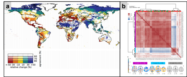
Figure 16: Two examples of domain-specific visualizations of multiverse analyses. (a) outcome values are contextualized in a geographical map [Bie15], (b) correlation matrix of outcome values [BNHC* 20].
