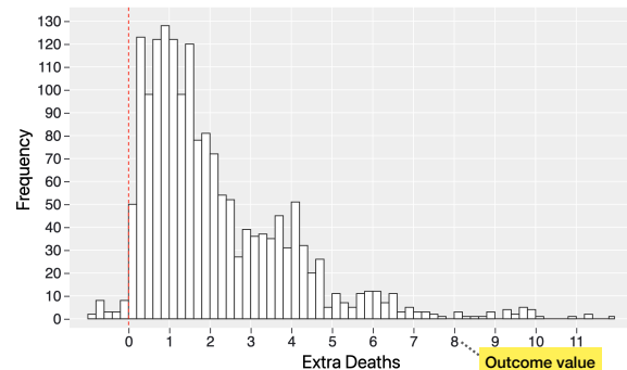
Figure 5: Example of an outcome histogram. Recreated after Steegen et al. [STGV16], but using the hurricane dataset (section 2). The x-axis encodes outcome values (effect size estimates), while the y-axis shows the count across the multiverse.
