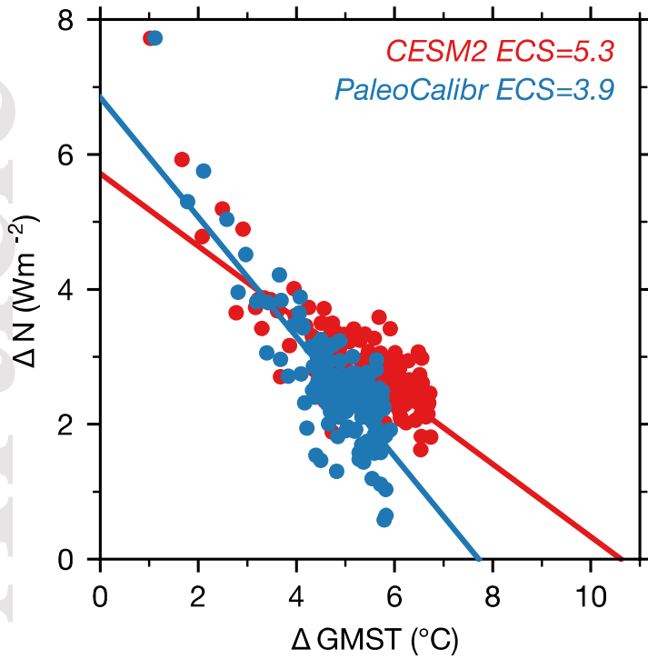
Figure 12. Scatter plot of the global mean surface temperature anomaly ( \Delta \text{GMST} ) and the top-of-atmosphere net radiation ( \Delta N ) in the abrupt 4\times\text{CO}_2 simulations using CESM2 and PaleoCalibr. 4\times\text{CO}_2 simulations are run for 150 model years. Equilibrium Climate Sensitivity (ECS) is estimated using the regression method, i.e., a half of the x-axis intercept.
