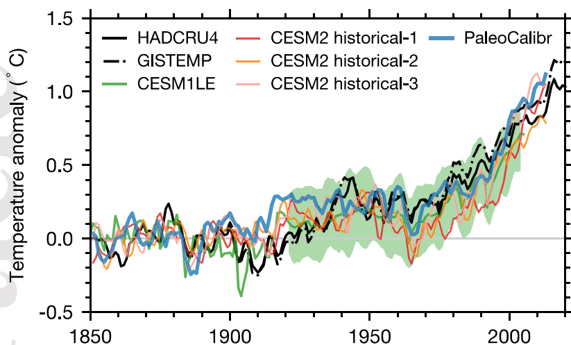
Figure 10. Time series of the global mean surface temperature anomaly during the historical period from observations (black), the CESM2 historical simulations using CAM6 (three members in red, orange, and pink), and the paleoclimate-calibrated configuration (PaleoCalibr; blue). Results from the CESM1 Large Ensemble (CESM1LE; green) are shown as a reference for a possible range of internal variability. The observations are from the HADCRU4 and GISTEMP. Temperature anomalies are calculated from the respective 1850–1900 averages.
