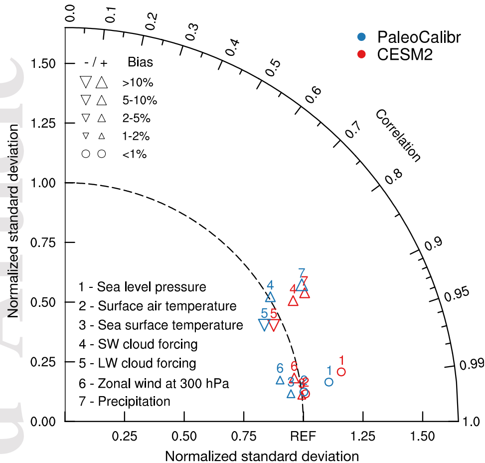
Figure 11. A Taylor diagram evaluating key climate variables in CESM2 and PaleoCalibr coupled historical simulations using observational and reanalysis datasets. Model simulated sea level pressure, surface air temperature, and zonal wind at 300 hPa are compared with averages between 1979 and 2014 from ERA5, shortwave and longwave cloud radiative forcing compared with averages between 2000 and 2014 from CERES-EBAF, precipitation compared with averages between 1979 and 2014 from GPCP, and sea surface temperature compared with averages between 1979 and 2014 from ERSST.
