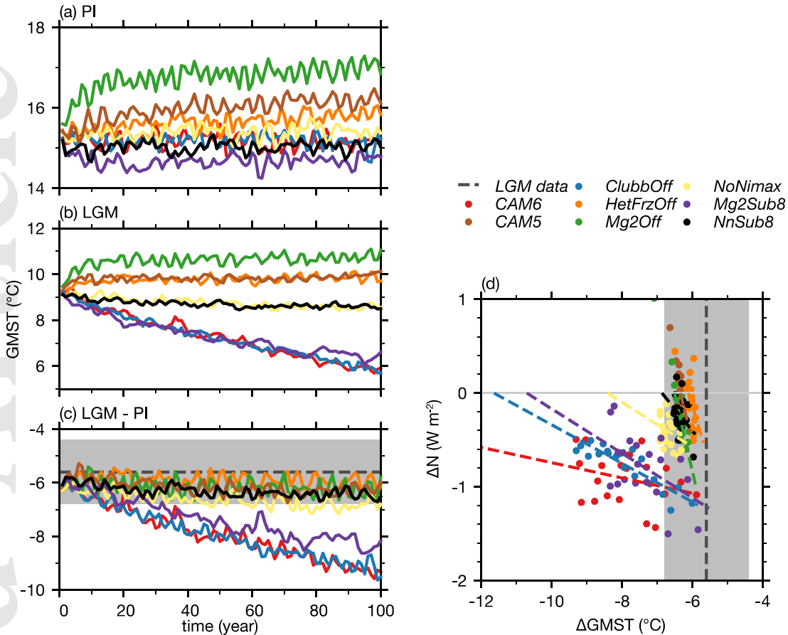
Figure 2. Time series of global mean surface temperature (GMST) in (a) the preindustrial (PI) and (b) the Last Glacial Maximum (LGM) simulations using various atmosphere model configurations within the coupled CESM2 framework. (c) Changes in GMST between paired LGM and PI simulations. (d) Changes in top-of-atmosphere radiation ( \Delta N ) versus GMST ( \Delta GMST ) in paired simulations. \Delta N and \Delta GMST (markers) are the 5-year running mean of the LGM time series with the last-30-year averages of the PI simulation subtracted. A linear regression between \Delta N and \Delta GMST is shown as dashed line for each configuration. In (c) and (d), the LGM \Delta GMST and the 95% uncertainty interval from Tierney et al. (2020) are shown. See text and Table 1 for details of the model configurations.
