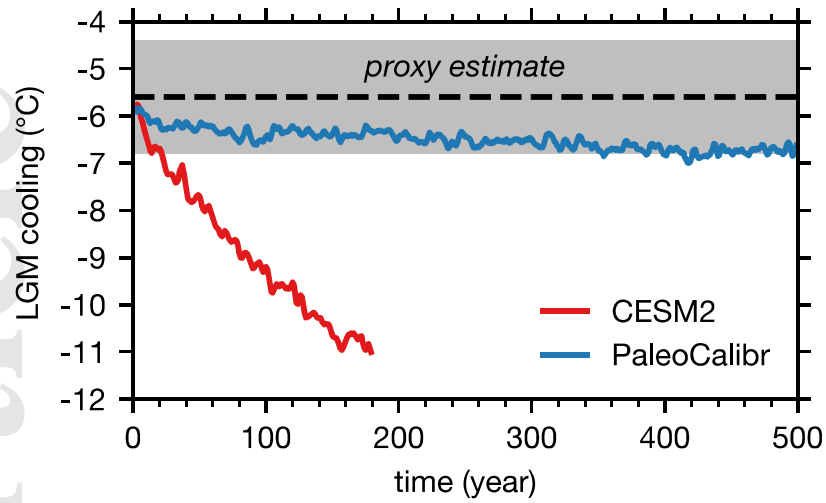
Figure 7. Time series of the global mean surface temperature anomaly in the LGM simulations with CESM2 and the paleoclimate-calibrated (PaleoCalibr) configurations. Black dashed line with the gray patch denotes the 95% uncertainty interval from Tierney et al. (2020) for the LGM global cooling.
