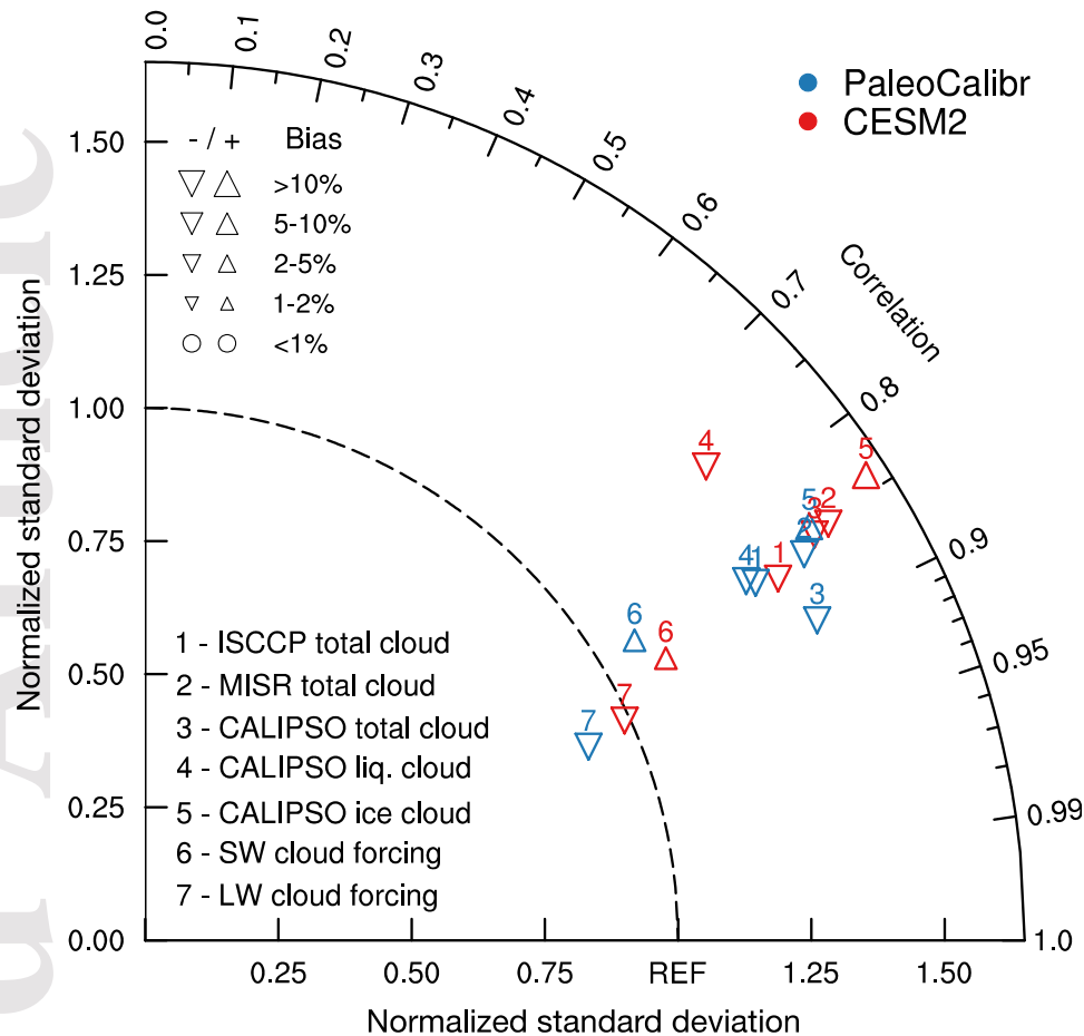
Figure 8. Taylor diagram evaluating key cloud variables in CESM2 and PaleoCalibr with satellite observations. Model variables are from AMIP historical simulations with an active Cloud Feedback Model Intercomparison Project Observational Simulator Package. Cloud observations are the total cloud fraction from ISCCP (60°S–60°N), MISR (60°S–60°N and ocean-only), and CALIPSO, the cloud phase partition between liquid and ice from CALIPSO, and the shortwave and longwave cloud radiative forcing (SWCF and LWCF) from CERES-EBAF. Averages between 2000 and 2014 are used for the model-data comparison, except for the CALIPSO cloud fraction that is averaged between 2008 and 2020.
