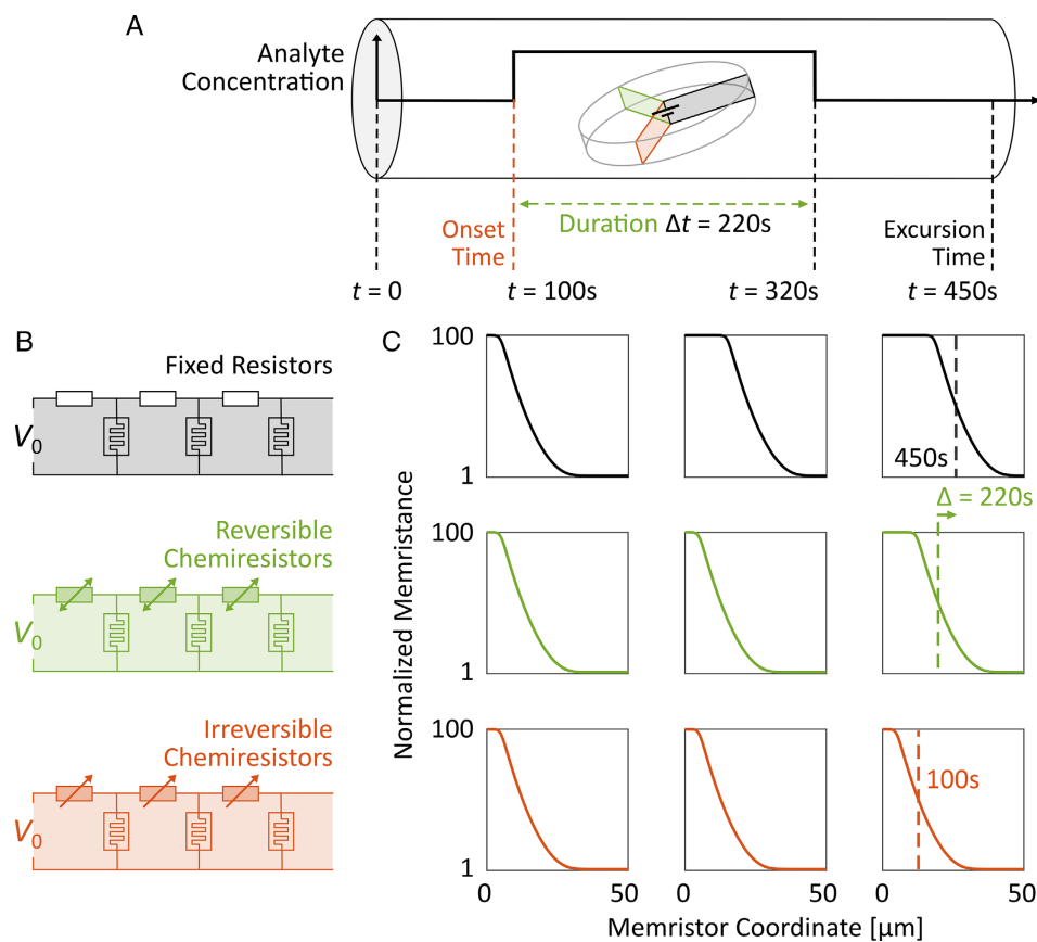
Figure 2. A) Illustration of a sensing robot traveling down a pipeline with an oxygen-rich leak region to be detected and reported. B) Memristor arrays with fixed resistors, reversible chemiresistors, and irreversible chemiresistors. C) Memristor states of the three respective arrays (top down: black, green, and red) at t = 100 , 320, and 450 s (left to right), which correspond to the times right before the robot enters the leak region, exits the leak region, and ends the voyage. The panel for t = 450 s shows that the final memristor states allow the excursion time, the duration, and the onset time to be extracted, and in turn location and length of the leak. V_0 = 1 V, \mu/L^2 = 1 s ^{-1} V ^{-1} , \alpha = 100 , oxygen concentration [\text{O}_2] = 250 ppm for t \in [100 s, 320 s] and 0 otherwise. The chemiresistor response R_R([\text{O}_2]) follows that described in Ref. [138].
