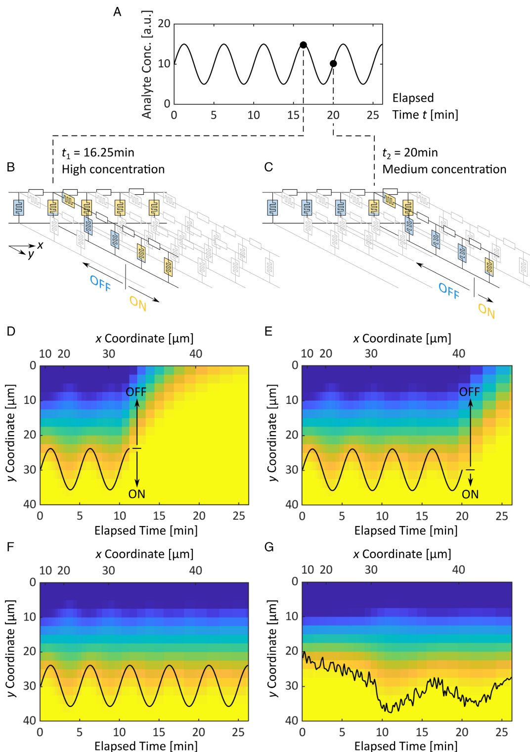
Figure 3. A) An example of a colloidal robot's history to be recovered from the 2D memristor states. B,C) Schematics of the 2D memristor array architecture at t = 16.25 min and 20 min, when the robot detected a high and medium concentration of analyte, respectively. The different concentrations are reflected in the corresponding branches as the different extent of switching. Blue, OFF; yellow, ON. \alpha = 200 . D,E) The 2D memristor states at t = 16.25 min and 20 min. The branches are sequentially activated over time, and each encoding the analyte concentration of a certain t . F,G) The final 2D memristor states of a robot experiencing a sinusoidal and realistic analyte profile, respectively. The profiles overlaid on top as solid curves conform well to memristor array readouts. Parameter values used in the simulations are listed in Methods S1.3, Supporting Information.
