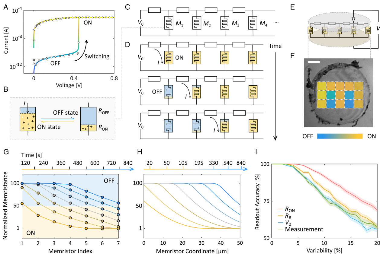
Figure 1. A) The experimental (circles) and simulated (colored curve) I - V relations of a representative memristor which is switched from OFF to ON. Experimental data digitized from ref. [137]. The memristance ranges from 37.5\text{ k}\Omega (ON, yellow) to 10\text{ G}\Omega (OFF, blue). B) The classical model of a single memristor's switching dynamics, in which the memristor is turned OFF or ON as a current I shifts the phase boundary. C) The memristor array architecture which comprises an energy input V_0 , memristors M_n in parallel bridged by either fixed resistors for logging excursion time or chemiresistors as sensors. D) The sequential switching phenomenon along a memristor array illustrated. As time elapses, the initially ON memristors are switched OFF sequentially. The final memristor states therefore encode time. E) Literature has shown that a continuous matrix of memristive ink material printed or coated between resistive 2D sheets is equivalent to an array of memristors in parallel. F) On a particle stamped out from the sandwich stack, different regions of the continuous memristive layer can be selectively switched ON/OFF by an applied voltage with the currents diffusing slowly. Scale bar, 50\text{ }\mu\text{m} . Data adapted from Ref. [38]. G) Simulated normalized memristance of seven discrete memristors in parallel. Memristors are sequentially switched OFF as time elapses. V_0 = 1\text{ V} , \mu/L^2 = 1\text{ s}^{-1}\text{ V}^{-1} , \alpha = R_{\text{OFF}}/R_{\text{ON}} = 100 . H) Simulated normalized memristance of a continuous memristor array. The switched OFF region of the memristive layer expands over time. V_0 = 1\text{ V} , \mu/L^2 = 1\text{ s}^{-1}\text{ V}^{-1} , R_R = 1.75\text{ k}\Omega\text{ }\mu\text{m}^{-1} , \alpha = 100 . I) Even with a high variability in R_{\text{ON}} , R_R , V_0 , or with a high measurement error of 20%, the majority of the 400 simulated memristor arrays report the correct excursion time. As microrobots are deployed and retrieved in batches, this allows the correct time to be interpreted.
