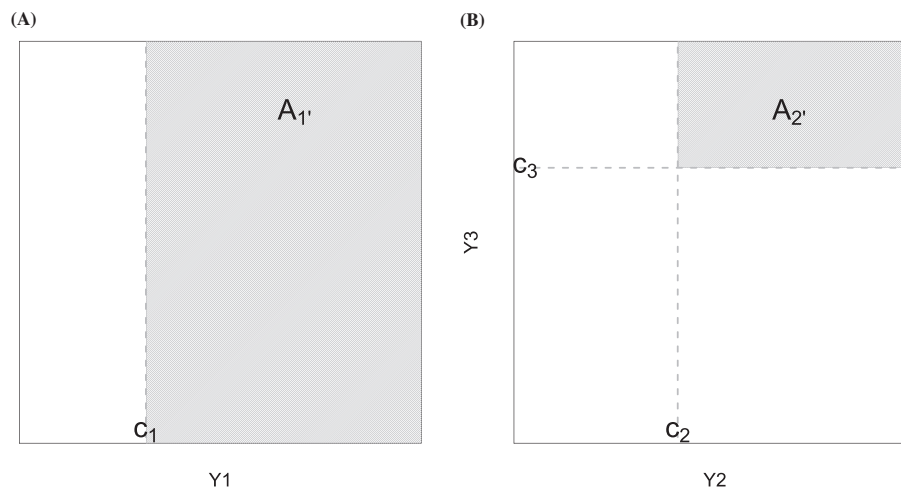
FIGURE 1 In the example, we define a positive screening rule Y_1 > c_1 OR (Y_2 > c_2 AND Y_3 > c_3) . Then in set notation we define (A) A_{1'} = B_1 , where B_1 = \{(y_1, y_2, y_3) : y_1 > c_1, y_2 \in \mathbf{R}, y_3 \in \mathbf{R}\} and (B) A_{2'} = B_2 \cap B_3 , where B_2 = \{(y_1, y_2, y_3) : y_1 \in \mathbf{R}, y_2 > c_2, y_3 \in \mathbf{R}\} and B_3 = \{(y_1, y_2, y_3) : y_1 \in \mathbf{R}, y_2 \in \mathbf{R}, y_3 > c_3\} . Then the positivity region \mathbf{A} = A_{1'} \cup A_{2'} . (A) Subgroup of diseased patients identified by rule Y_1 > c_1 . (B) Subgroup of diseased patients identified by rule Y_2 > c_2 AND Y_3 > c_3
