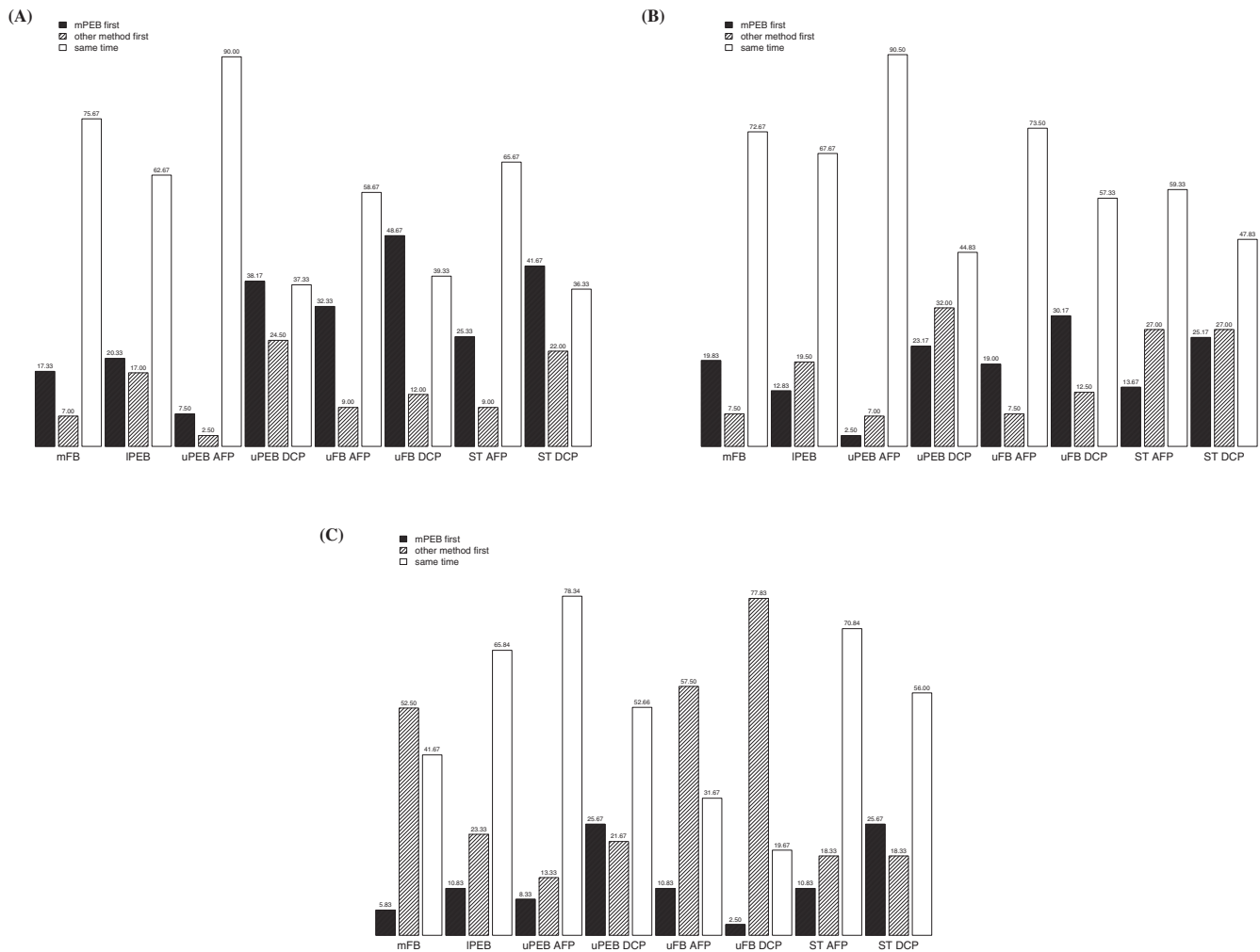
FIGURE 2 Cross-validated estimate of the percentage of times the proposed multivariate parametric empirical Bayes (mPEB) algorithm has a positive screen first, another method has a positive screen first, and the first positive screen for both is the same in the three time periods. (A) 1 year prior to clinical diagnosis. (B) 1 to 2 years prior to clinical diagnosis. (C) >2 years prior to clinical diagnosis. IPEB , regression plus univariate PEB algorithm applied to the linear combination; mFB , multivariate fully Bayesian; ST , single threshold; uFB , univariate fully Bayesian; uPEB , parametric empirical Bayes
