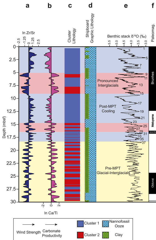
Figure 5. Elemental ratio depth series for Ocean Drilling Program (ODP) Hole 1207A sediment core between 0.0 and 30.0 m. (a) XRF-based \ln Zr/Sr ; (b) XRF-based \ln Ca/Ti ; (c) cluster lithologies; (d) shipboard visual description lithologies; (e) foraminiferal benthic stack \delta^{18}O from Ahn et al. (2017); and (f) magnetic polarity stratigraphy. Depth is further categorized into three interpreted zones; pre-MPT glacial/interglacials (yellow), post-MPT cooling (blue), and pronounced interglacials (red).
