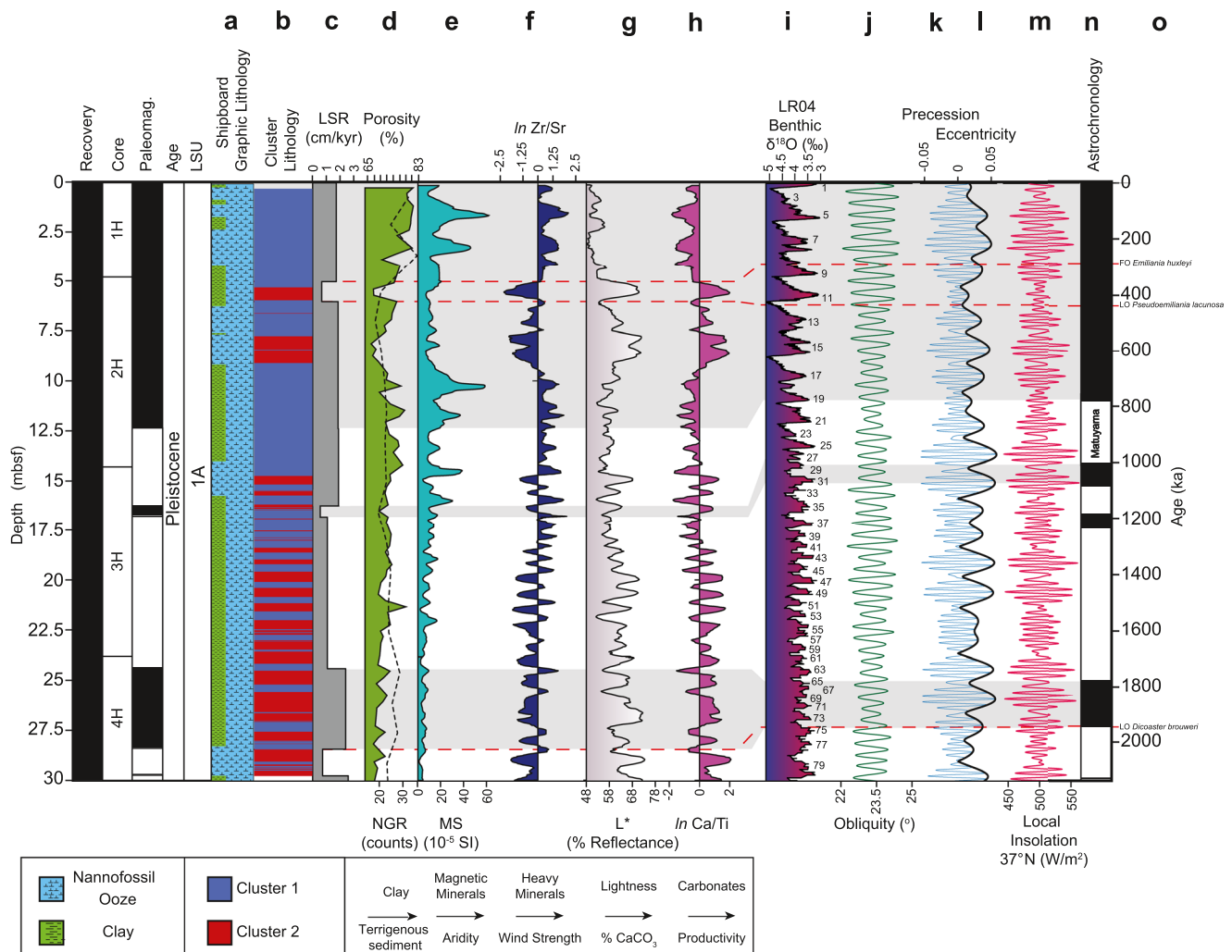
Figure 4. Depth series developed for Ocean Drilling Program (ODP) Hole 1207A between 0 and 30 mbsf and correlation to age-based time series data. Depth series data includes (a) shipboard graphic lithology column based on visual core description (Bralower et al., 2002); (b) cluster lithologies defined in this study using XRF core scanning data; (c) linear sedimentation rates (LSR) in cm/kyr determined from the age model used in this study (Table 2); (d) shipboard low-resolution physical property data of natural gamma radiation (NGR; light green), and porosity (black dashed line); (e) shipboard magnetic susceptibility (MS; Bralower et al., 2002); (f) normalized and standardized XRF-based \ln Zr/Sr ratios; (g) shipboard color reflectance data L^* ; (h) normalized and standardized XRF-based \ln Ca/Ti ratios; age-based times-series includes (i) \delta^{18}O benthic oxygen isotope stack (Ahn et al., 2017) with MIS labels for interglacial periods; (j, k, l) orbital parameters of obliquity (dark green), precession (light blue) and eccentricity (black), and insolation ( 37^\circ N ), respectively, as defined by Laskar et al. (2004); (m) astrochronology with correlation to Hole 1207A paleomagnetic normal (highlighted in gray) and reversed intervals (white background); (n) local insolation at 37^\circ N in W/m^2 ; and (o) calcareous nannofossil datums with red dashed lines depicting tie points to depth series data. Summaries of depth series data as proxies for paleoenvironmental conditions are labeled below time series data. All XRF ratios are plotted with an 11-point running mean.
