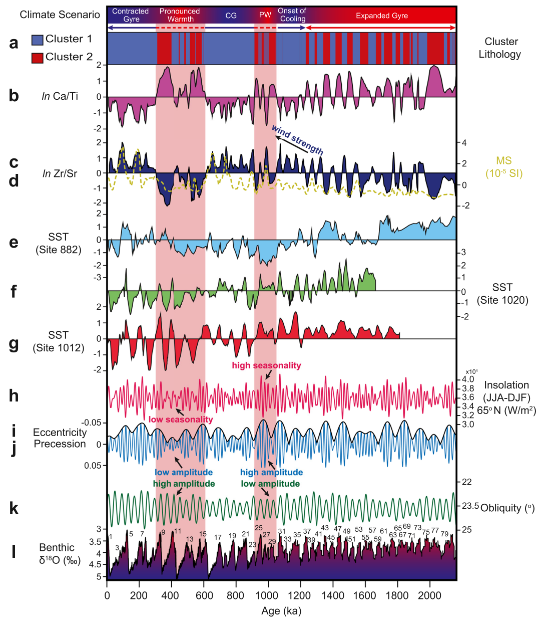
Figure 8. Age-based time series developed for Ocean Drilling Program (ODP) Hole 1207A between 0 and 2,164 ka (0–30 mbsf). Time series data includes (a) cluster lithologies defined in this study using XRF core scanning data; (b) normalized and standardized XRF-based \ln \text{Ca/Ti} ratio; (c) normalized and standardized XRF-based \ln \text{Zr/Sr} ratio; (d) shipboard magnetic susceptibility (MS; brown dashed line; Bralower et al., 2002); (e) sea surface temperatures (SSTs) from Subarctic North Pacific ODP Site 882; SSTs from eastern equatorial upwelling sites ODP Site 1020 (f) and 1012 (g); (h) insolation representing seasonality (65°N; JJA-DJF); (i, j, k) orbital parameters of eccentricity (black), precession (light blue), and obliquity (dark green). \delta^{18}\text{O} benthic oxygen isotope stack (Ahn et al., 2017) with MISs labels for interglacial periods. Red shaded boxes denote periods encompassing MIS 15-9 and 29-25 where we interpret an expanded North Pacific Subtropical Gyre and pronounced warmth over Site 1207A.
