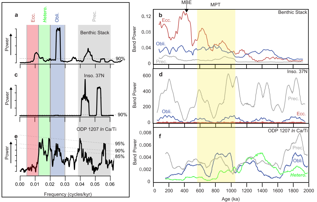
Figure 3. Power spectra and time-frequency analysis results for (a and b) benthic \delta^{18}\text{O} record (Ahn et al., 2017), (c and d) local insolation at 37^\circ\text{N} in \text{W}/\text{m}^2 , and (e and f) Ocean Drilling Program (ODP) Hole 1207A \ln \text{Ca}/\text{Ti} of normalized and standardized XRF data. Cumulative band power in the precession (0.04–0.06), obliquity (0.02–0.03), eccentricity (0.001–0.013), and heterodyne (0.0133–0.02) bands are highlighted in power spectra results (eccentricity = red, heterodynes = green, obliquity = blue, precession = gray). The Mid-Pleistocene Climate Transition (MPT) interval (highlighted in yellow) spans the interval in which there is the emergence of the eccentricity frequency in the benthic \delta^{18}\text{O} record of ice volume/deep ocean temperature until when the cumulative band power associated with eccentricity is greater than obliquity.
