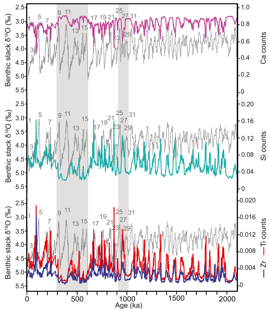
Figure 6. Normalized elemental counts from XRF core scanning at Ocean Drilling Program (ODP) Hole 1207A plotted against a global benthic foraminiferal \delta^{18}\text{O} stack (Ahn et al., 2017). Interglacial periods discussed in-text are denoted by MIS numbers. The wider vertical light gray bar indicates the periods encompassing MIS 15-9 and 29-25 when Zr, Ti, and Si counts decrease and Ca counts increase.
