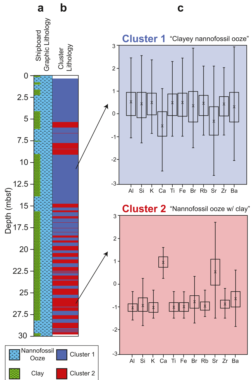
Figure 2. Cluster results depth series developed for Ocean Drilling Program (ODP) Hole 1207A sediment core between 0.0 and 30.0 m. (a) Shipboard graphic lithology from ODP Leg 198. (b) Cluster lithology displaying variability between cluster 1 (blue) and cluster 2 (red). (c) Elemental composition for cluster 1 (clayey nannofossil ooze) and cluster 2 (nannofossil ooze w/ clay).
