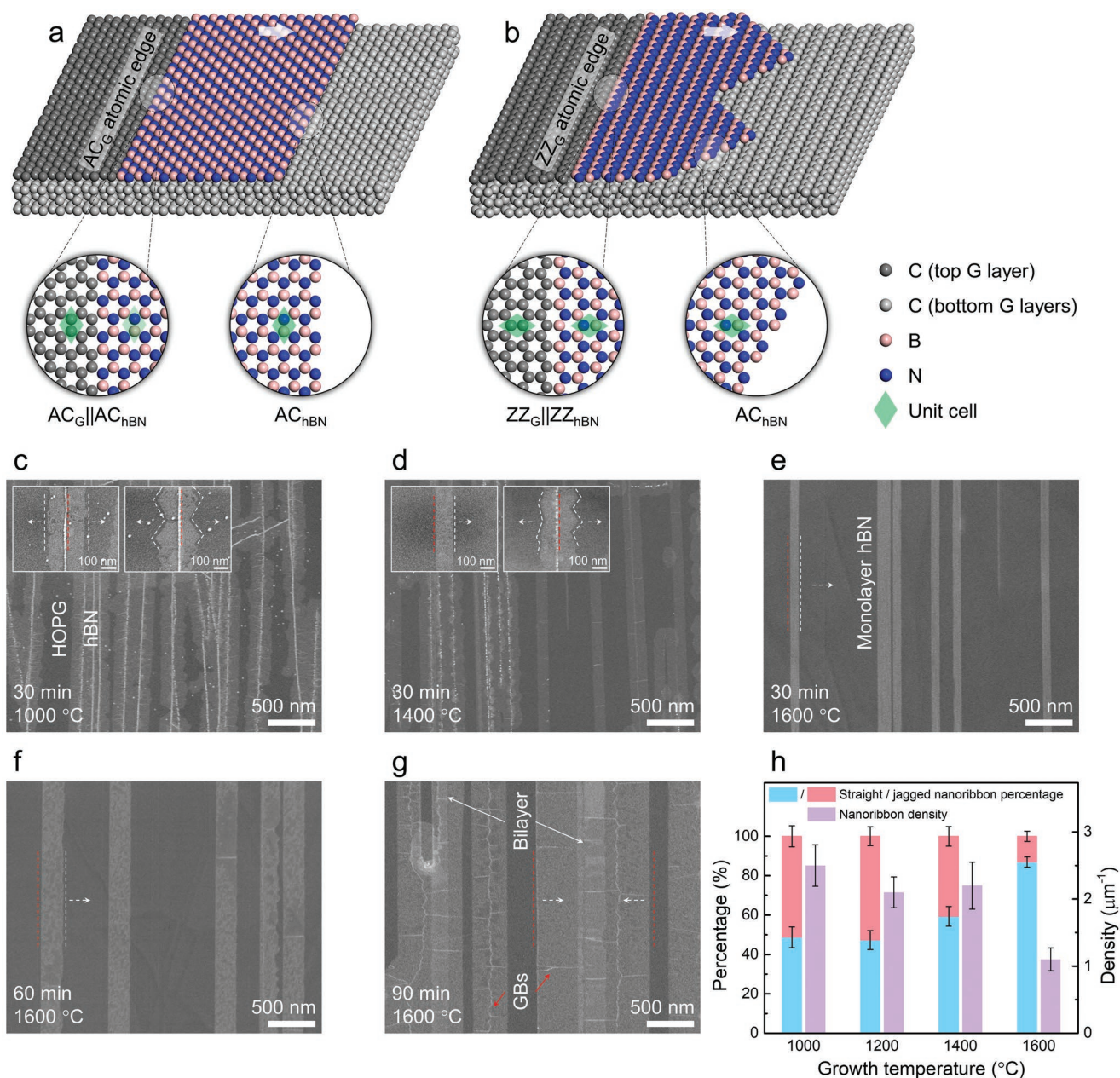
Figure 1. Concept and demonstration of interface-mediated synthesis of monolayer hBN. a,b) Schematics of monolayer hBN grown along the armchair ( AC_C ) (a) and zigzag ( ZZ_C ) (b) graphene atomic edges, forming straight and jagged nanoribbons, respectively. All growth fronts of monolayer hBN are terminated with AC_{hBN} edges. The magnifications show the atomic configurations of the AC_C||AC_{hBN} and ZZ_C||ZZ_{hBN} in-plane interfaces, and the AC_{hBN} growth fronts. The white arrows point to the growth direction. c–e) Typical SEM images of monolayer hBN nanoribbon morphology, grown along graphene atomic edges at 1000 °C (c), 1400 °C (d), and 1600 °C (e) for 30 min. The insets in (c,d) show the typical morphology of straight and jagged hBN nanoribbons. e–g) Evolution of straight monolayer hBN nanoribbons is followed after 30 min (e), 60 min (f), and 90 min (g) growth time at 1600 °C. The red dashed lines depict the hBN/graphene nucleation interfaces and the white dashed lines show the outline of hBN growth fronts; the white dashed arrows point to the growth direction. The white solid arrows indicate bilayer hBN formed from the initial hBN/graphene nucleation interfaces after underlying straight monolayer hBN nanoribbons coalescence; the red solid arrows show the GBs formed during nanoribbon growth and coalescence. h) Measured percentage of straight versus jagged hBN nanoribbons and nanoribbon density is shown as a function of growth temperature, demonstrating the dominance of straight nanoribbons (with well-defined AC_C||AC_{hBN} in-plane interfaces) at a growth temperature of 1600 °C. The error bars show the standard deviation.
