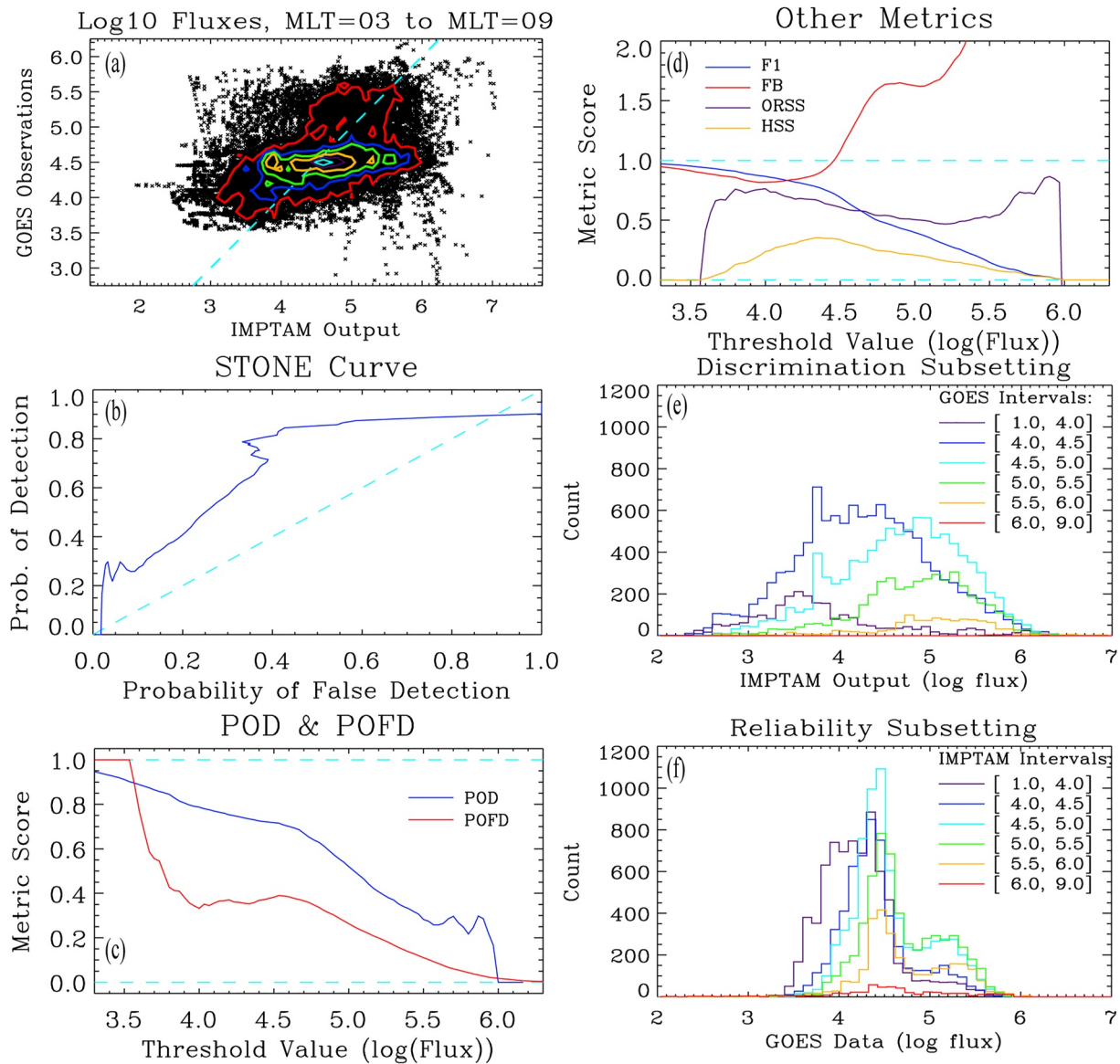
Figure 13. Comparison of 40 keV electron differential number fluxes (log base 10 of electrons \text{cm}^{-2} \text{s}^{-1} \text{sr}^{-1} \text{keV}^{-1} ) from geosynchronous orbiting environmental satellite (GOES) and real-time Inner Magnetosphere Particle Transport and Acceleration Model (IMPTAM). Shown are: (a) scatterplot of the data-model pairs with 10 bins per decade and contours drawn every 40 counts/bin increment; (b) the sliding threshold of observation for numeric evaluation curve; (c) the probability of detection and probability of false detection curves as a function of threshold; (d) the four other metrics discussed in this study; (e) discrimination subsetting histograms of IMPTAM values for six ranges of the GOES values; and (f) reliability subsetting histograms of GOES values for six ranges of the IMPTAM values. Dashed lines in cyan are included for reference.
