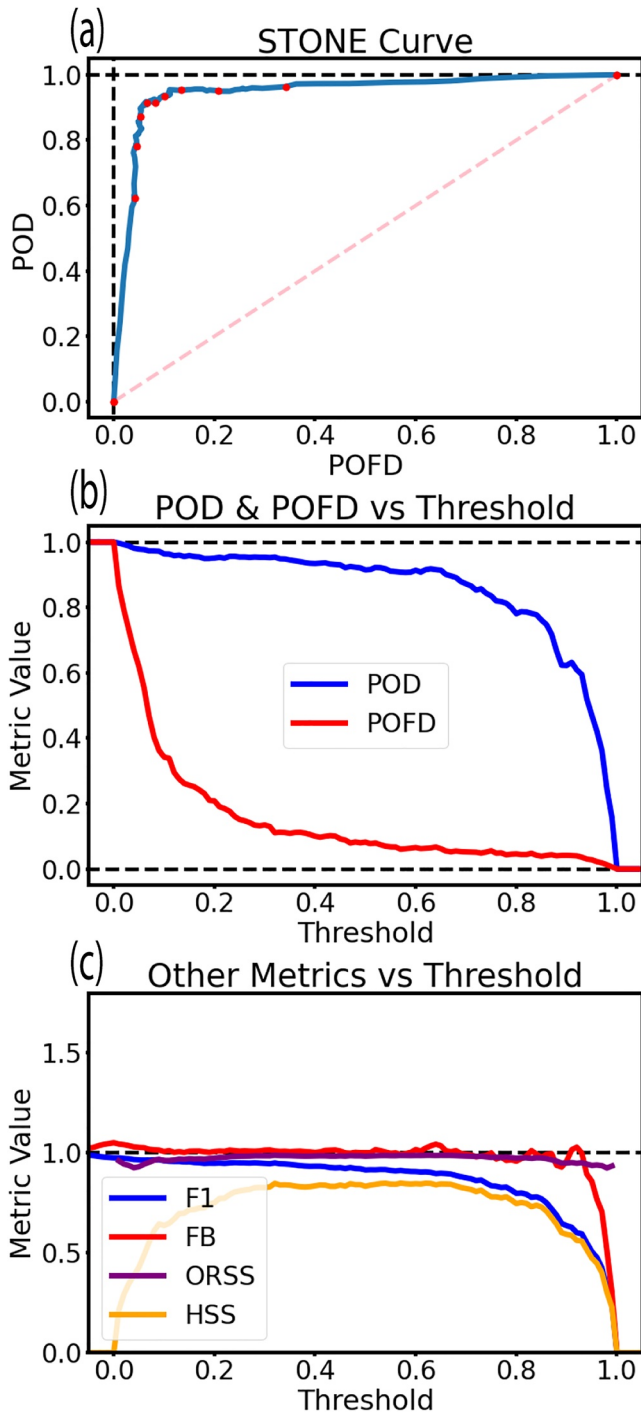
Figure 3. For the example scatterplot shown in Figure 1 with simultaneously threshold sweeps, (a) the sliding threshold of observation for numeric evaluation curve, with a red dot shown every 0.1 along the threshold sweep; (b) the probability of detection and probability of false detection scores as a function of threshold setting; and (c) four other metric scores, also as a function of threshold setting.
