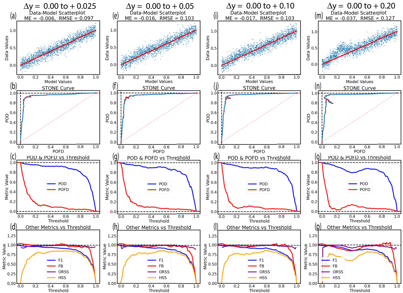
Figure 10. Same as Figure 9 but with a positive shift in three x -axis bins (between 0.1 and 0.4).
