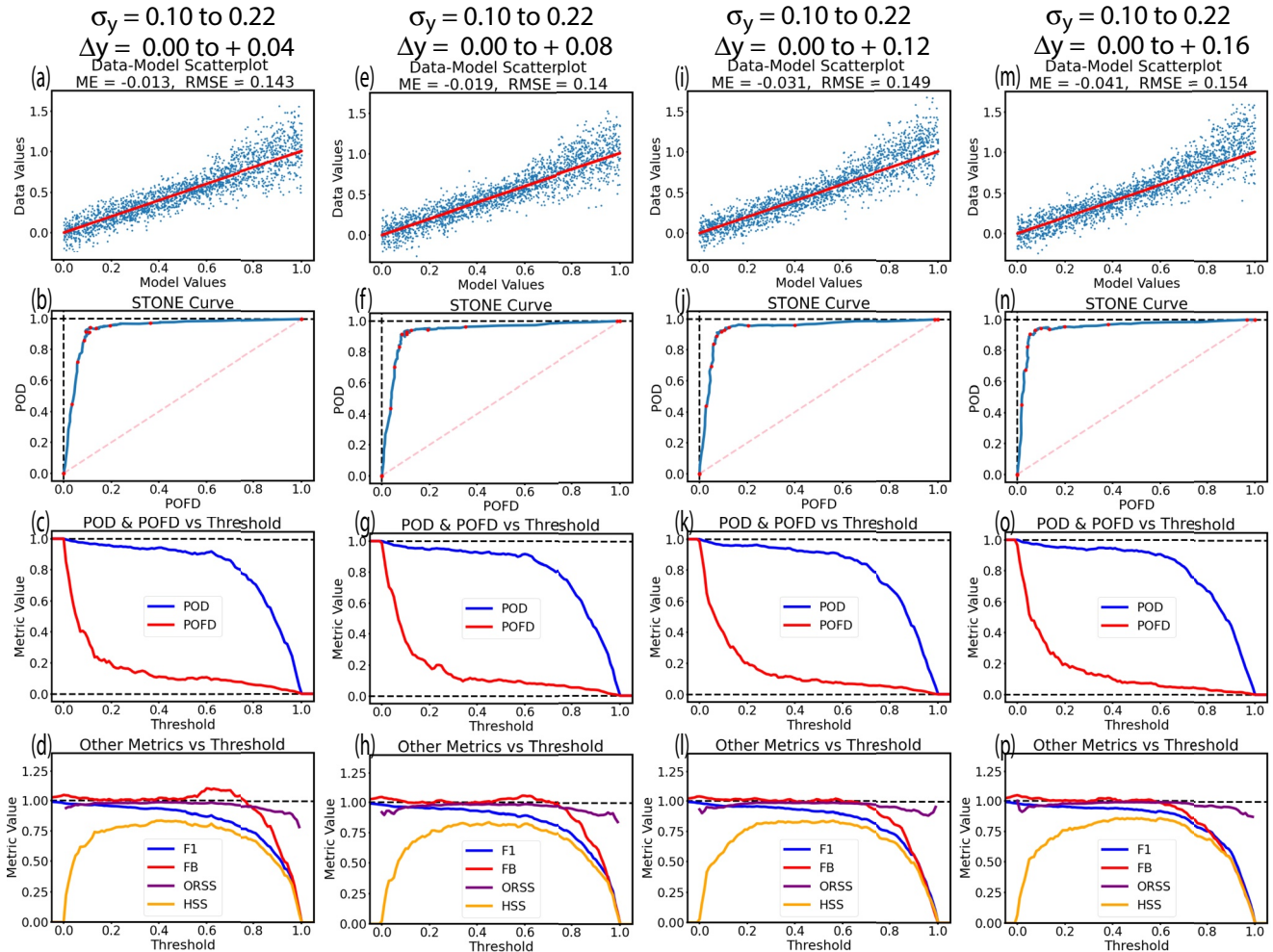
Figure 7. Same as Figure 6 except with positive shifts in the Gaussian peak relative to the unity slope line.
