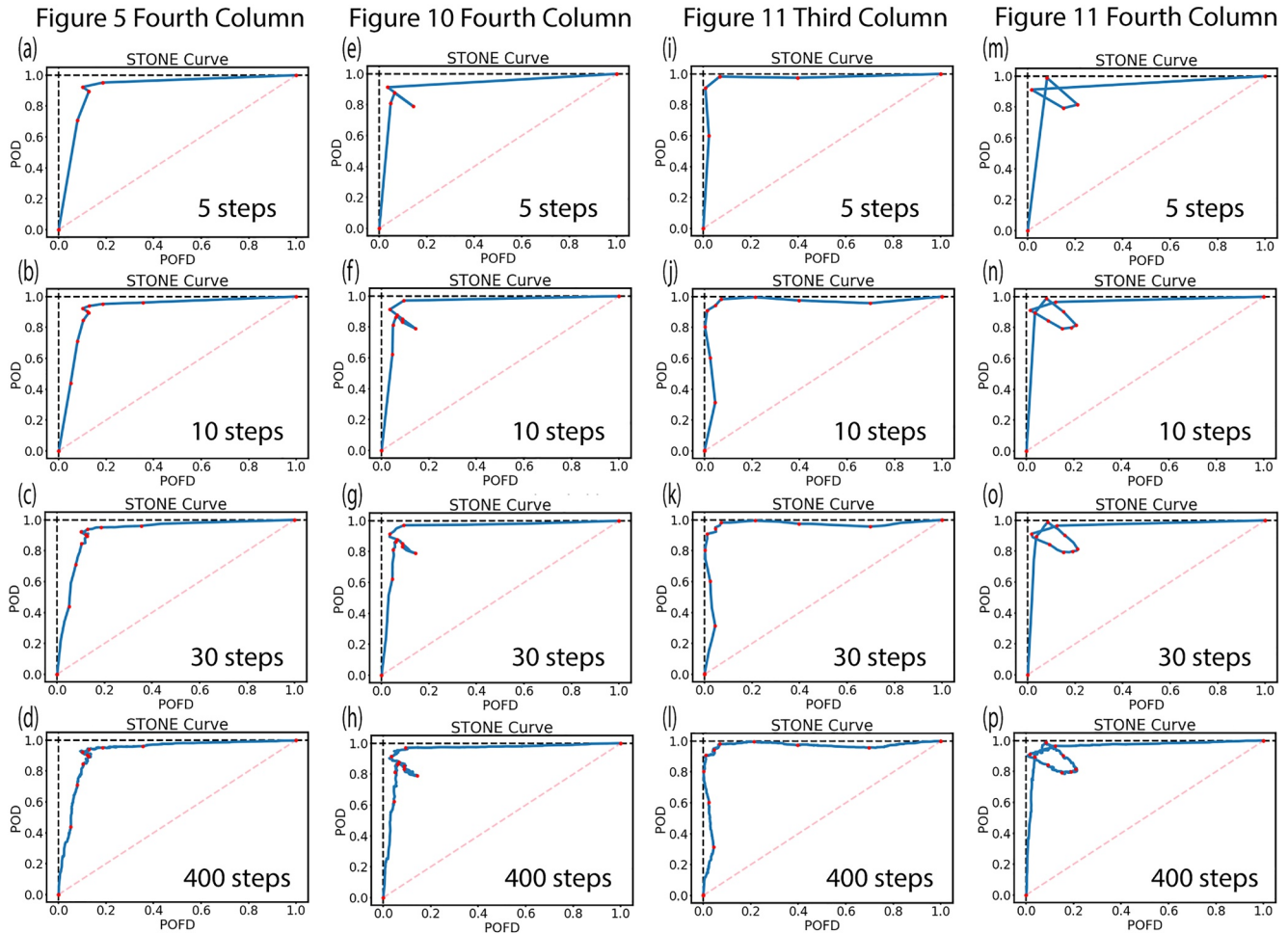
Figure 12. Changing the resolution of the threshold sweep when calculating the sliding threshold of observation for numeric evaluation (STONE) curve and other metrics. Four of the distributions from previous figures were used as indicated above each column. The original STONE curve above was conducted with 100 steps between 0 and 1; these STONE curves were created with a different number of steps in that interval: 5 for the top row, 10 for the second row, 30 for the third row, and 400 for the fourth row.
