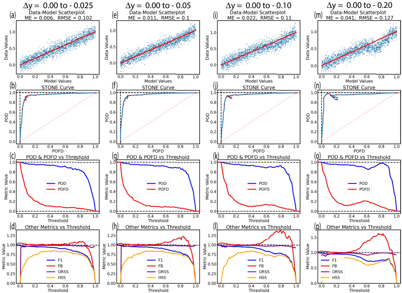
Figure 9. Same as Figure 4 but with a constant spread of 0.1 and a negatively shifting bias to the error distribution in three x -axis bins (between 0.6 and 0.9), two halfway, and the middle the full shift. From left to right, the maximum shifts are -0.025 , -0.05 , -0.10 , and -0.20 .
