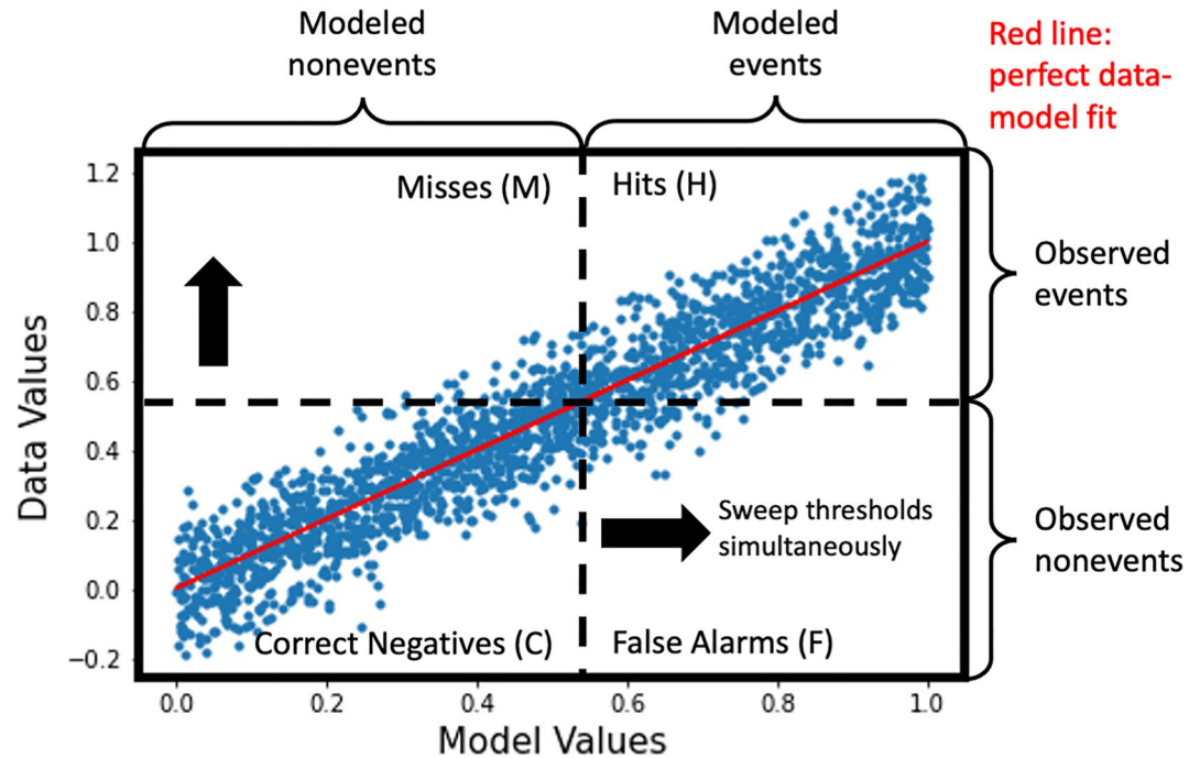
Figure 1. Data-versus-model scatterplot with event identification thresholds drawn. The arrows indicate the sweep conducted to generate a collection of contingency tables as a function of threshold setting, moving both thresholds simultaneously.
