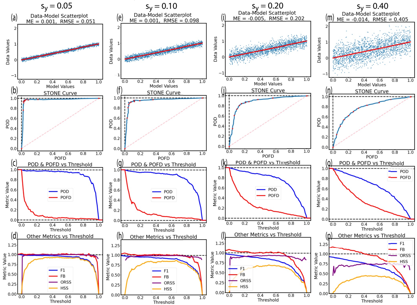
Figure 4. Scatterplots (top row), the corresponding sliding threshold of observation for numeric evaluation curves (second row), its underlying probability of detection and probability of false detection values as a function of threshold (third row), as well as several other metrics versus threshold (fourth row). The formats of the plots are identical to those in Figures 1 and 3. The four columns have data-model errors with Gaussian distributions with no offset but different spreads as indicated.
