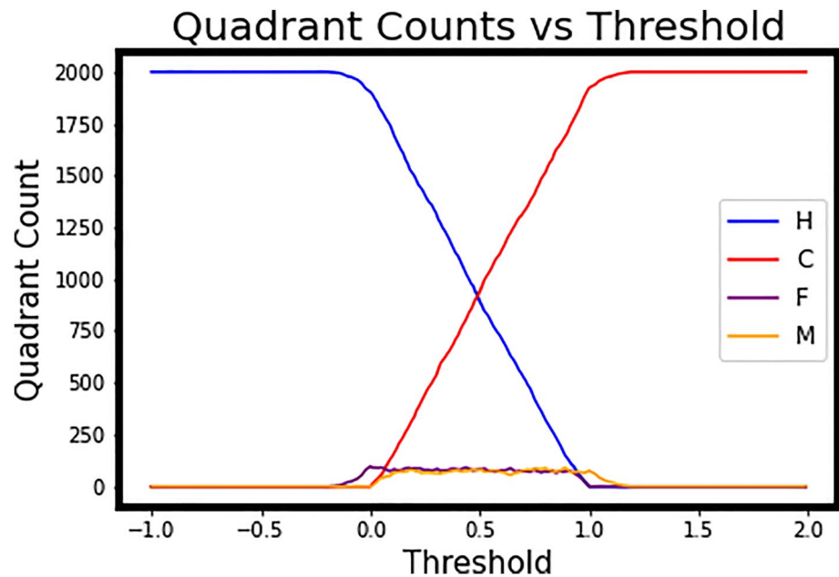
Figure 2. Quadrant counts for H, C, F, and M as a function of sweeping the data and model event identification thresholds simultaneously through the example scatterplot shown in Figure 1.
