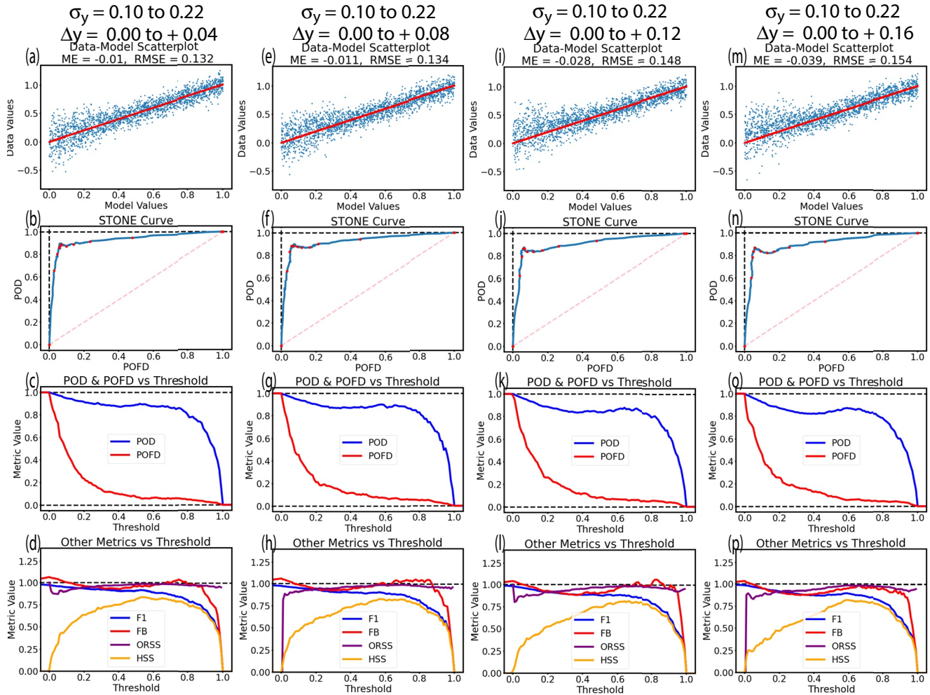
Figure 8. Same as Figure 6 except with the increasing spread and positive shift of the error distribution at low x value, below 0.4.
