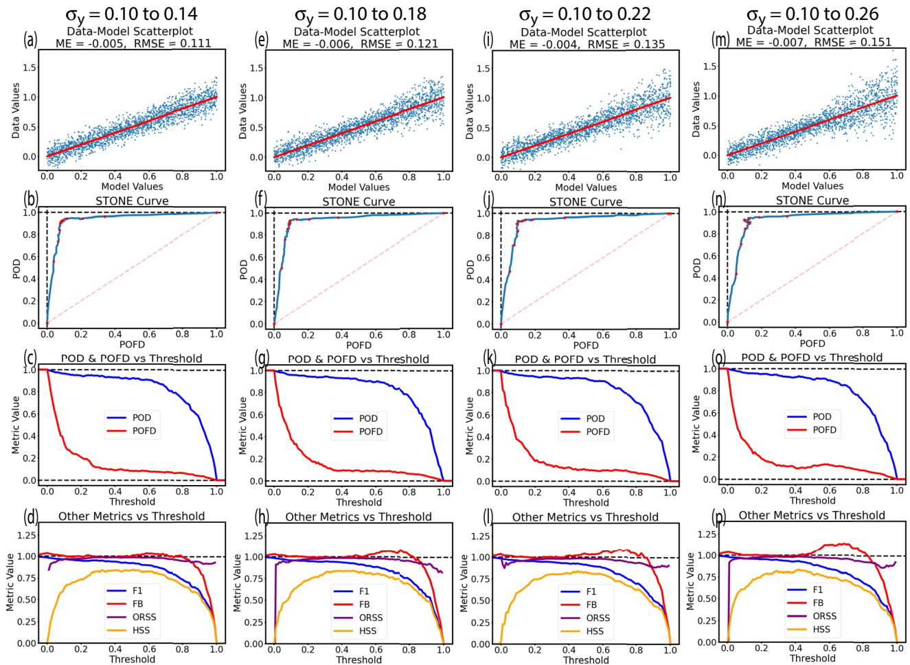
Figure 5. Same as Figure 4, but systematically varying the width of the distribution but only for x > 0.6 . All distributions have \sigma = 0.10 for x < 0.6 , then increase within each 0.1 interval by a given increment: left column by 0.01, second column by 0.02, third column by 0.03, and right column by 0.04.
