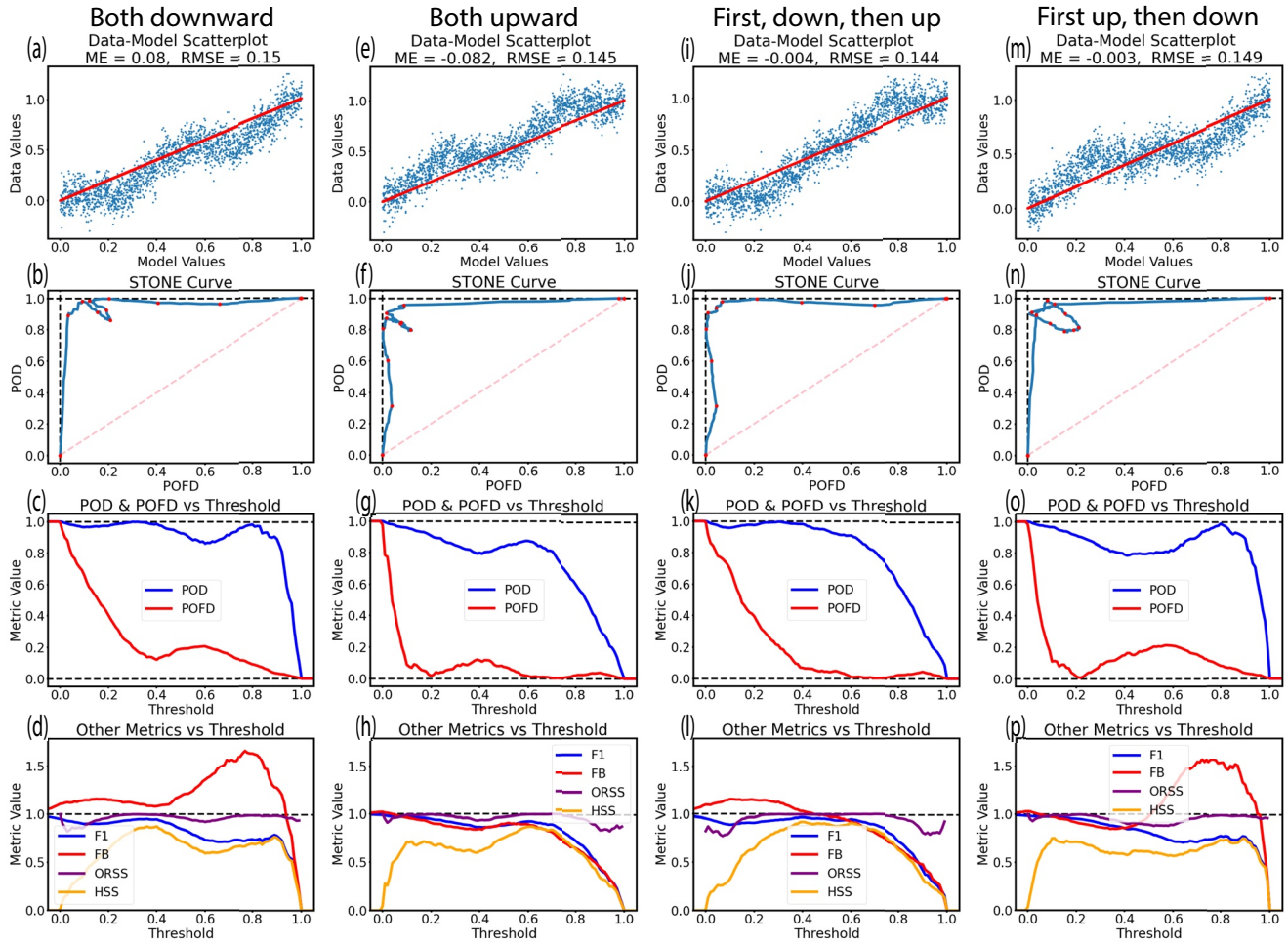
Figure 11. Same as Figure 9 but with two shifts in three x -axis bins (one between 0.1 and 0.4 and another between 0.6 and 0.9).
