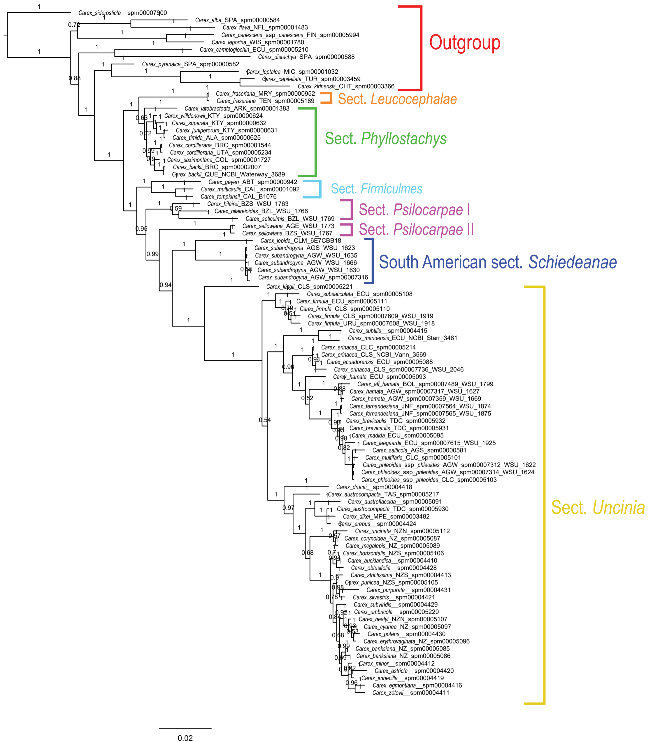
Fig. S9. Phylogenetic reconstruction based on the Bayesian inference analyses of the all-nrData dataset.
