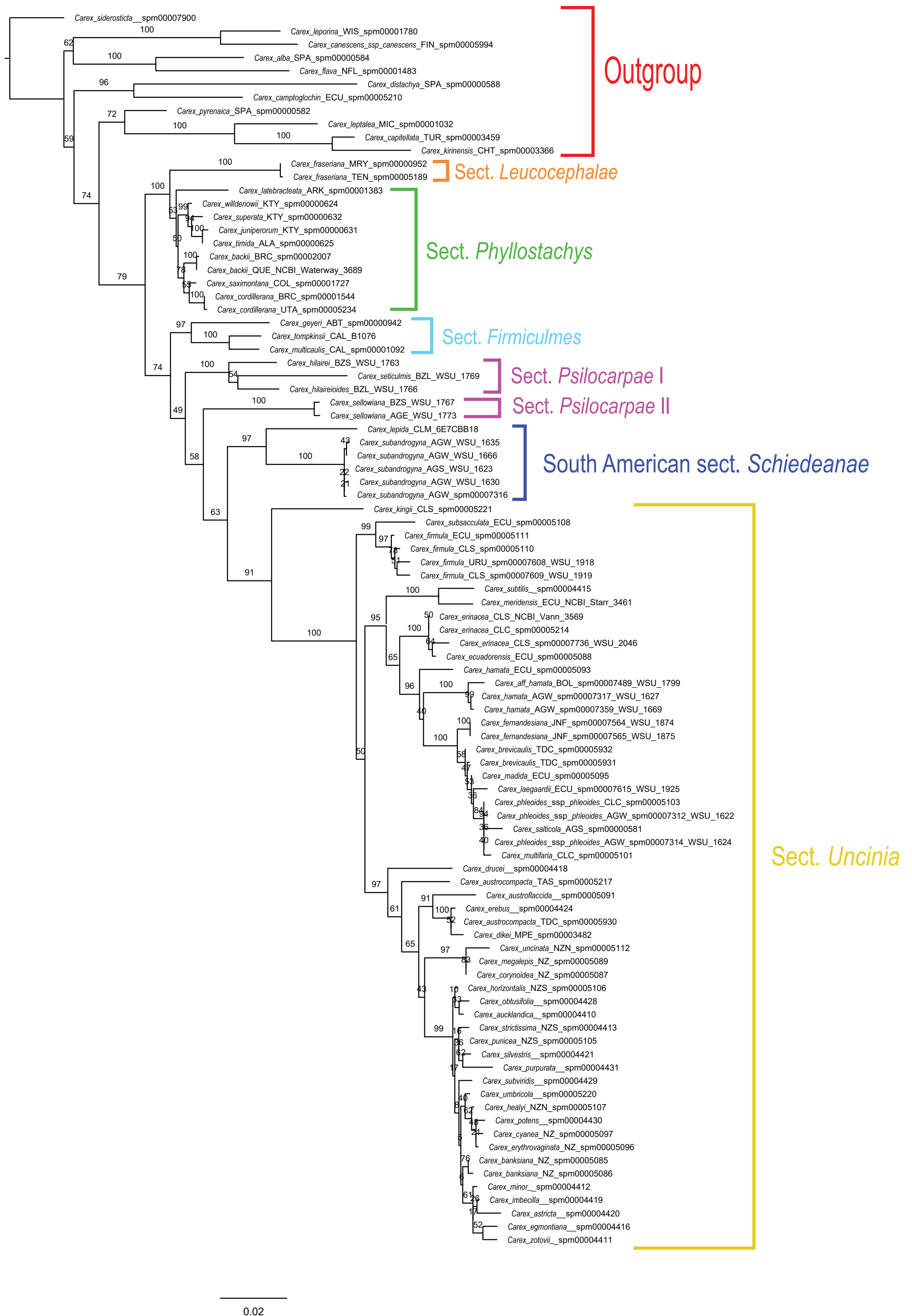
Fig. S10. Phylogenetic reconstruction based on the maximum likelihood analyses of the all-nrData dataset.
