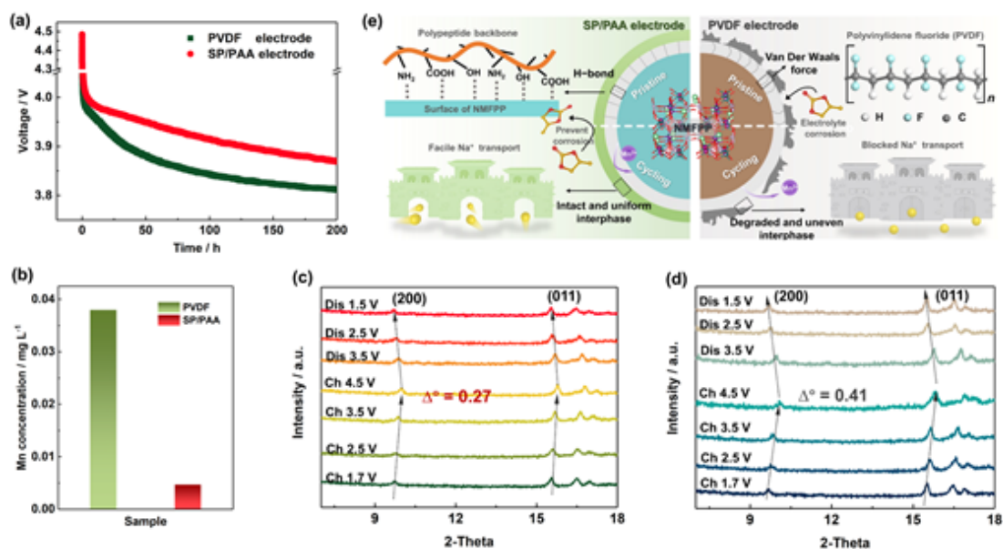
Figure 6. Stability of the electrodes. (a) Self-discharging tests of the two electrodes. (b) Mn concentration of the electrolytes determined by ICP. (c) Ex-situ XRD of the SP/PAA electrodes. (d) Ex-situ XRD of the PVDF electrodes. (e) Schematic illustration of the features and functions of SP/PAA and PVDF binders.
