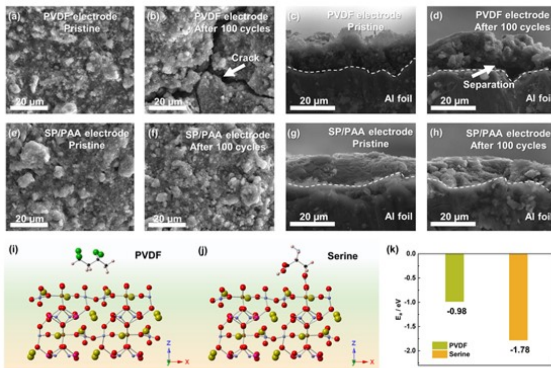
Figure 4. Integrity of the electrodes. (a) SEM images of the pristine and (b) after 100 cycles of the PVDF electrodes. (c,d) The corresponding cross-sections of the PVDF electrodes. (e) SEM images of the pristine and (f) after 100 cycles of the SP/PAA electrodes. (g,h) The corresponding cross-sections of the SP/PAA electrodes. (i) Adsorption configurations of PVDF and (j) serine on the Na 4 Mn 2 Fe(PO 4 ) 2 P 2 O 7 (001) crystal plane. Red, green, black, pink, blue, purple, brown, rosy and yellow spheres represent O, F, C, H, N, P, Fe, Mn, and Na atoms, respectively. (k) The calculated adsorption energy.
