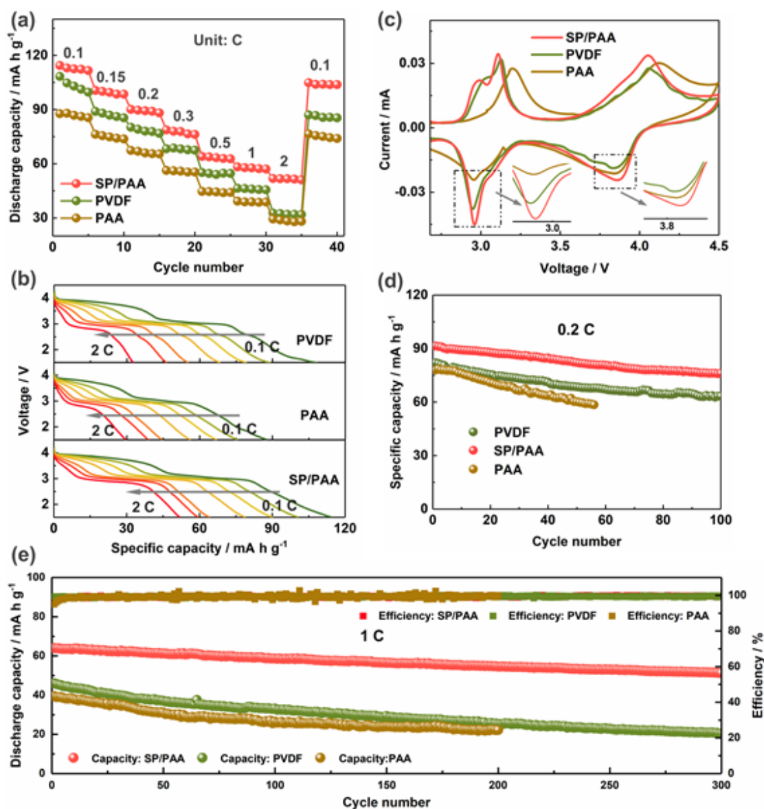
Figure 2. Electrochemical performance of NMFPP electrodes made up from different binders. (a) Rate performance of the electrodes from 0.1 C to 2 C. (b) The corresponded
