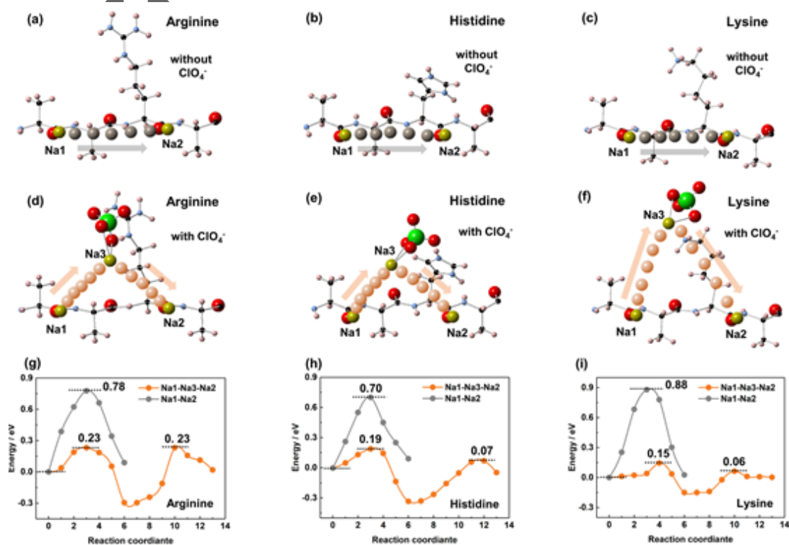
Figure 3. DFT calculations disclose the effect of SP on the enhanced sodium storage performance. \text{Na}^+ -ions diffusion paths in (a) arginine, (b) histidine, and (c) lysine that without the \text{ClO}_4^- . \text{Na}^+ -ions diffusion paths in (d) arginine, (e) histidine, and (f) lysine that with the existence of \text{ClO}_4^- . The sodium diffusion energy barriers in (g) arginine, (h) histidine, and (i) lysine.
