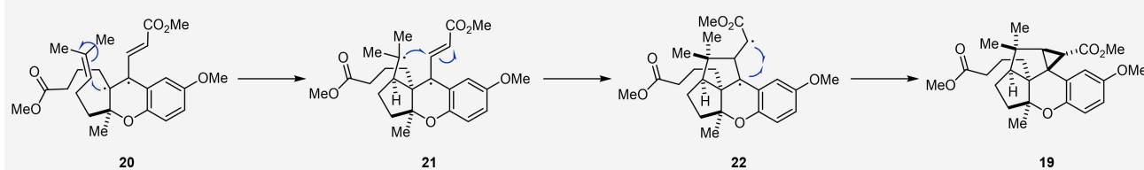
Scheme 3. Challenges observed in developing a Catellani and subsequent [2+2] cycloaddition approach towards cochlearol B ( 2 ).
