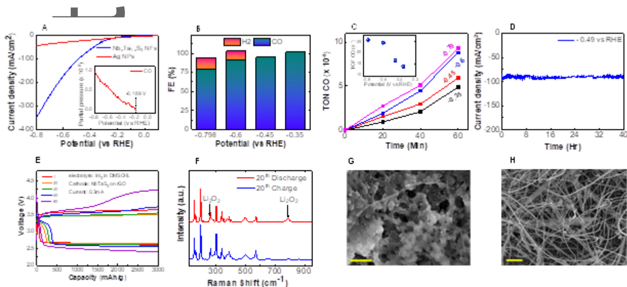
Figure 4. Electrochemical CO 2 conversion and Li-air battery experiments using Nb 1-x Ta x S 3 nanofibers-based cathodes. (A) CV test at 50mV/s scan rate for Ag nanoparticles (red) and NbTaS 3 nanofibers (Blue). The inset shows the onset potential of CO production measured by online DEMS at a scan rate of 1 mV/sec. (B) Faradic efficiency (FE) towards production of CO and H 2 from CA experiments at four different potentials. (C) Turnover number over an hour of CA experiments showing the activity of NbTaS 3 catalyst with the TOF in the inset. (D) Catalyst stability test over 40 hours at the potential of -0.49 V vs RHE. (E) Li-air battery cycling performance utilizing Nb x Ta 1-x S 3 catalyst. (F) Raman spectroscopy of the cathode after 20 th discharge and charge cycle. SEM image of the cathode surface after (G) 20 th discharge and (H) 20 th charge cycle (scale bars: 1 μm).
