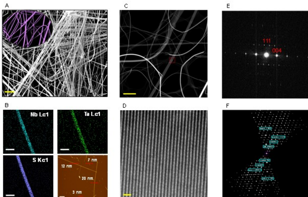
Figure 1. Summary of characterization of 1D-Nb 1-x Ta x S 3 alloy. (A) SEM image of long belt-like Nb 1-x Ta x S 3 nanofibers (scale bar: 50 μm). (B) SEM-EDX elemental maps obtained from individual fibers (scale bar: 2 μm) and a typical AFM topography image of bath-sonicated fibers with the heights of 3 to 20 nm (scale bar: 5 μm). (C) HAADF STEM image of the Nb 1-x Ta x S 3 nanofibers (scale bar: 200 nm). (D) High-resolution HAADF STEM image of the nanofiber viewed along the [110] direction, showing clear lattice fringes (scale bar: 1 nm). (E) Fourier transforms of the image. (F) 2D slice cuts from the reconstructed 3D reciprocal lattice show the h0l plane. Diffused scattering can be observed in the data, which indicates disordered structure of Nb 1-x Ta x S 3 nanofibers.
