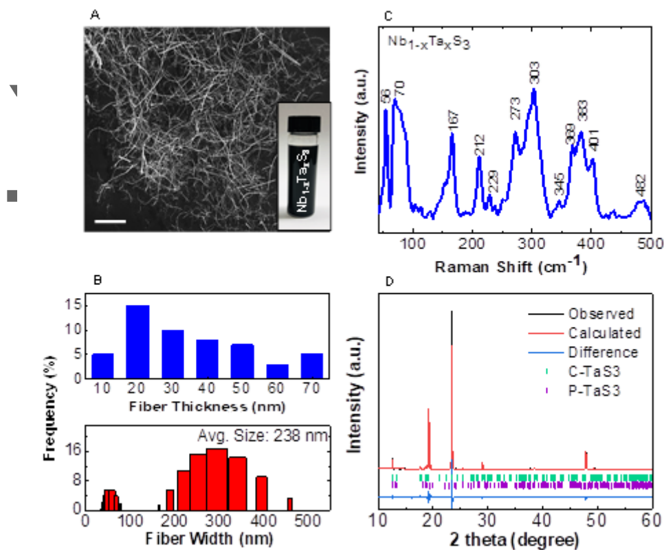
Figure 2. Summary of characterization of 1D-Nb 1-x Ta x S 3 nanofibers. (A) SEM image of drop casted solution on Si Substrate (scale bar: 5 μm). Inset shows dispersions of exfoliated Nb 1-x Ta x S 3 nanofibers in IPA solvent. (B) AFM frequency distribution obtained from ~50 randomly selected exfoliated fibers and size distribution from DLS measurements for Nb 1-x Ta x S 3 alloy. (C) Raman characteristics of TMTC alloy at ambient conditions excited by 633 nm laser. (D) Pawley refinement of the XRD patterns obtained from 1D-Nb 1-x Ta x S 3 nanofibers.
