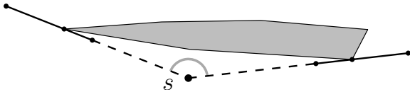
Figure 3: To show there are no separating 2-cycles, note that any convex obstacle subtends an arc of < \pi radians.
