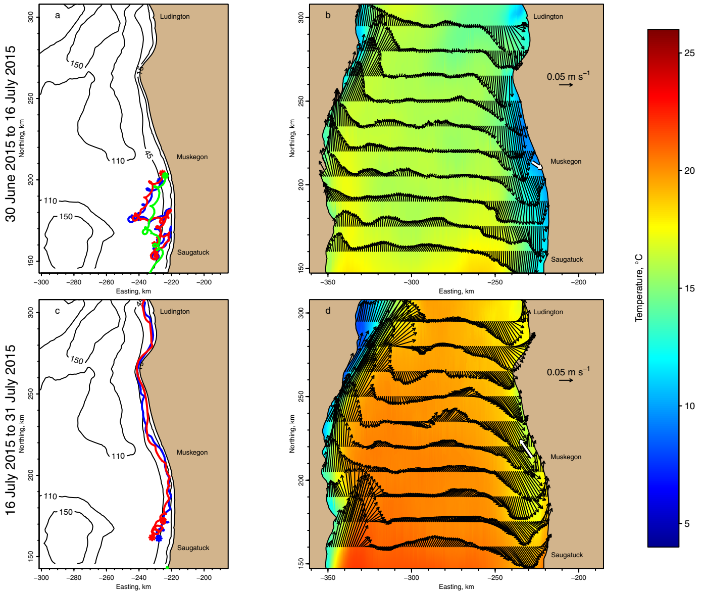
Fig. 7. 2015 Drifter trajectories, model currents and surface temperature, divided into periods of upwelling (a,b) and downwelling (c,d). Other symbols are explained in Fig. 4.
