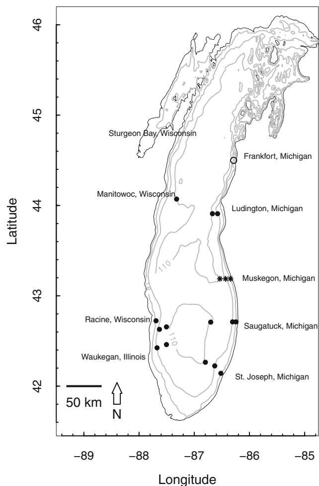
Fig. 1. Map of Lake Michigan, with bathymetry contours (15, 45, and 110 m), and port cities in the U.S. states of Michigan (MI), Wisconsin (WI), and Illinois (IL). Locations of larval alewife collections (solid circles), and drifter deployment stations located at 15, 45, and 110-m depth offshore of Muskegon (asterisks; M15, M45, M110) are indicated. Stations offshore of Sturgeon Bay and Frankfort were sampled, but no larval alewife were collected.
