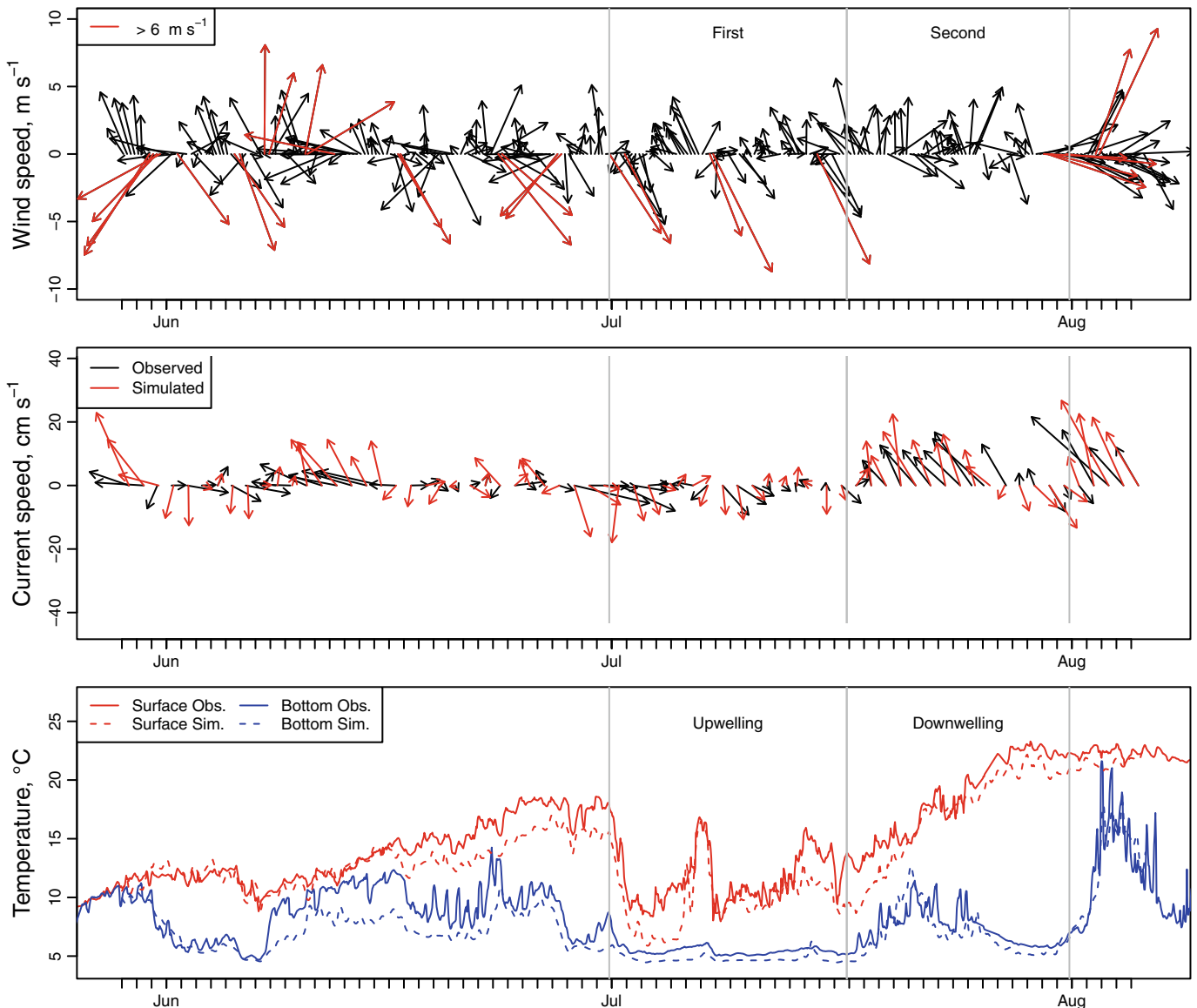
Fig. 4. Observed wind, currents, surface and bottom temperature at the M15 station (Fig. 1) during the first, second, and 3 rd 2015 drifter deployments. Symbols are explained in Fig. 3 caption.
