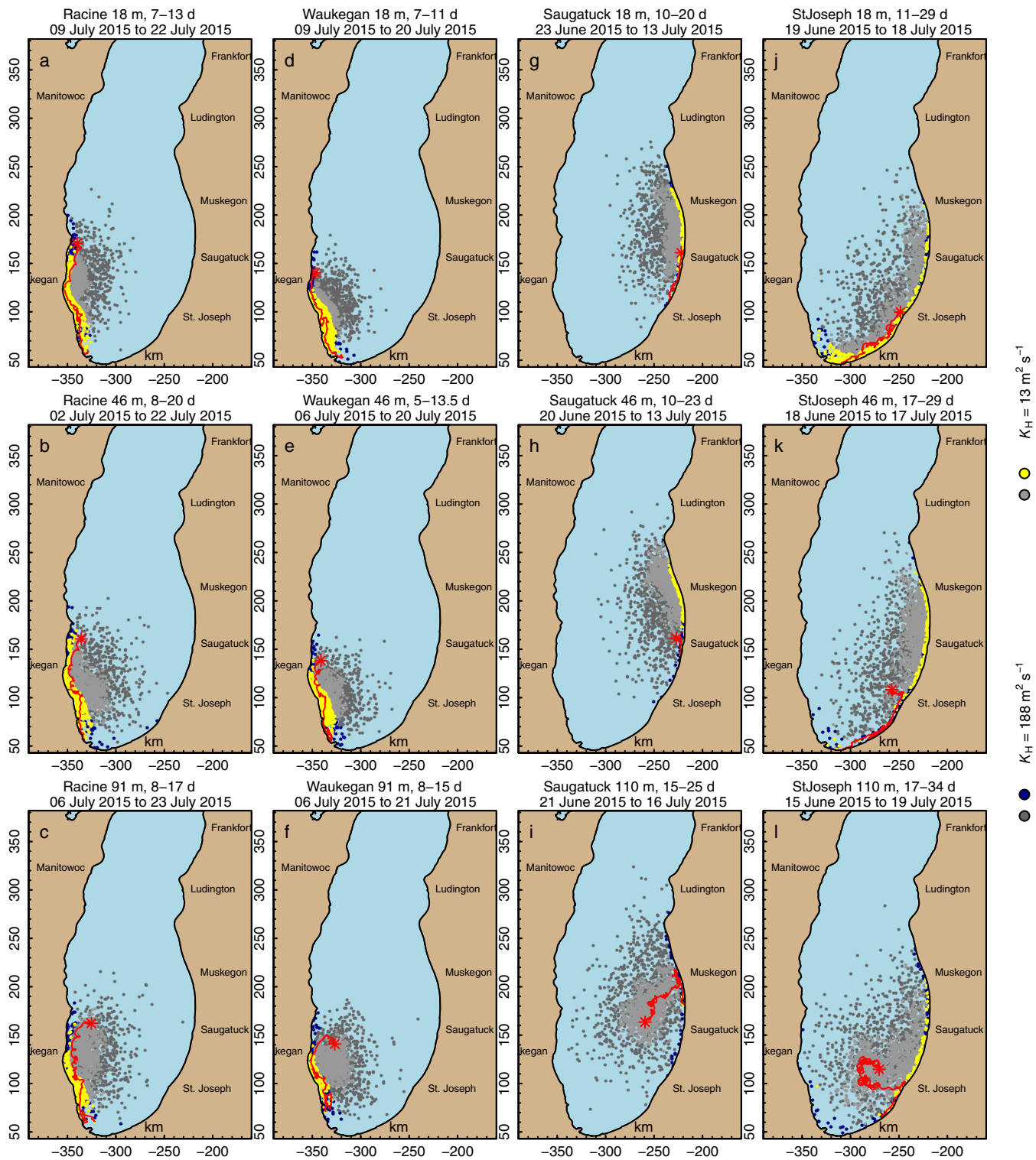
Fig. 10. Predicted origins of alewife larvae in southern Lake Michigan using two scenarios of horizontal diffusivity, K_H = 13 \text{ m}^2 \text{ s}^{-1} (yellow) and 188 \text{ m}^2 \text{ s}^{-1} (navy blue), within a range of depths that were plausible for spawning ( < 20 \text{ m} bottom depth). Gray areas indicate estimated origin locations in deep water, not likely to be spawning areas. Backward trajectory simulations began at the site of field collection (red asterisk) and ran for the duration of the oldest age larva collected in that sample, with the range of ages indicated above each panel. The red line illustrates one example from the ensemble of model backward trajectories, over the date range indicated above each panel.
