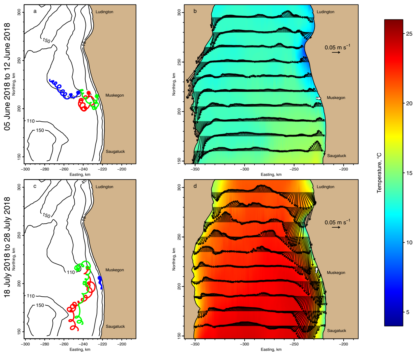
Fig. 5. 2018 Satellite-tracked drifter buoy trajectories, model currents, and surface temperature for upwelling periods (Fig. 3) offshore of Muskegon. The observed surface current vector at the Muskegon ADCP averaged over the period is indicated by a white arrow with black outline. Model currents are plotted at 1 km spacing in easting and 15 km spacing in northing to visualize coastal currents.
