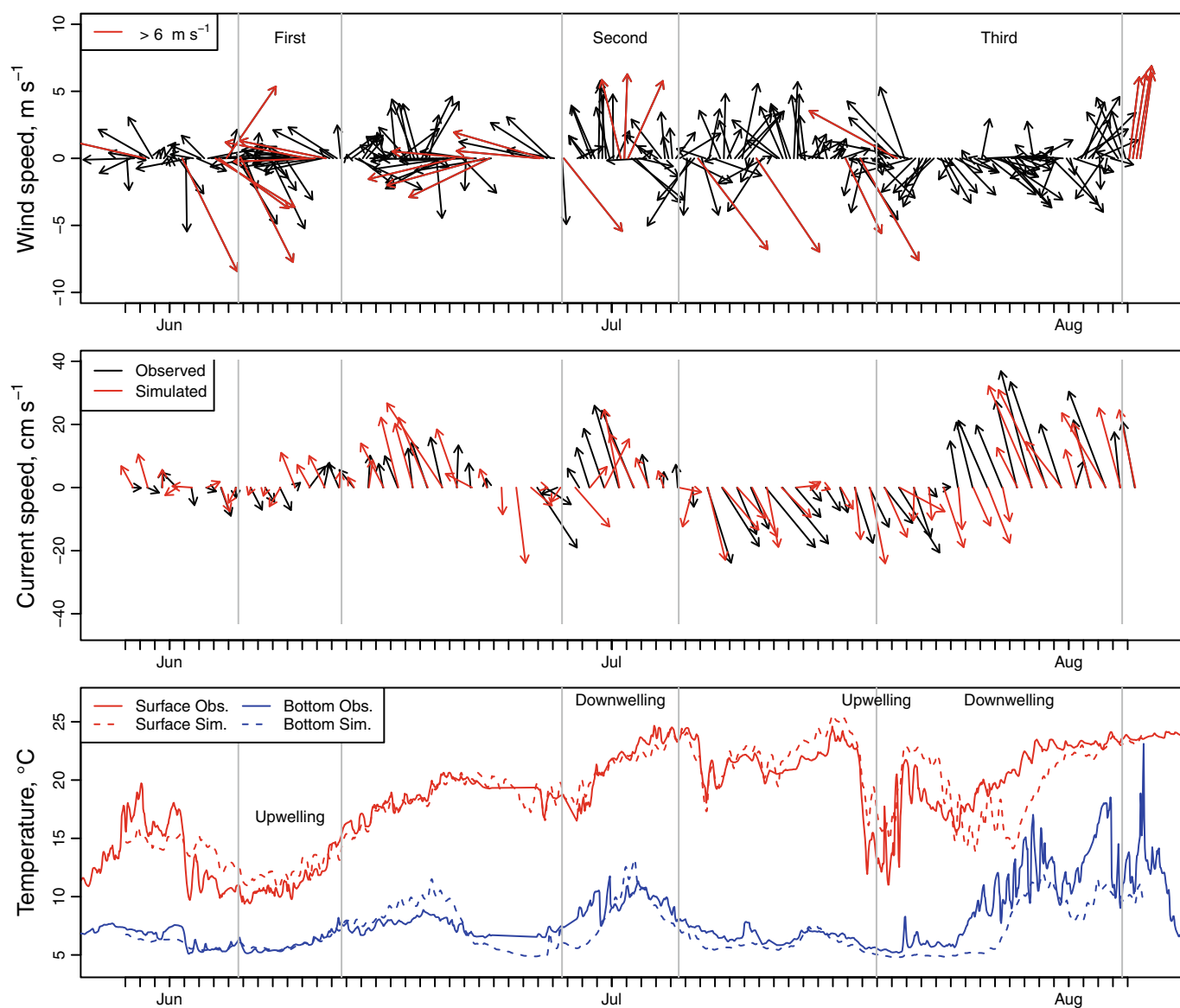
Fig. 3. Observed wind, currents, surface and bottom temperature at the Muskegon M15 station (Fig. 1) during the first, second, and 3 rd 2018 drifter deployments, with periods of upwelling and downwelling indicated. Wind and currents are averaged over 6 h. Wind vector arrows highlighted in red were > 6 \text{ m s}^{-1} speed. FVCOM model simulated currents and temperatures are plotted along with observations.
