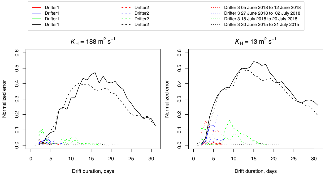
Fig. 9. Model skill in predicting possible drifter buoy origins for the backward trajectory simulations in Fig. 8, given as the minimum distance between the observed drifter position and the spatial patch of likely drifter origin locations (nearest Lagrangian particle). The two panels give results for the two scenarios of horizontal diffusivity ( K_H = 13 and 188 \text{ m}^2 \text{ s}^{-1} ). Line color indicates the deployment period, given in the legend, while each individual drifter within a deployment period is shown with a different line type (solid, dashed, dotted).
