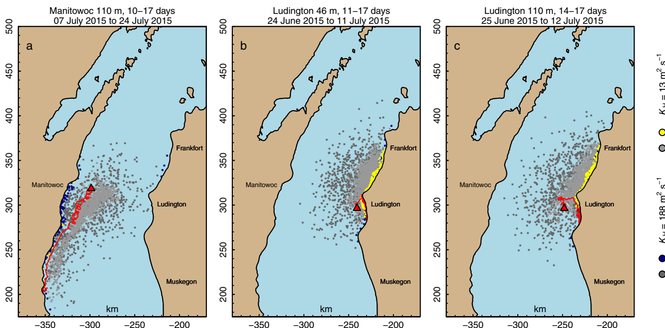
Fig. 11. Predicted origins of alewife larvae in northern Lake Michigan using two scenarios of horizontal diffusivity, K_H = 13 \text{ m}^2 \text{ s}^{-1} (yellow) and 188 \text{ m}^2 \text{ s}^{-1} (navy blue), within a range of depths that were plausible for spawning ( < 20 \text{ m} bottom depth). Gray areas indicate estimated origin locations in deep water, not likely to be spawning areas. Backward trajectory simulations began at the site of field collection (red asterisk) and ran for the duration of the oldest age larva collected in that sample, with the range of ages indicated above each panel. The red line illustrates one example from the ensemble of model backward trajectories, over the date range indicated above each panel.
