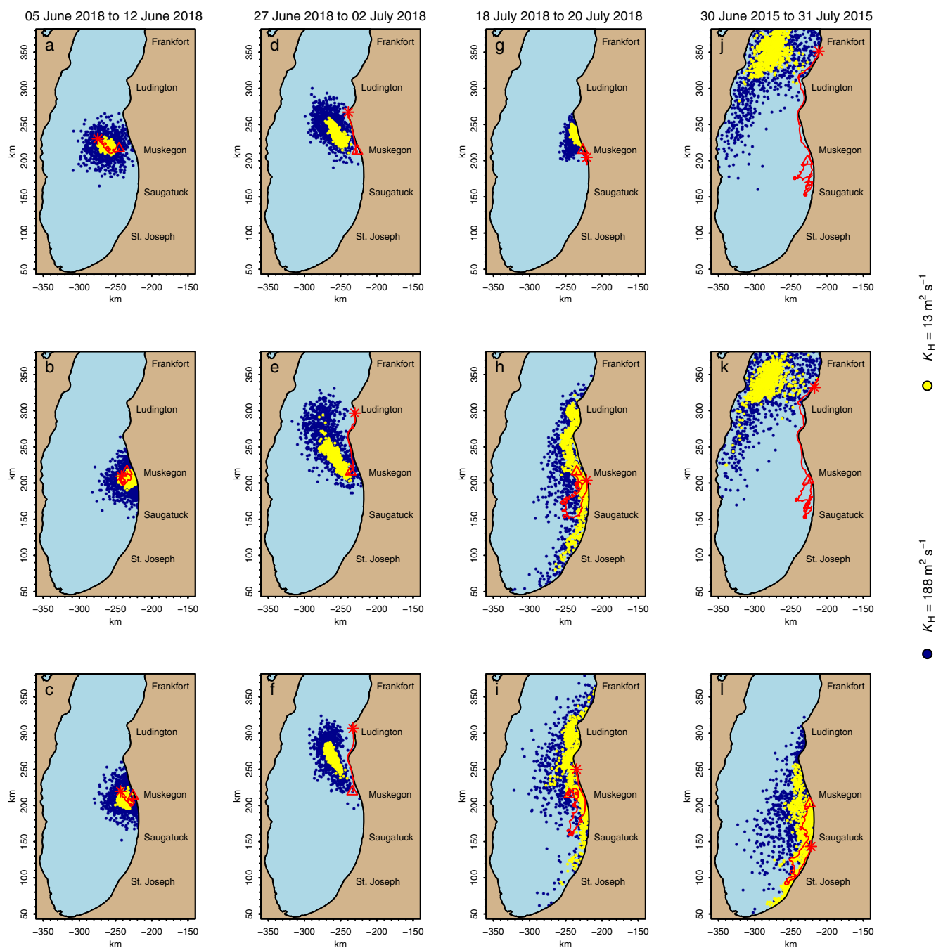
Fig. 8. Prediction of the origin of satellite-tracked drifter buoys from their final position and drift duration using backward trajectory simulations. The model-predicted drifter origin is given as a spatial patch represented by colored points indicating two scenarios of horizontal diffusivity: K_H = 13 \text{ m}^2 \text{ s}^{-1} (yellow) and 188 \text{ m}^2 \text{ s}^{-1} (navy blue). The observed drifter origin, track, and final location are shown by a red triangle, solid line, and asterisk, respectively.
