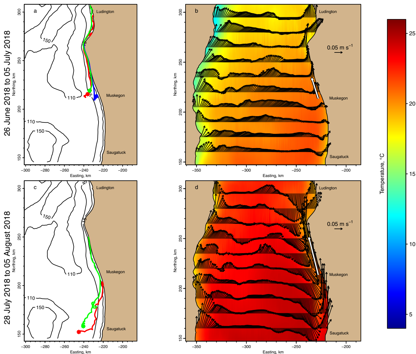
Fig. 6. 2018 Drifter trajectories, model currents, and surface temperature for downwelling periods (Fig. 3) offshore of Muskegon. Other symbols are explained in Fig. 4.
