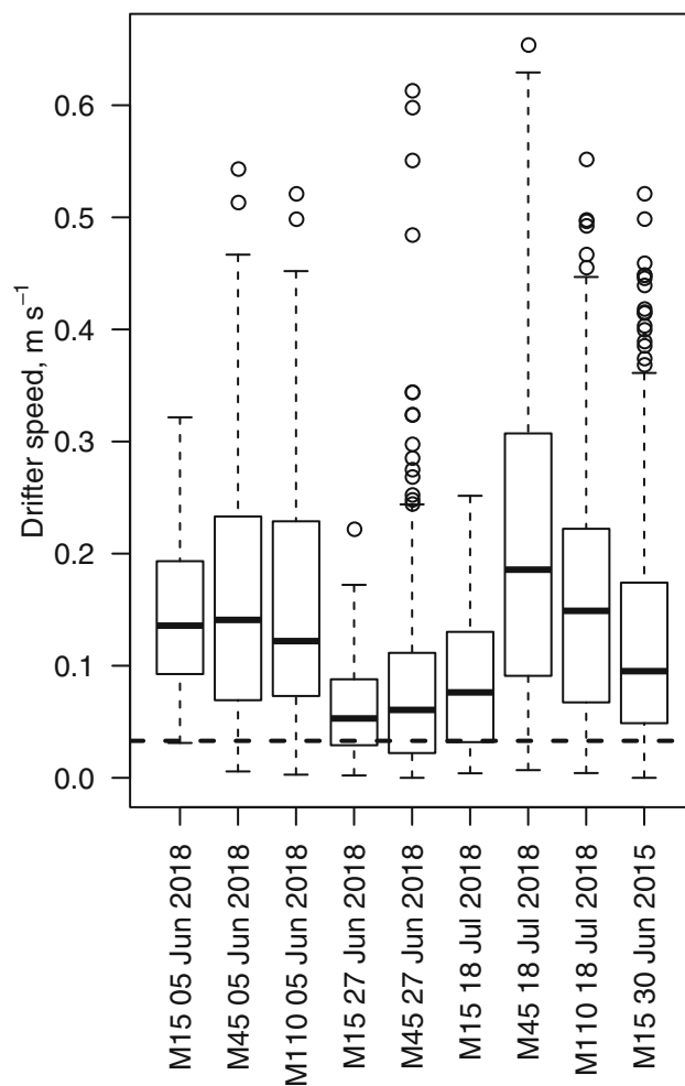
Fig. 2. Drifting speeds recorded by satellite-tracked drifting buoys deployed at stations offshore of Muskegon, MI (Fig. 1), in June and July of 2015 and 2018. The horizontal dashed line indicates an estimate of larval alewife swimming speed (see “Discussion” section). Box plots indicate the median and interquartile range, with whiskers extending to the most extreme value within 1.5 times the interquartile range, and circles indicating values outside the range of the whiskers.
