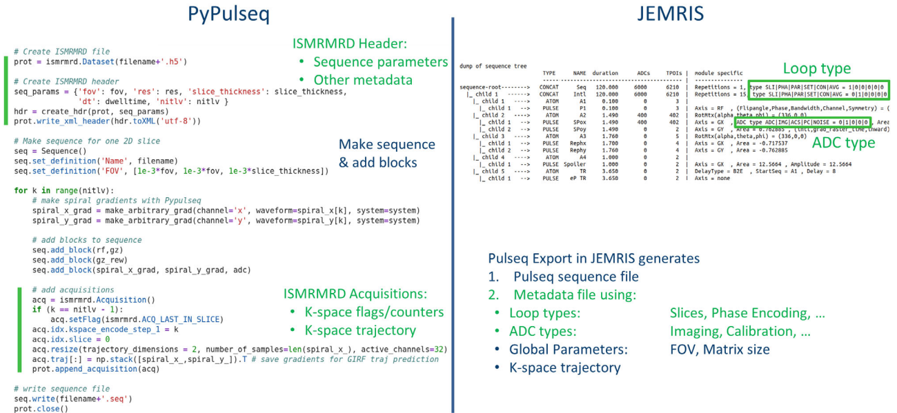
FIGURE 2 Left: Sequence development and metadata file creation with PyPulseq. The metadata file is initialized, and a header is created from global sequence parameters (full header function not shown). The sequence object is created, and event blocks are added. At the same time, readout information such as k-space flags, counters, and the k-space trajectory are added to the metadata file. Right: Dump of the sequence tree from a sequence developed with the JEMRIS simulation framework. The metadata header is generated from the global parameters in JEMRIS. Acquisition-specific k-space information is generated from the new JEMRIS loop-type and ADC-type parameters and added to the metadata, together with the k-space trajectory. Green color indicates new features.
