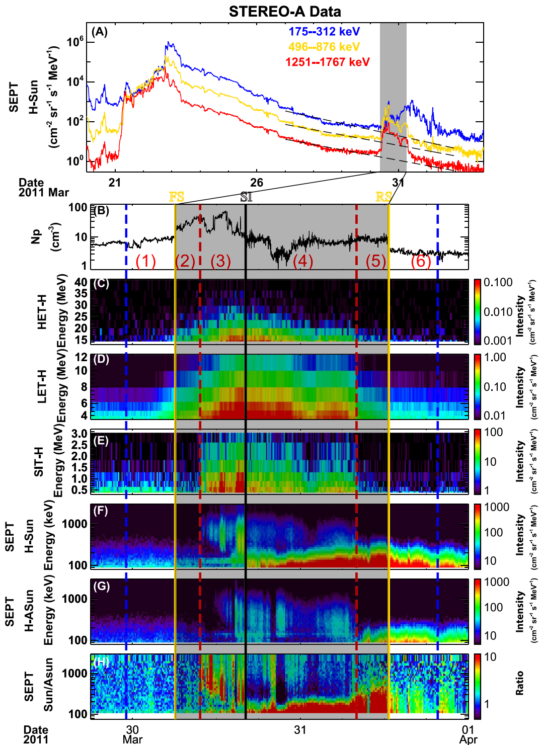
Figure 1. Overview of the SIR event. Panel (a) shows the ion intensities in three energy bands measured by the sunward telescope of SEPT instrument between 2011 March 20–2011 April 3. The shaded region indicates the stream interaction region (SIR). The three dashed lines exhibit the expected intensities in the SIR and beyond. Panel (b) shows the solar wind proton number density. From panel (c) to panel (g), the ion intensities measured by the HET, LET, SIT, the sunward and anti-sunward telescopes of SEPT are presented, respectively, and the unit of the differential fluxes is \text{cm}^{-2} \text{sr}^{-1} \text{s}^{-1} \text{MeV}^{-1} . The bottom panel (h) presents the intensity anisotropies of the ions observed by the sunward and the anti-sunward telescopes of SEPT. The shaded regions mark the SIR, with the gold vertical lines showing the boundaries, which are forward shock (FS) and reverse shock (RS). The black vertical line indicates the stream interface (SI). The blue (23:06 UT on March 29 and 08:02 UT on March 31) and red (09:40 UT on March 30 and 19:37 UT on March 31) vertical dashed lines mark four boundaries of the targeted regions, see details in the text. The colors in panels (c) to (g) indicate the ion intensities, and the colors in the last panel mean the ratios of the sunward to the anti-sunward intensities.
