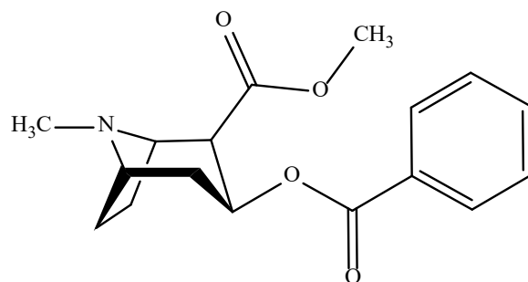
FIGURE 1. Chemical structure of cocaine
