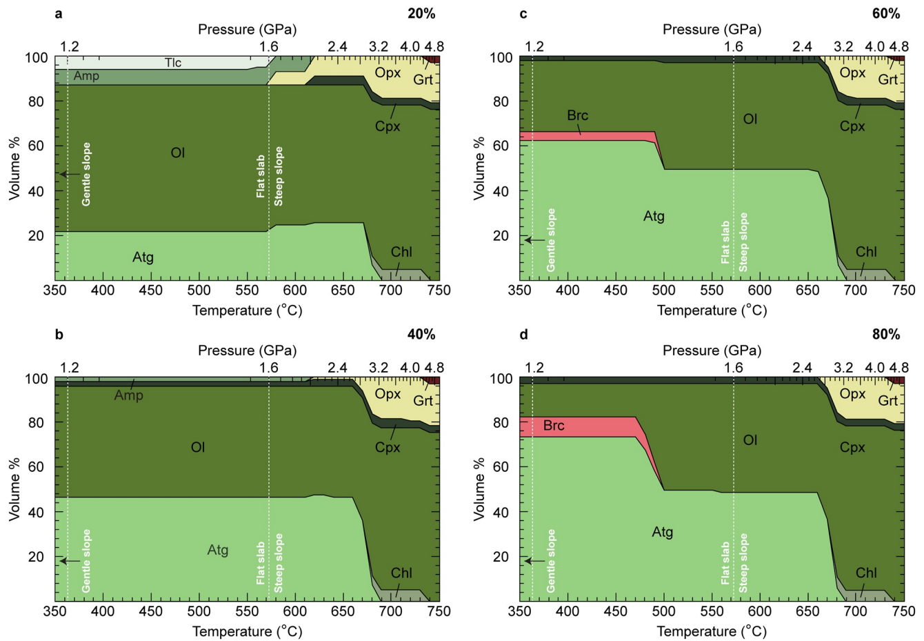
Figure 4. The effect of different degrees of hydration for harzburgite during subduction. Calculated mineral assemblages along the Guerrero geotherm at (a) 20%, (b) 40%, (c) 60%, and (d) 80% of hydration.
