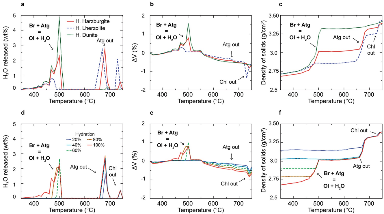
Figure 3. Petrophysical properties of the subducted oceanic Cocos plate. (a) H_2O released, (b) \Delta V_r (solids + fluid), and (c) density of solids evolution during subduction of the hydrated ultramafic portion of the Cocos oceanic lithospheric mantle. (d–e) Effects of different degrees of hydration (of a harzburgite) on (d) H_2O released, (e) \Delta V_r (solids + fluid), and (f) density.
