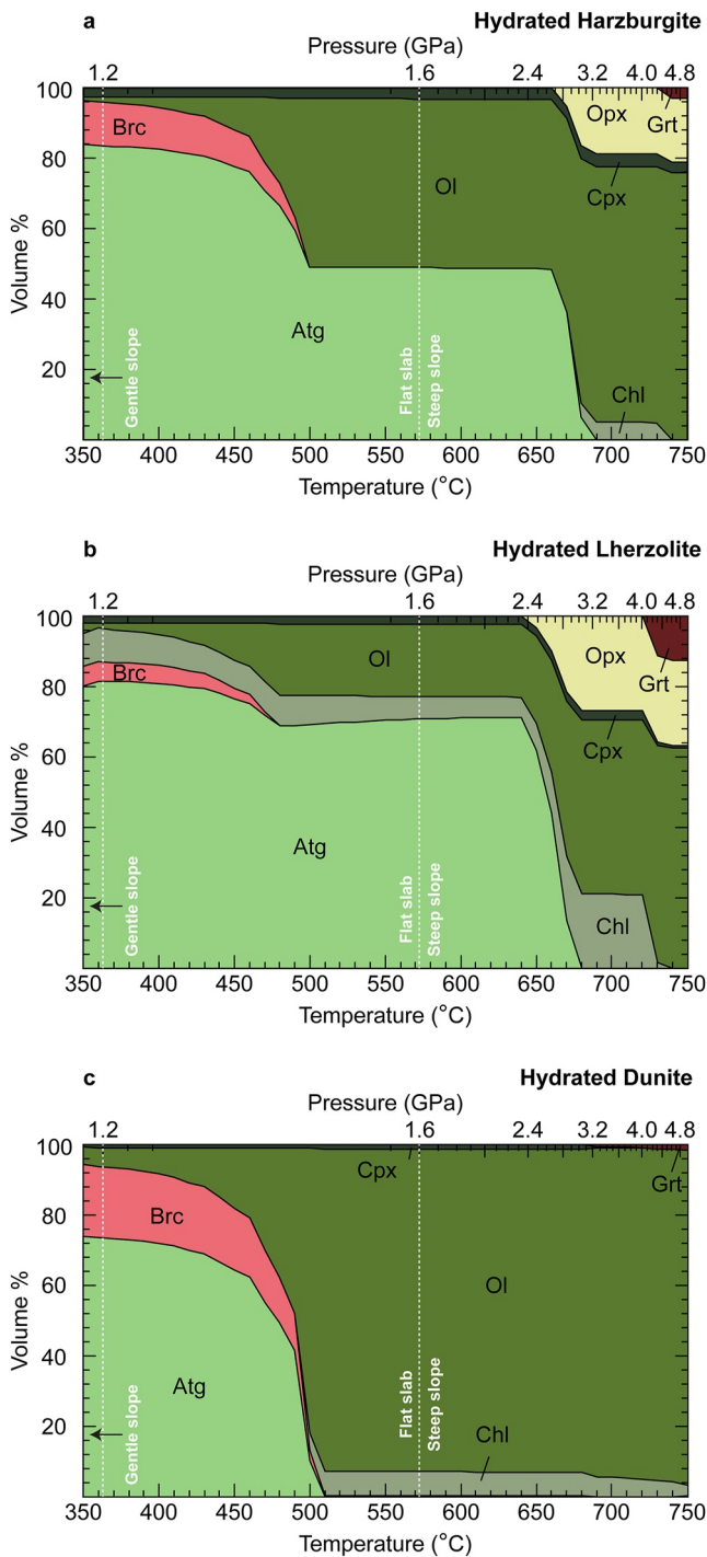
Figure 2. Equilibrium mineral assemblages along the Guerrero geotherm. (a–c) Mineral proportions for hydrated harzburgite, lherzolite, and dunite, respectively. Brucite is completely consumed regardless of the modeled composition at 480–500°C and ~1.5 GPa along the flat slab segment. The gentle slope, flat slab, and steep slope refer to the areas of the slab as shown in Figure 1. Brc–brucite; Atg–antigorite; Ol–olivine; Opx–orthopyroxene; Cpx–clinopyroxene; Grt–garnet; Chl–chlorite.
