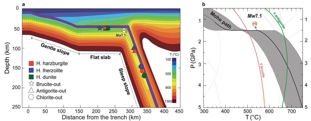
Figure 5. Thermal model and location of the dehydration reactions of the subducted oceanic Cocos plate. (a) Thermal model for central Mexico (Manea & Manea, 2011) showing the location and focal mechanism of the 2017 Puebla-Morelos earthquake, and the position of brucite, antigorite, and chlorite dewatering (at Moho depths). (b) Summarized P – T diagram for a hydrated harzburgite with the stability of brucite and antigorite, and the P – T path with its uncertainties of \pm 75^\circ\text{C} (the gray shaded areas; see also Figure S1 in Supporting Information S1).
