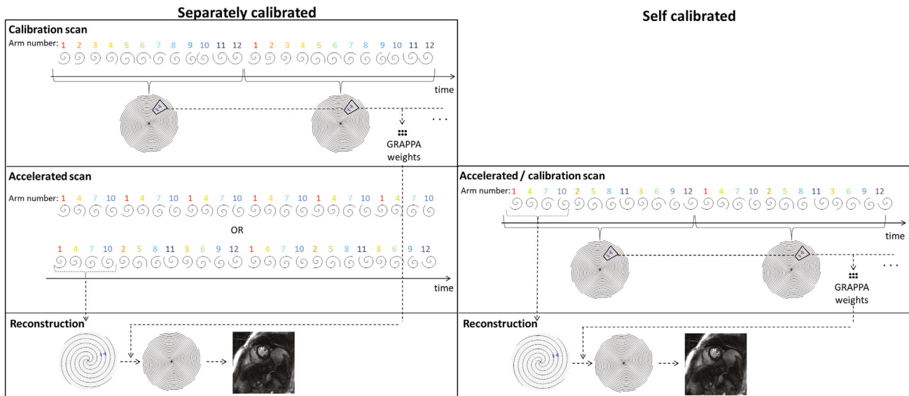
FIGURE 1 Schematic of separately-calibrated and the proposed self-calibrated through-time spiral GRAPPA acquisition. In the original implementation of through-time spiral GRAPPA, fully-sampled calibration data are acquired in a separate scan from the accelerated data (left). In the proposed self-calibrated implementation, accelerated data are acquired in an interleaved manner, and consecutive frames are merged to form fully-sampled calibration data (right)
