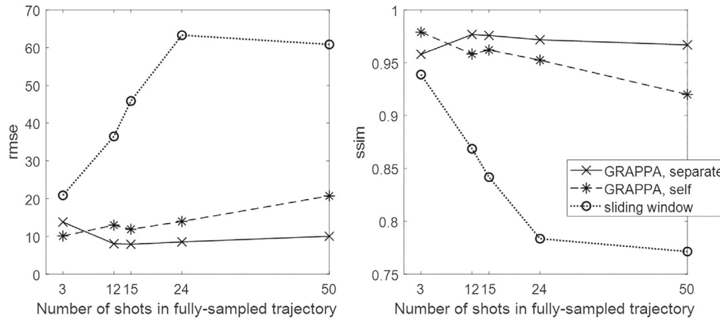
FIGURE 3 Comparison of sample trajectories tested in digital phantom simulations. The trajectories differ in the number of arms in the fully-sampled k-space, and thus both the TR and the time elapsed over the GRAPPA calibration kernel in separately and self-calibrated modes. The acceleration factor was chosen such that the temporal resolution per accelerated frame is <45 ms, as recommended for evaluation of LV structure and function. 21,22 Please see Supporting Information Table S1 for the kernel durations and acceleration factors of these trajectories. RMSE and SSIM values are calculated compared to ground truth images, and are given for the two spiral GRAPPA implementations and a sliding window reconstruction. All simulations were performed for a heart rate of 90 beats/min and a respiratory rate of 16 breaths per minute
