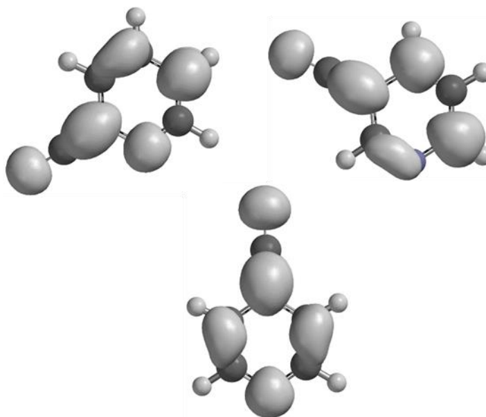
Figure 3. Mulliken spin density isosurfaces for the 2-CNPy •- , 3-CNPy •- , and 4-CNPy •- radical anions.
