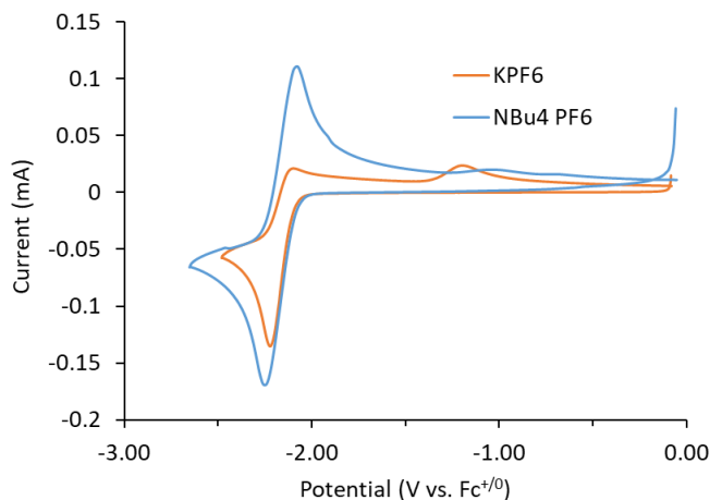
Figure 7. Cyclic voltammograms of 3-CN-6-PhPy at a glassy carbon electrode in CH 3 CN with 0.50 M [NBu 4 ][PF 6 ] and with 0.50 M KPF 6 at a scan rate of 100 mV/s.
