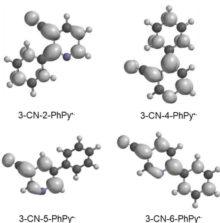
Figure 5. Mulliken spin density isosurfaces for 3-CN-2-PhPy •- , 3-CN-4-PhPy •- , 3-CN-5-PhPy •- and 3-CN-6-PhPy •- radical anions.
