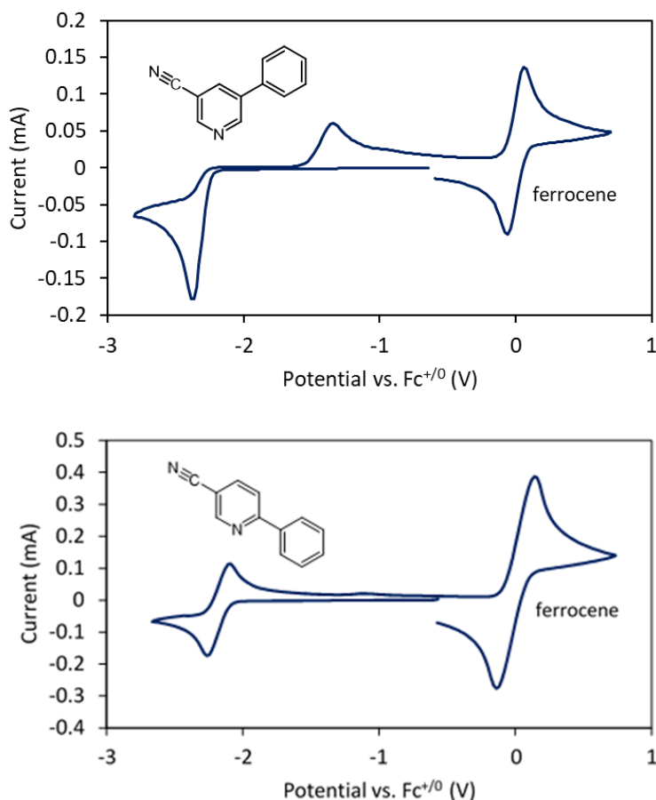
Figure 6. Cyclic voltammograms of 3-CN-5-PhPy (top) and 3-CN-6-PhPy (bottom) at a glassy carbon electrode in CH 3 CN with 0.50 M [NBu 4 ][PF 6 ] at a scan rate of 100 mV/s, both with a ferrocene internal standard. Dimerization of the radical anion of 3-CN-5-PhPy results in re-oxidation (of the dimer) at a positively shifted potential.
