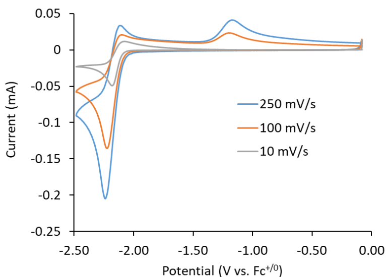
Figure 8. Cyclic voltammograms of 3-cyano-6-phenylpyridine at a glassy carbon electrode in \text{CH}_3\text{CN} with 0.50 M \text{KPF}_6 at scan rates of 10 , 100 , and 250 mV/s.
