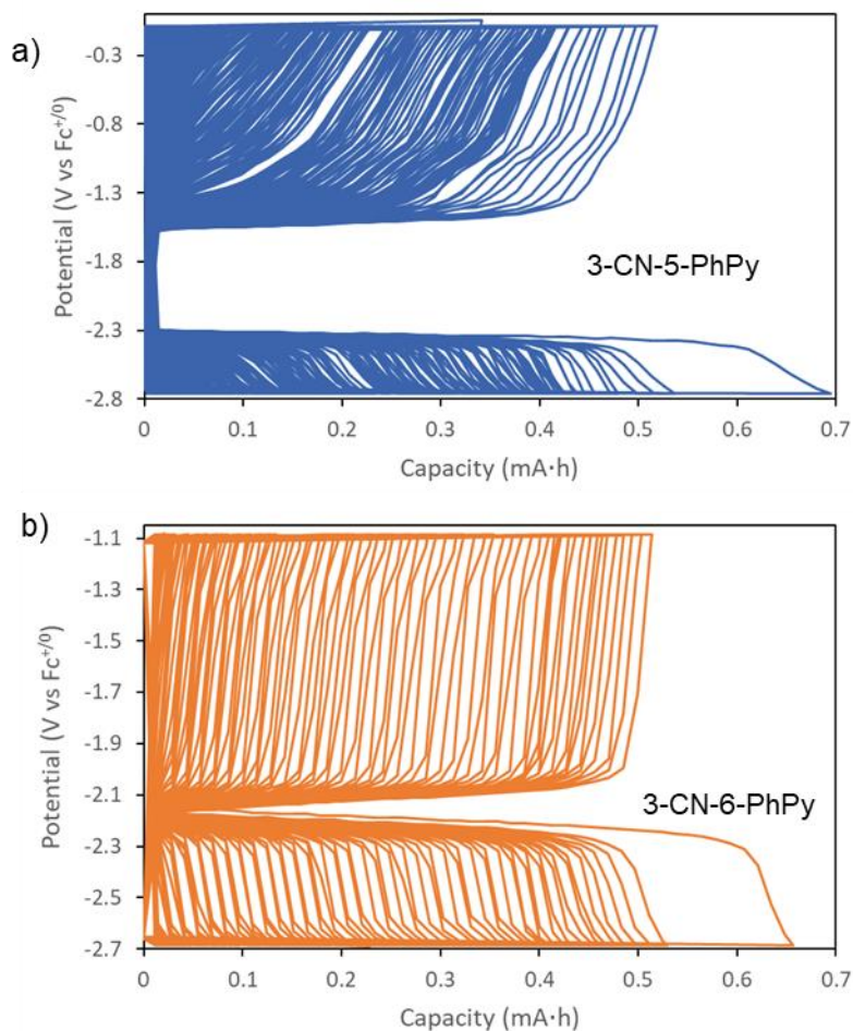
Figure 9. Charge-discharge curves (5.0 mL of a 5.0 mM solution of active material in 0.50 M [\text{NBu}_4][\text{PF}_6] in \text{CH}_3\text{CN} ; current = 5.00 mA) with for (a) 3-CN-5-PhPy and (b) 3-CN-6-PhPy. Theoretical capacity is 0.67 mAh.
