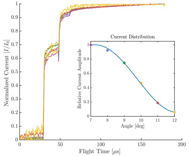
Fig. 5 Time of flight curves for 850 volts and 20 nA.
