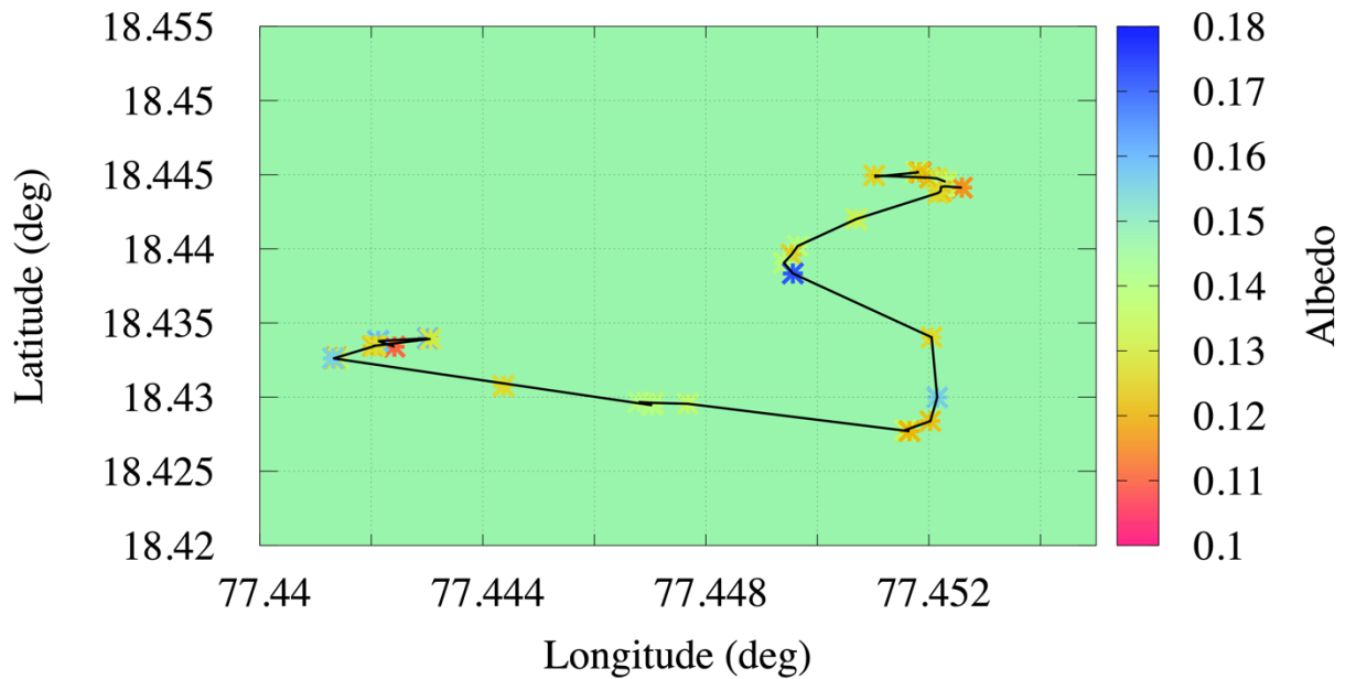
Figure 14. Color-coded albedo map showing MEDA-derived values at ~14:00 LMST (asterisks) across Perseverance’s traverse (black line), and a TES-retrieved value of 0.147 (greenish background color) for the shown area at around the same local time. Although MEDA-derived values ranged between 0.1 and 0.18 depending on the terrain, the averaged MEDA-derived value across Perseverance’s traverse is 0.14, in good agreement with TES.
