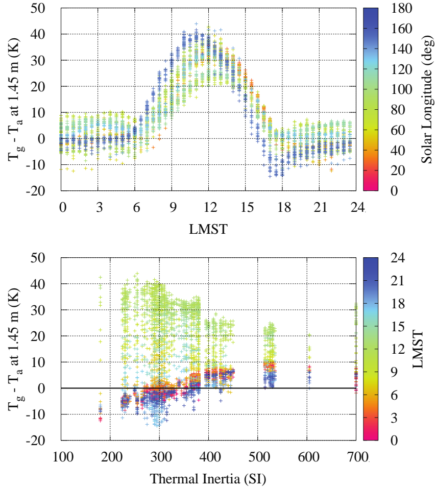
Figure 12. (Top) Diurnal evolution of the thermal gradient in the first 1.45 m as a function of LMST, with color code for Ls. This evolution governs the diurnal variation of the turbulent heat flux shown in Fig. 9e. (Bottom) Thermal gradient in the first 1.45 m as a function of thermal inertia, with color code for LMST. For TI > 390 SI units, the ground temperature generally stayed warmer than the air at 1.45 m throughout the night (horizontal black line), indicating a lack of local thermal inversion.
