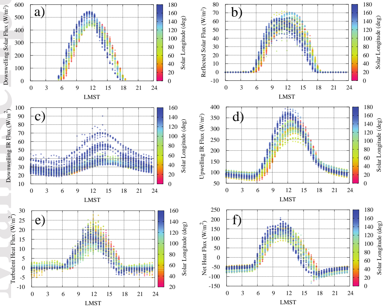
Figure 9. Diurnal evolution of the surface energy budget, Eq. (1), at Jezero crater for the first 350 sols of the Mars 2020 mission. Color-bar is used for Ls. Letters in each subpanel refer to the same term as in Fig. 8.
