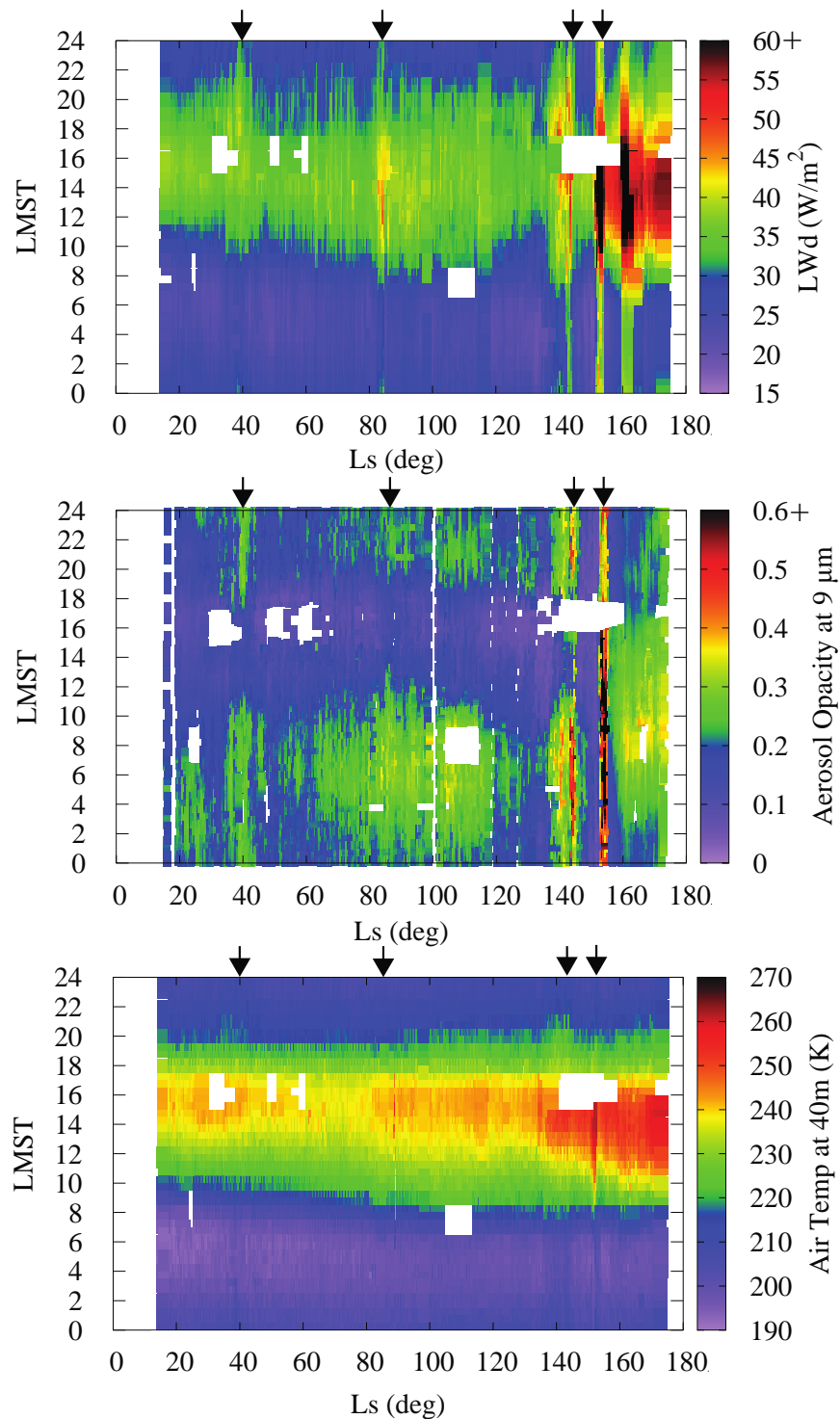
Figure 10. Color-coded downwelling LW flux ( top ), aerosol opacity at 9 μm ( middle ), and air temperature at ~40 m ( bottom ) as a function of Ls and LMST. The temporal gaps correspond to TIRS measurements taken either during in-flight calibrations or with the Sun within the FoV of IR1 and IR2. The black arrows mark the Ls at which the daily maximum, mean and minimum LW_d showed relative maxima (Fig. 8c).
