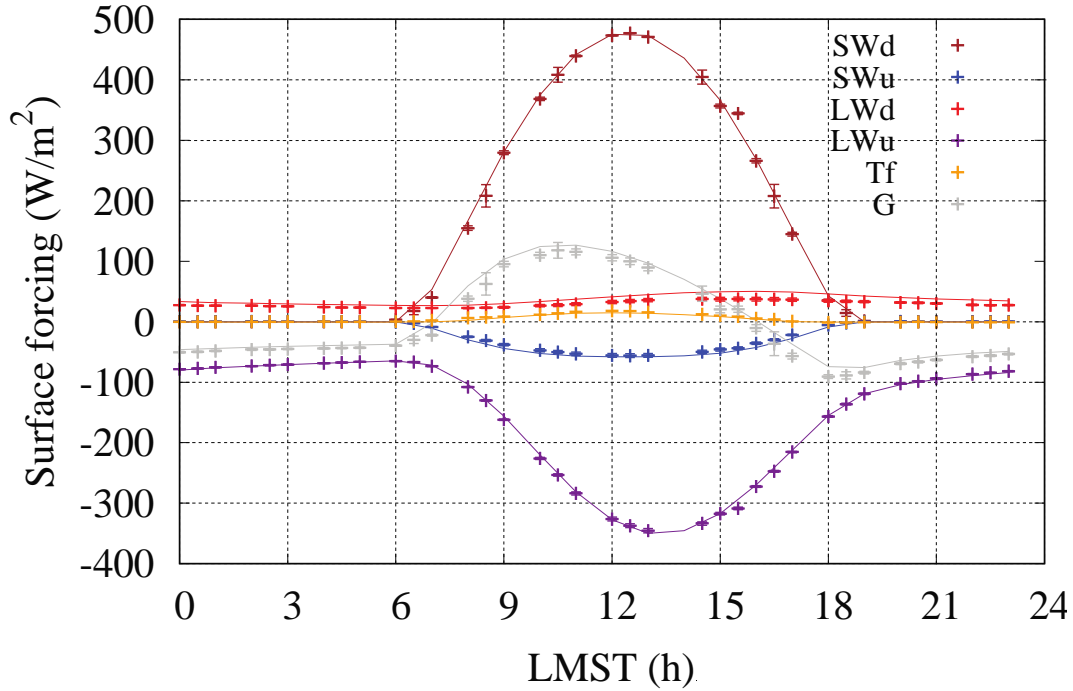
Figure 4. Surface energy budget on sol 30 ( L_s \sim 20^\circ ) as a function of LMST obtained from MEDA (symbols) and simulated with SCM (solid lines). Colors represent the terms of the SEB in Eq. (1). Except for the downwelling LW flux (red), which is systematically overestimated by the model, there is a very good agreement between observations and simulations. This behavior repeats on every other sol. SCM was run on sol 30 using the following values: visible aerosol opacity, \tau = 0.47 (obtained from Mastcam-Z, Fig. 3a), albedo at noon, \alpha = 0.12 (obtained from MEDA), and thermal inertia, TI = 225 \text{ J m}^{-2} \text{ K}^{-1} \text{ s}^{-1/2} , which provides the best SCM fit to measured ground temperatures).
