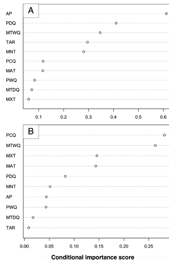
Fig. 3. Conditional forest analysis variable importance for (A) nitrogen isotope values and (B) carbon isotope values of the Virginia opossum ( Didelphis virginiana ). WorldClim variables include annual precipitation (AP), precipitation in the driest quarter (PDQ), mean temperature in the wettest quarter (MTWQ), temperature annual range (TAR), minimum temperature in the coldest month (MNT), precipitation in the coldest quarter (PCQ), mean annual temperature (MAT), precipitation in the wettest quarter (PWQ), mean temperature in the driest quarter (MTDQ), and maximum temperature in the warmest month (MXT).
