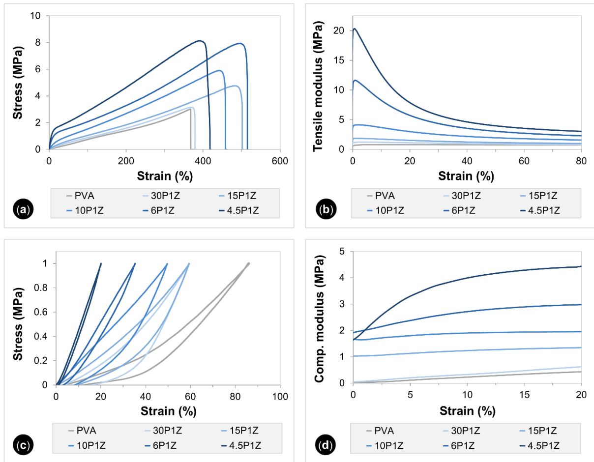
Figure 6. Mechanical characterization of PVA and nanofiber-reinforced hydrogels with different PVA:PBO nanofiber mass ratios. Typical tensile stress-strain curves (a) and corresponding values of tensile moduli up to 80% of strain (b). Typical compressive stress-strain curves (c) and corresponding values of compression moduli up to 20% of strain (d).
