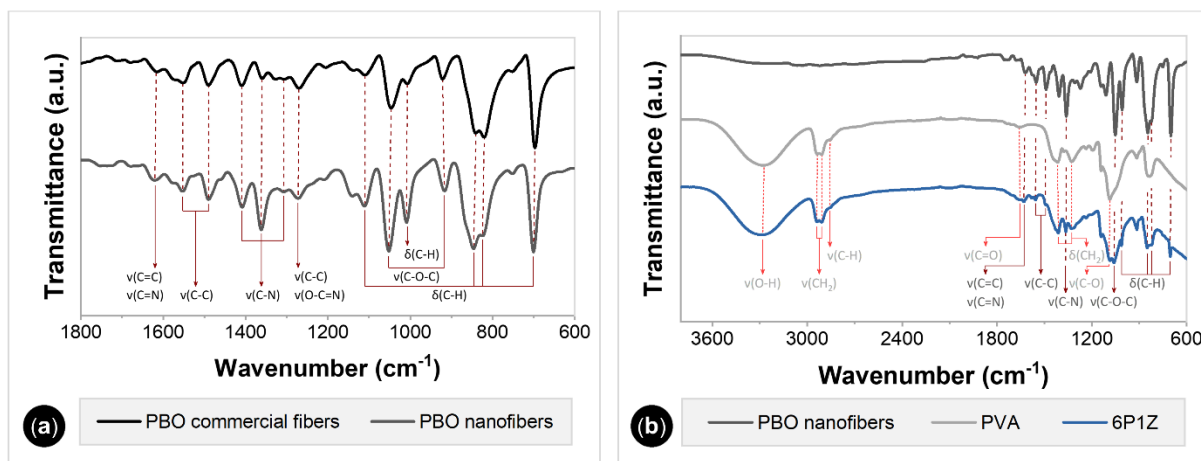
Figure 3. ATR-FTIR spectra of PBO commercial fibers and nanofibers (a). ATR-FTIR spectra of PBO nanofibers, PVA, and 6P1Z (b). Abbreviations: v - stretching; and \delta - bending.
