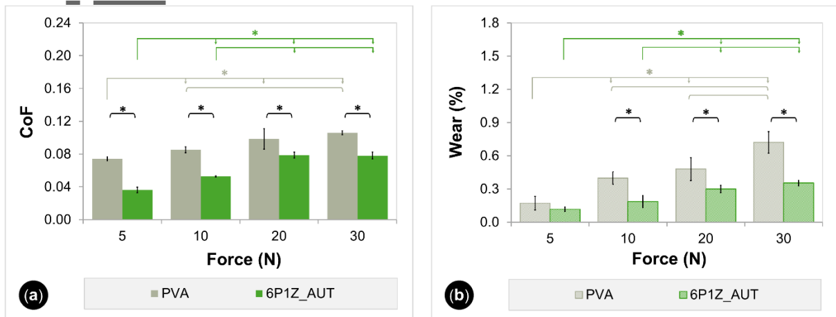
Figure 8. Dynamic friction coefficients (a) and wear mass percentages (b) of PVA and 6P1Z_AUT samples obtained in the ball-on-plate friction tests under lubricated conditions. The error bars correspond to \pm SD. Friction coefficient data were tested by Welch's ANOVA/Dunnett's T3 (PVA under 5, 10, 20 or 30 N), ANOVA/Tukey's HSD (6P1Z_AUT under 5, 10, 20 or 30 N), and independent samples t-test (PVA vs. 6P1Z_AUT under each of the applied forces). Data from the wear measurements were analyzed by ANOVA/Tukey's HSD (each type of sample under 5, 10, 20, or 30 N) and independent samples t-test (PVA vs. 6P1Z_AUT under each of the applied forces). Statistical differences ( p < 0.05 ) between groups are indicated with an asterisk (*).
