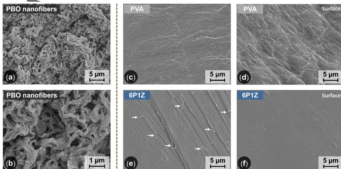
Figure 2. Cross-sectional SEM images of PBO nanofiber films (a, b), PVA (c), and 6P1Z (e). SEM images of the surface of PVA (d) and 6P1Z (f). The white arrows indicate the location of some of the nanofibers incorporated within the 6P1Z composite.
